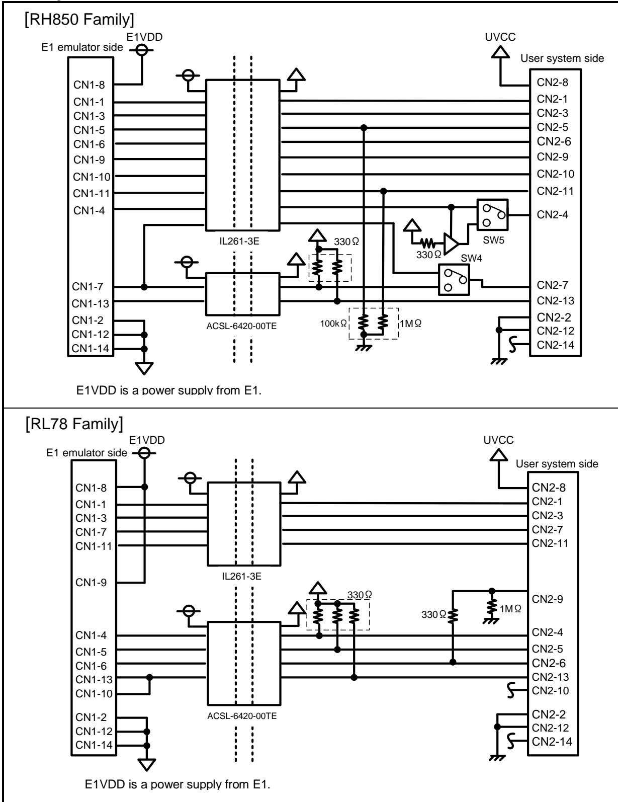
Figure 4.2 Connection Diagrams
