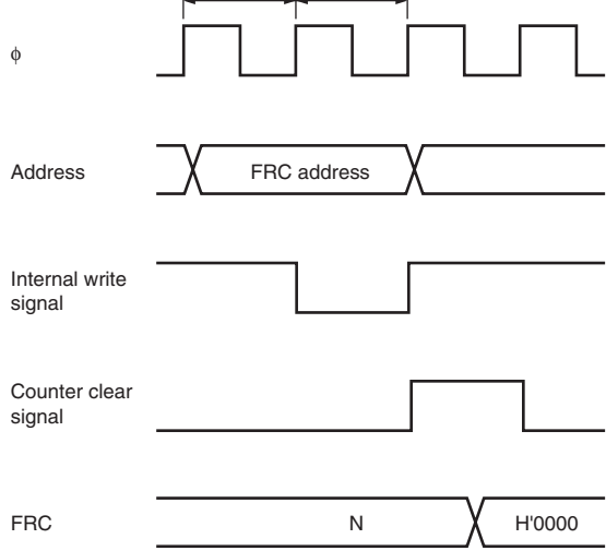
Figure 10.8 Conflict between FRC Write and Clear
