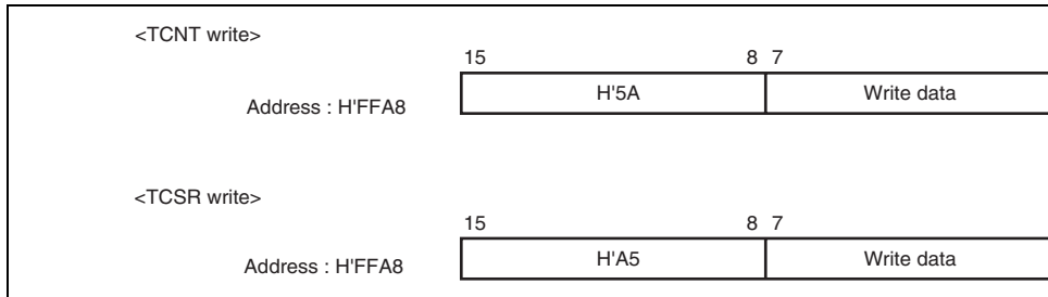
Figure 12.6 Writing to TCNT and TCSR (WDT_0)
