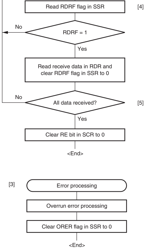
Figure 13.19 Sample Serial Reception Flowchart
