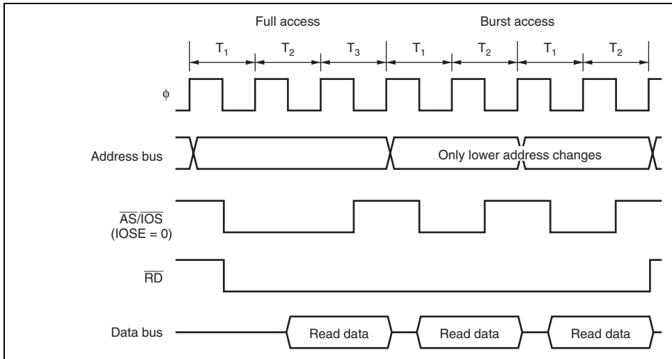
Figure 6.30 Access Timing Example in Burst ROM Space (AST = BRSTS1 = 1)
