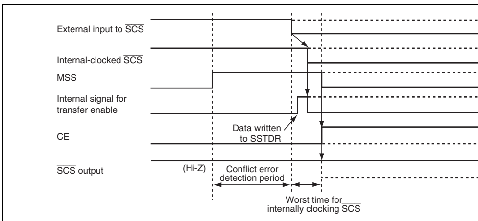
Figure 17.10 Conflict Error Detection Timing (Before Transfer)
