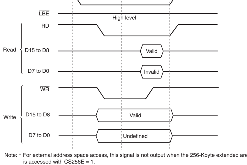
Figure 6.13 Glueless Extension Even Byte Access (ADMXE = 0)
