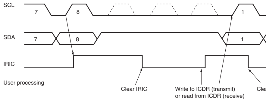
Figure 18.27 IRIC Setting Timing and SCL Control (3)
