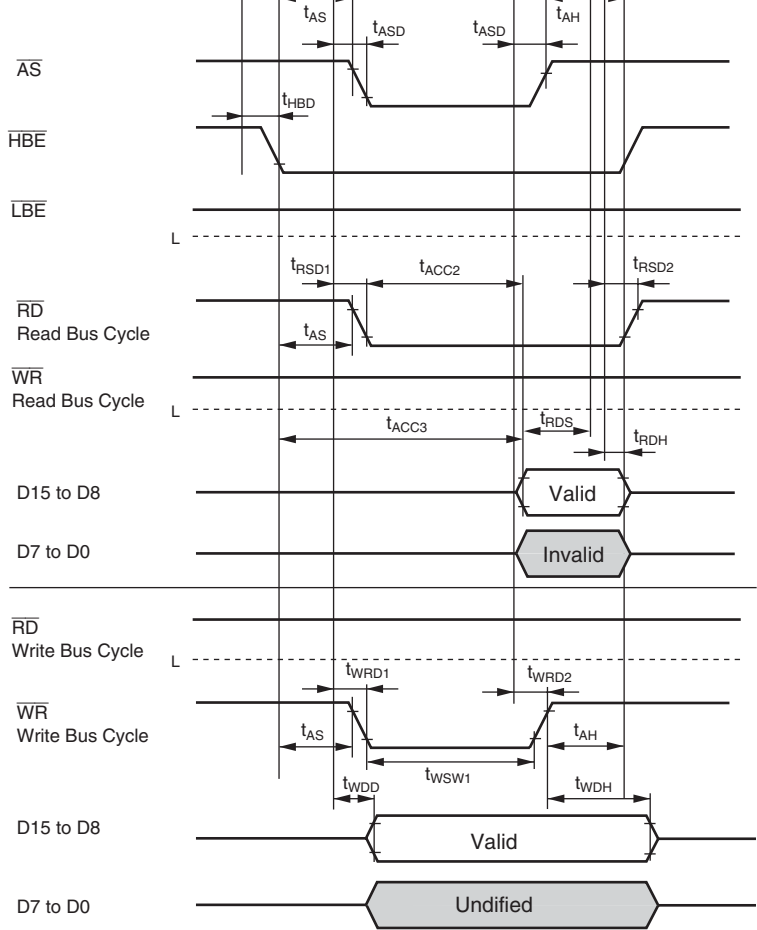
Figure 31.15 Even Byte Access ( ADMXE = 0 )
