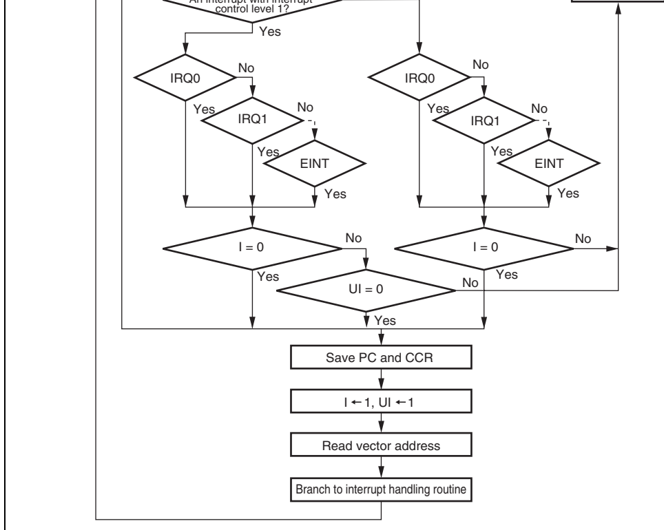
Figure 5.6 Flowchart of Procedure Up to Interrupt Acceptance in Interrupt Control Mode 1
