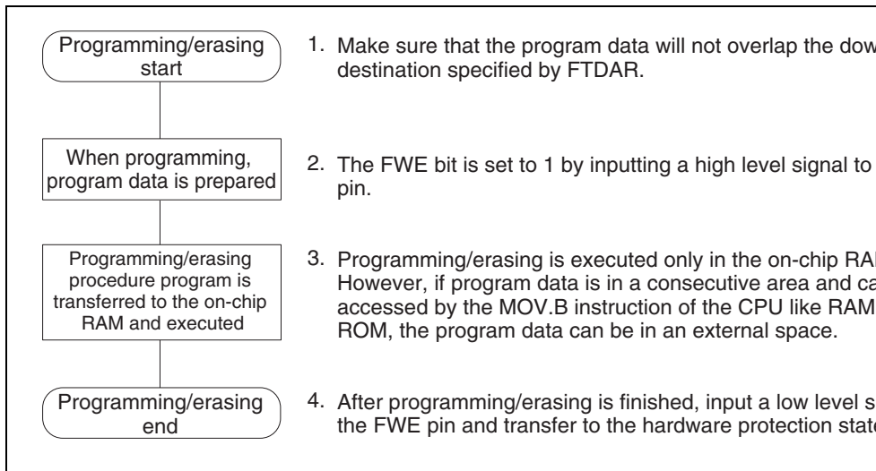
Figure 25.11 Programming/Erasing Overview Flow
