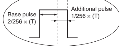
Figure 9.6 Output Waveform when DADR = H'0207 (OS = 1)
