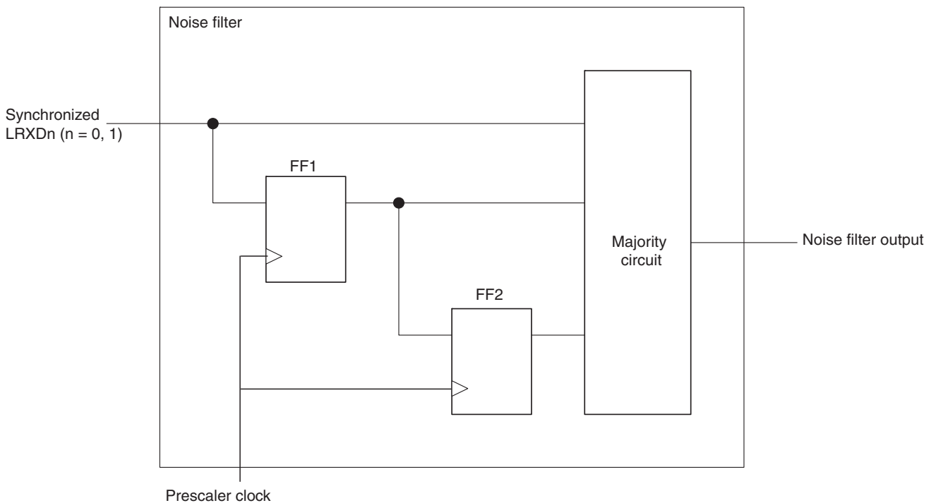
Figure 17-45. Example of Noise Filter Circuit
