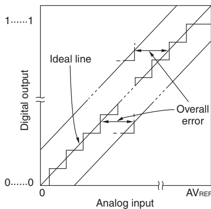
Figure 12-42. Overall Error
