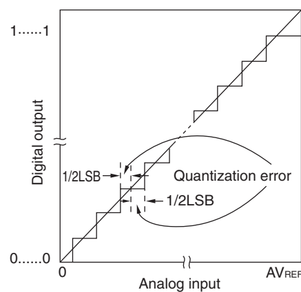
Figure 12-43. Quantization Error
