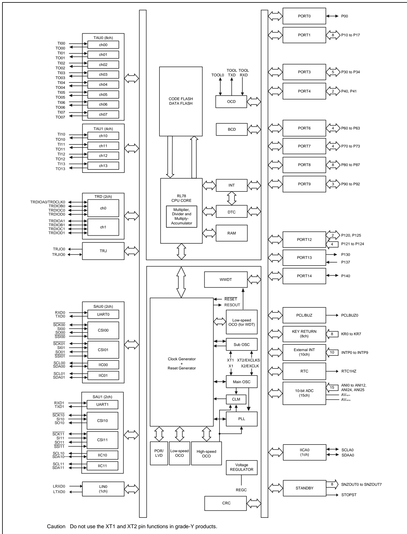
Figure 1-17. Block Diagram
