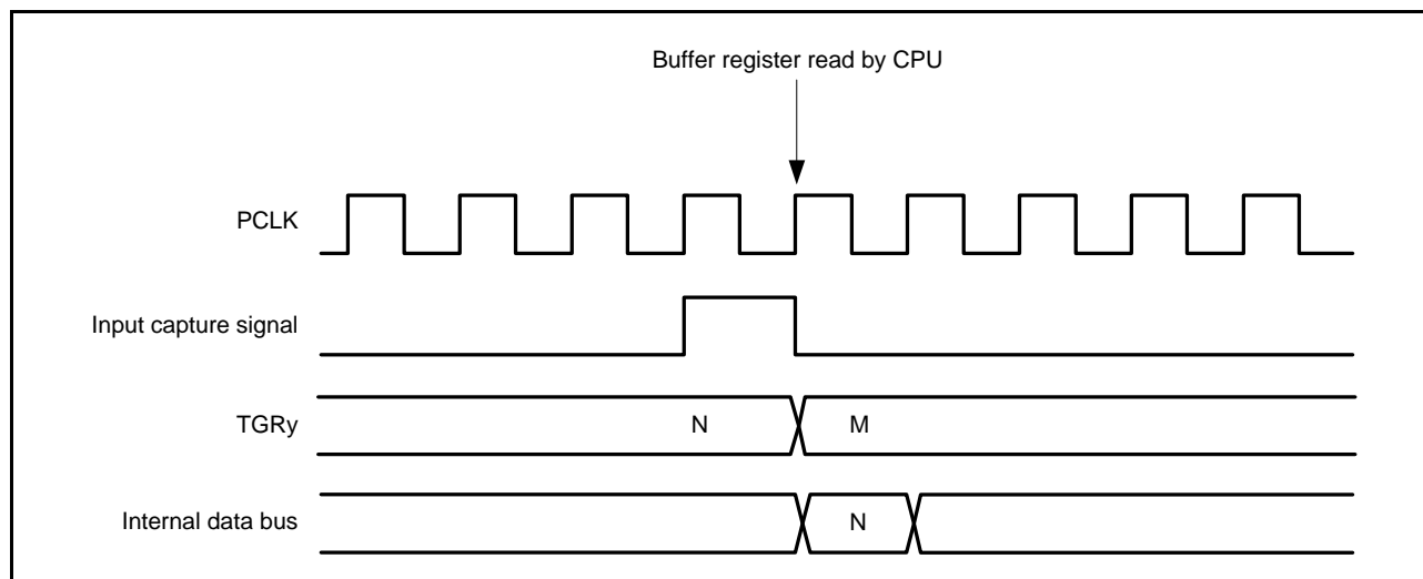
Figure 24.49 Conflict between TPUM.TGRy Read and Input Capture
