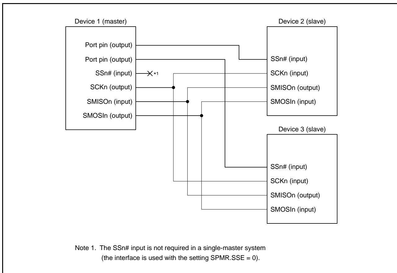
Figure 32.51 Example of Connections via a Simple SPI Mode (In Single Master Mode, SPMR.SSE Bit = 0)
