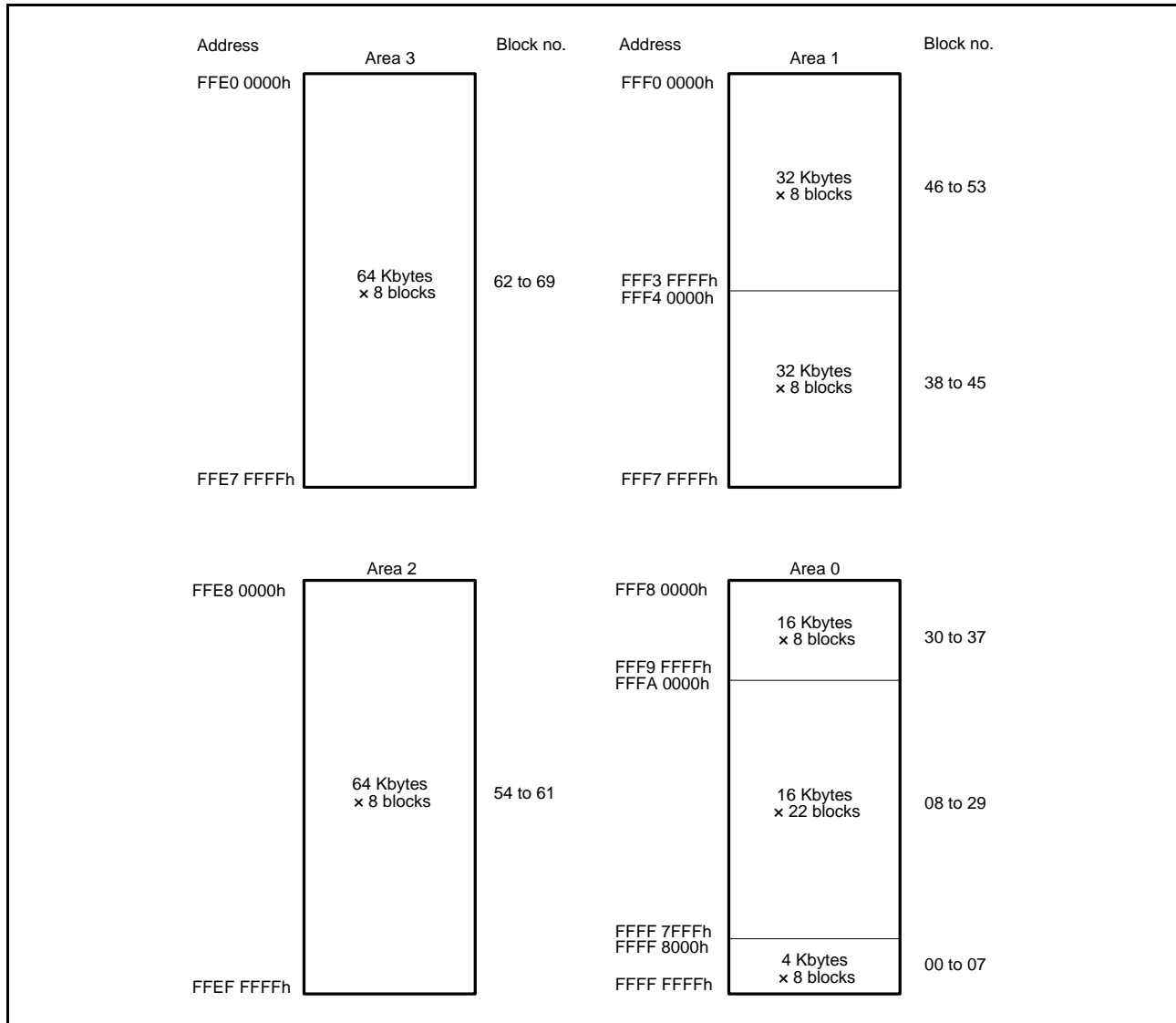
Figure 43.3 Block Configuration of the User Area
