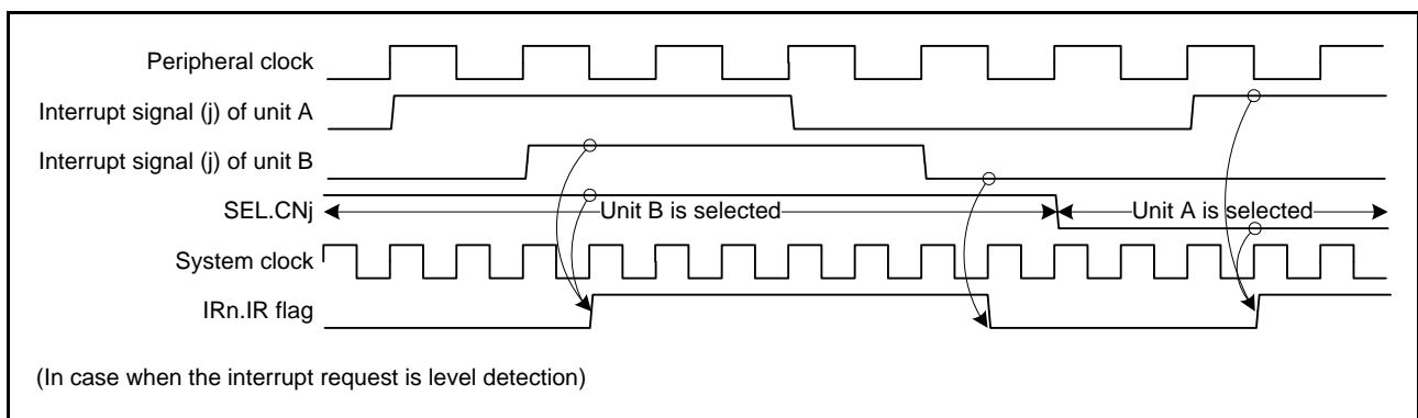
Figure 15.17 Unit Selection Example
