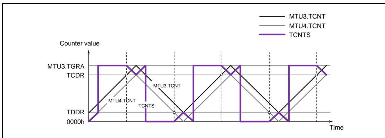
Figure 22.39 Counter Operation in Complementary PWM Mode
