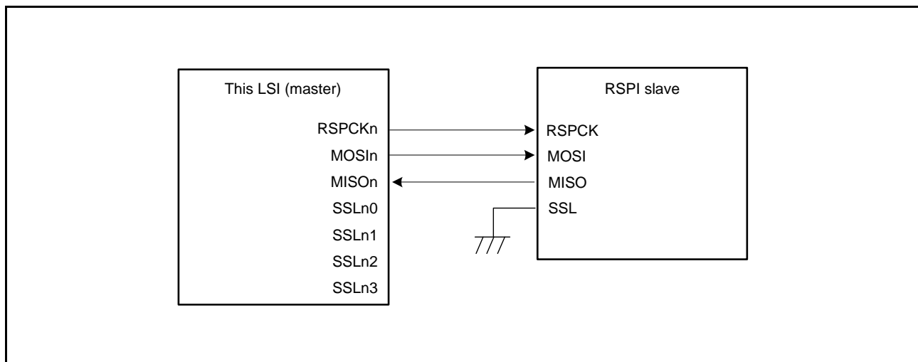
Figure 35.5 Single-Master/Single-Slave Configuration Example (This LSI = Master)
