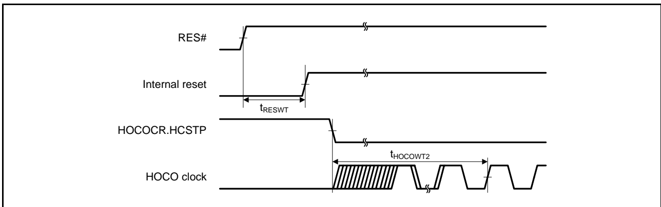
Figure 45.8 HOCO Clock Oscillation Start Timing (Oscillation is Started by Setting the HOCOEN Bit)
