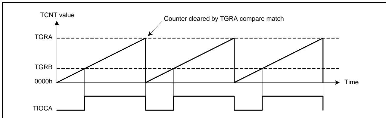
Figure 24.22 Example of PWM Mode Operation (1)
