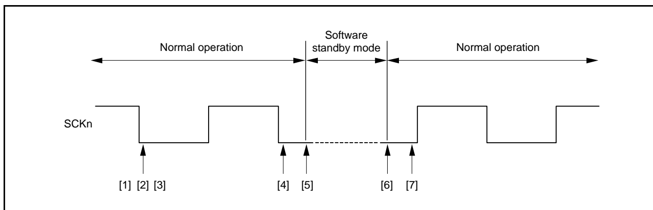
Figure 32.39 Clock Stop and Restart Procedure
