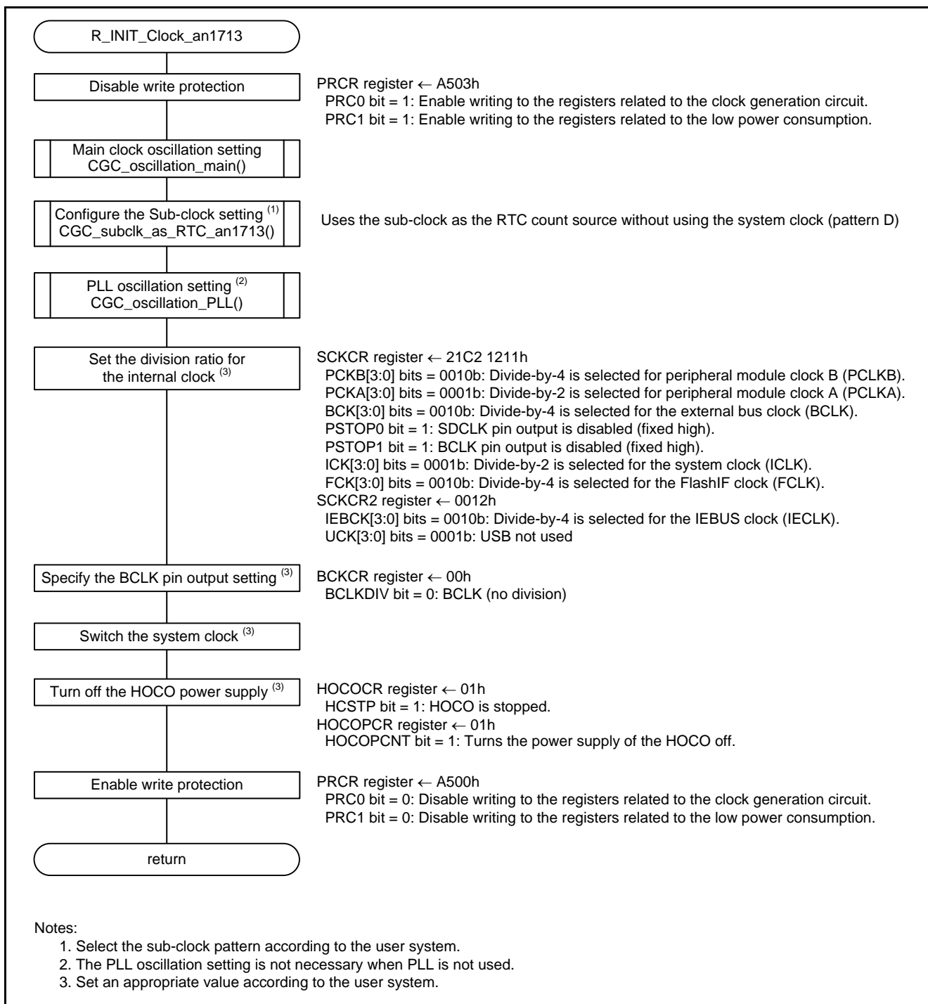
Figure 5.13 Clock Initialization
