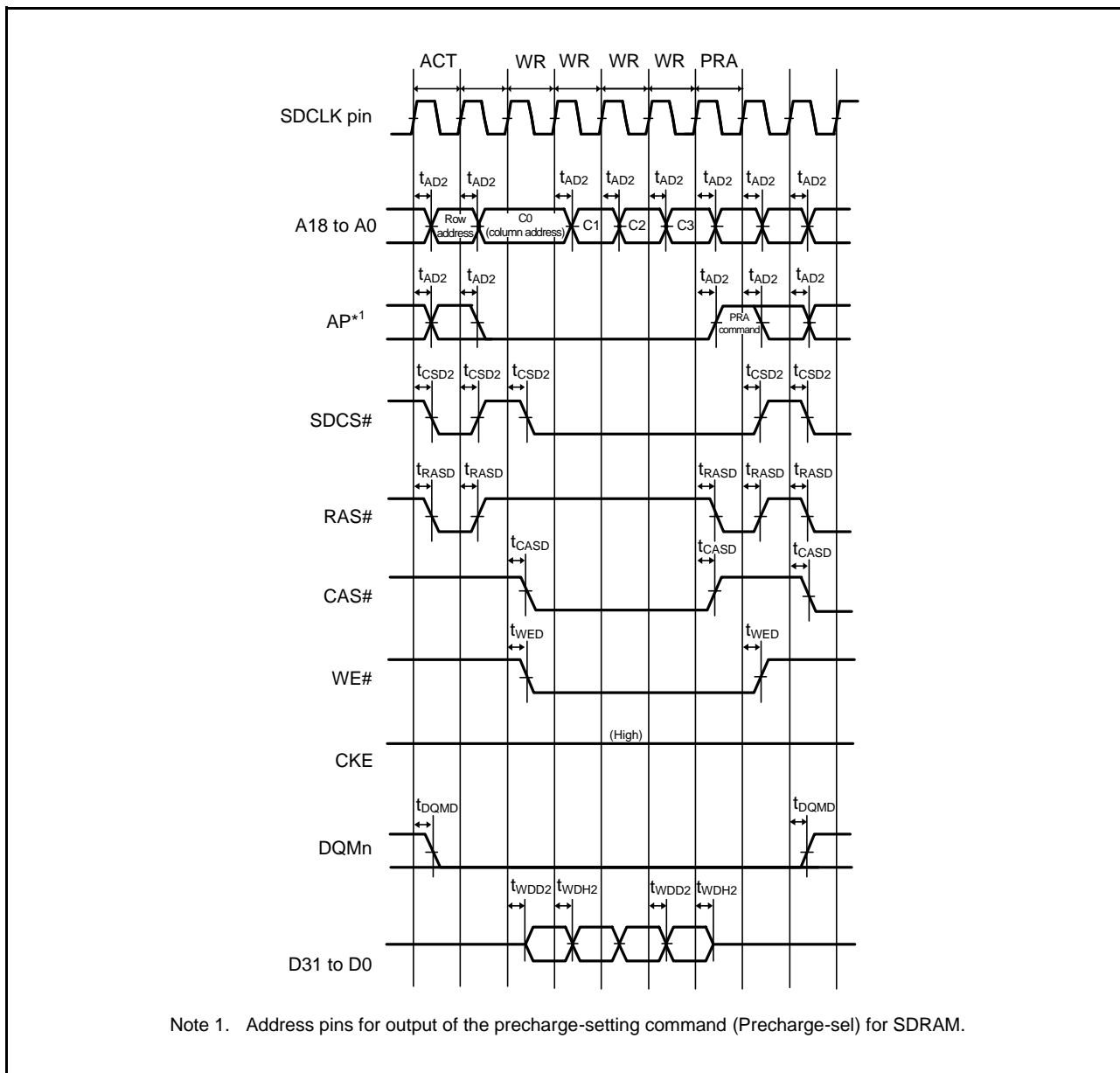
Figure 2.28 SDRAM Space Multiple Write Bus Timing
