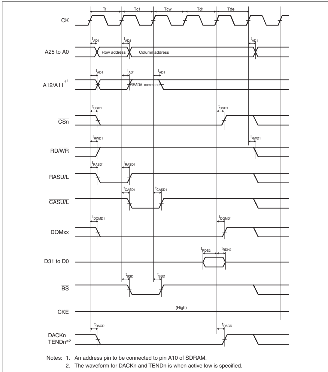
Figure 31.18 Synchronous DRAM Single Read Bus Cycle (Auto Precharge, CAS Latency 2, WTRCD = 0 Cycle, WTRP = 0 Cycle)
