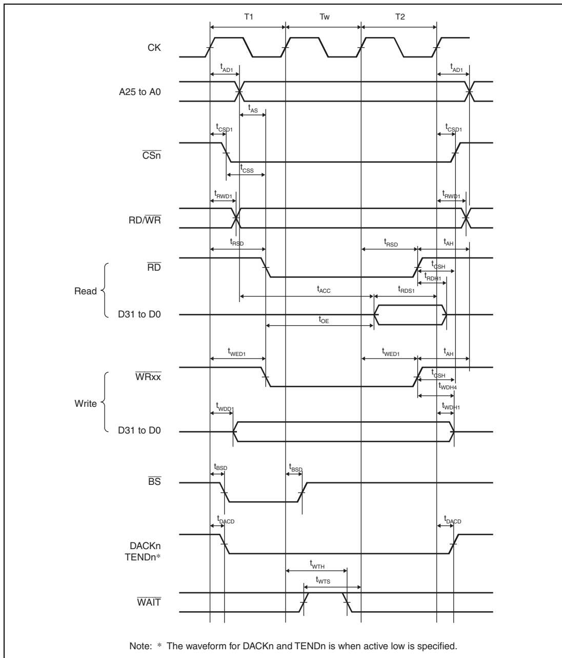
Figure 31.11 Basic Bus Timing for Normal Space (One Software Wait Cycle)
