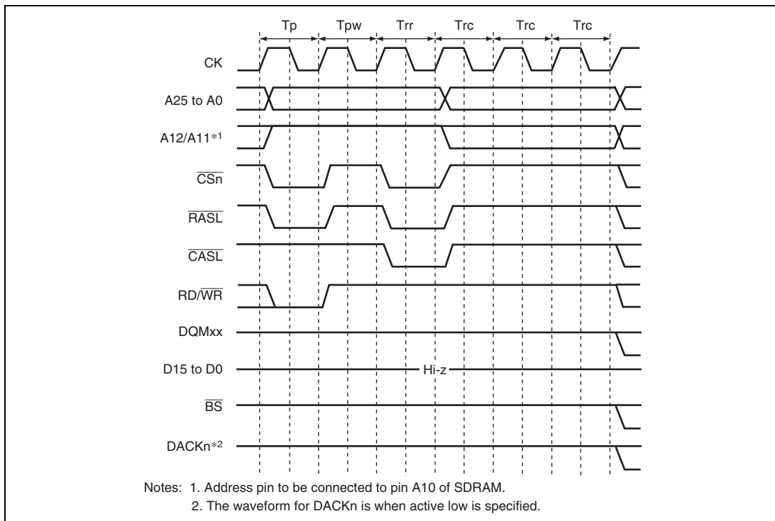
Figure 9.28 Auto-Refresh Timing
