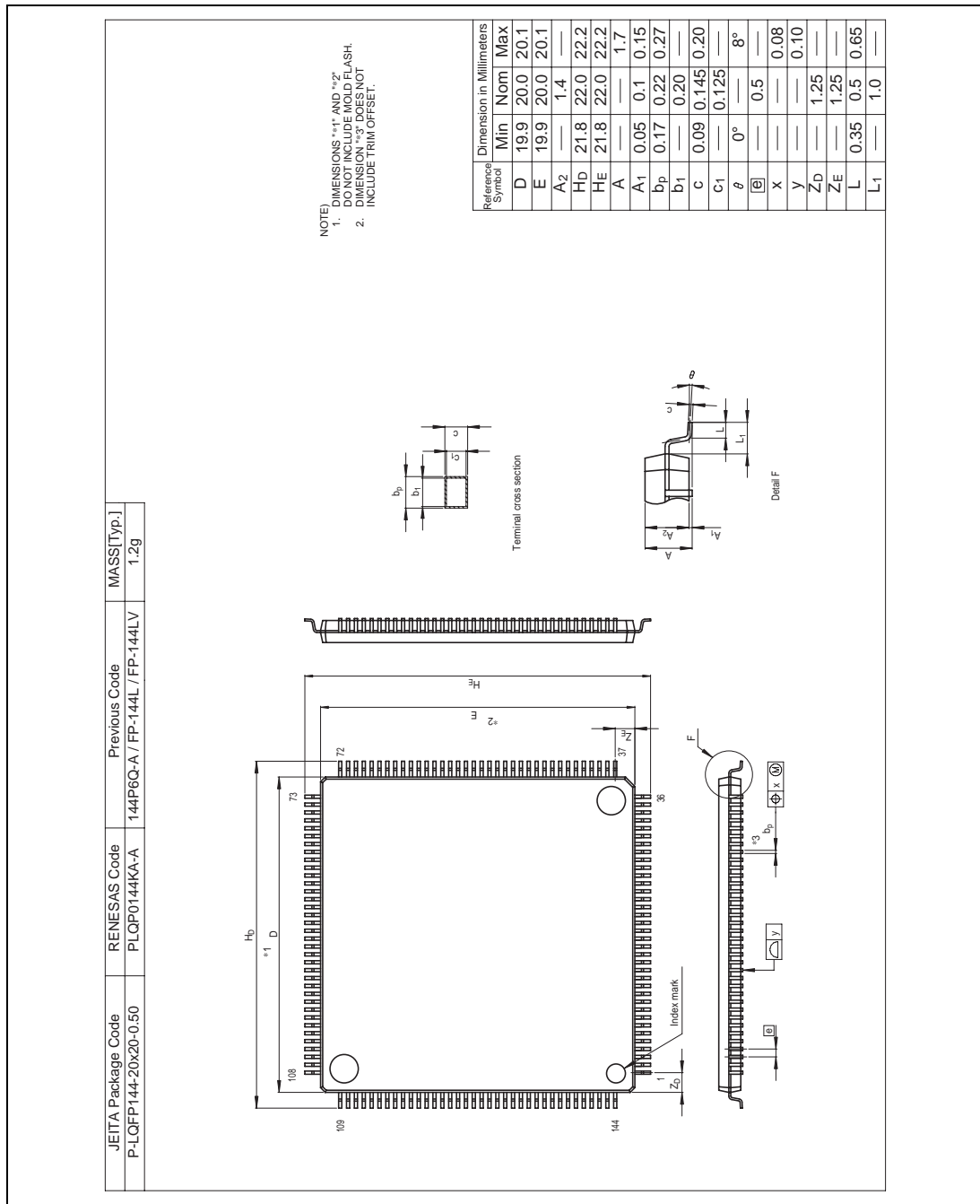
Figure C.2 FP-144LV
