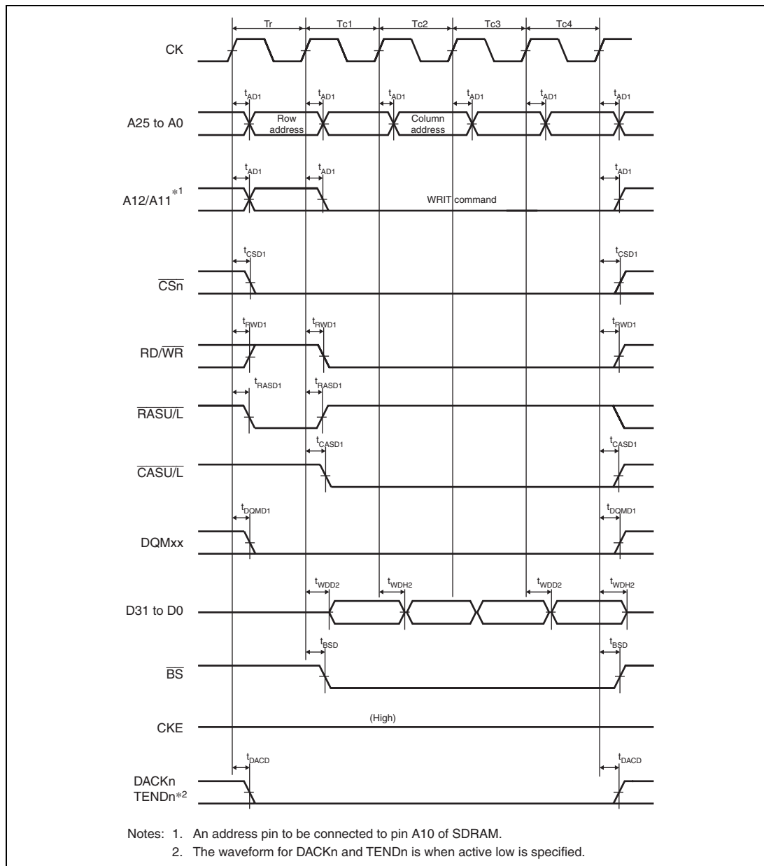
Figure 31.29 Synchronous DRAM Burst Write Bus Cycle (Four Write Cycles) (Bank Active Mode: ACT + WRITE Commands, WTRCD = 0 Cycle, TRWL = 0 Cycle)
