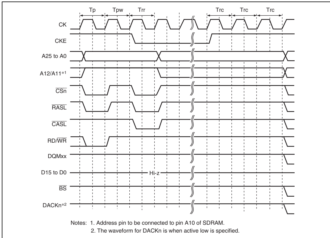
Figure 9.29 Self-Refresh Timing
