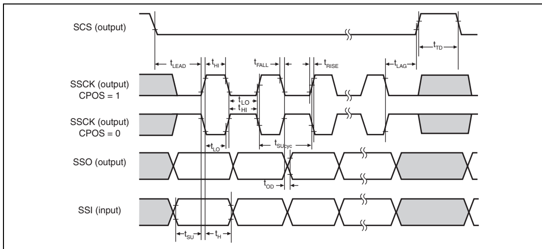
Figure 31.49 SSU Timing (Master, CPHS = 1)
