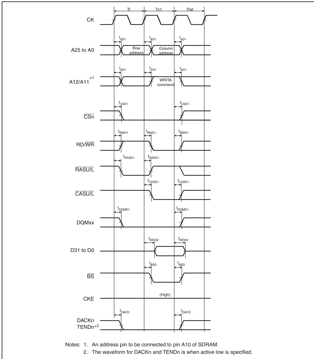
Figure 31.22 Synchronous DRAM Single Write Bus Cycle (Auto Precharge, TRWL = 1 Cycle)
