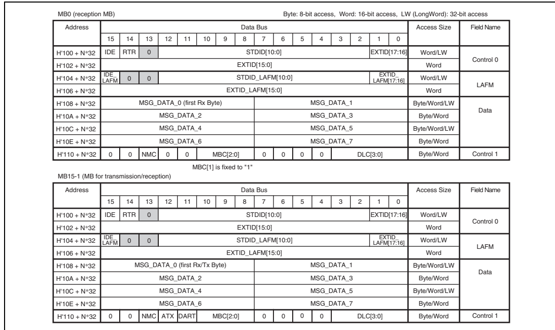
Figure 22.3 Mailbox-N Structure
