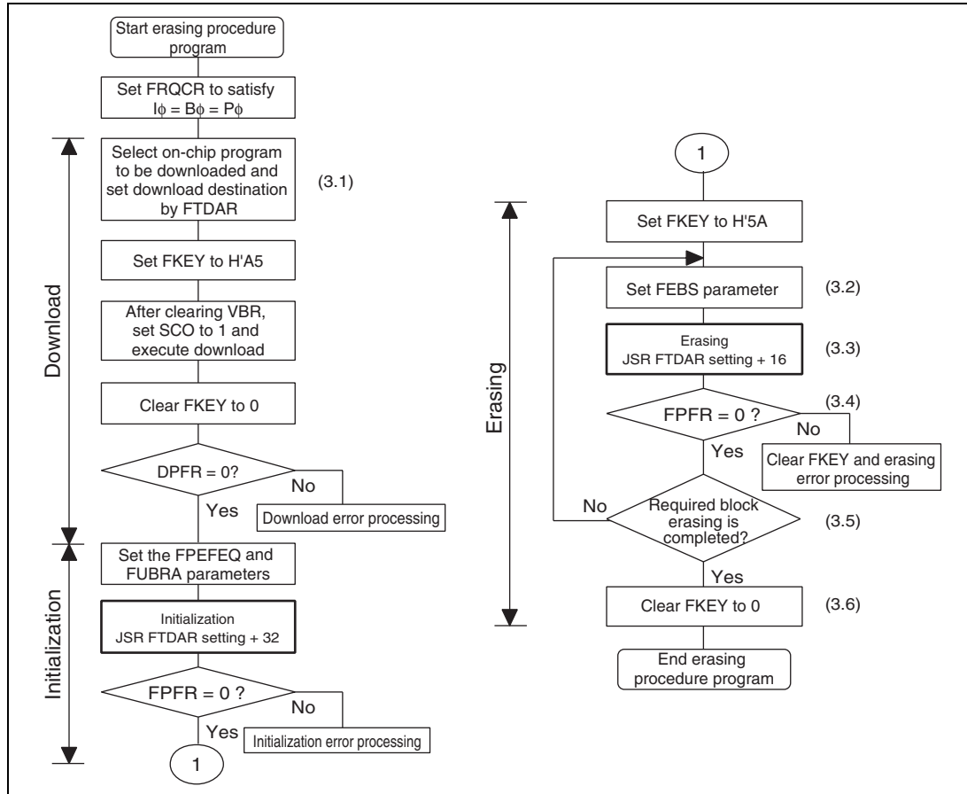
Figure 26.14 Erasing Procedure
