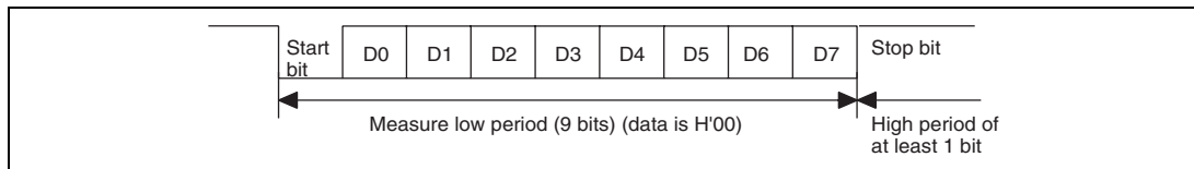
Figure 26.7 Automatic Adjustment Operation of SCI Bit Rate
