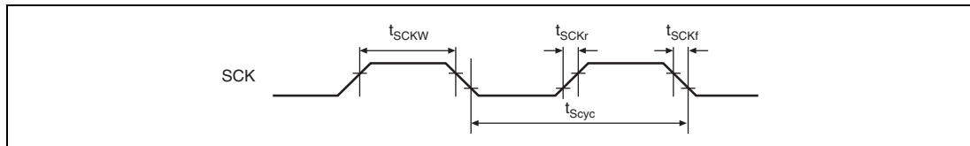
Figure 31.47 SCK Input Clock Timing
