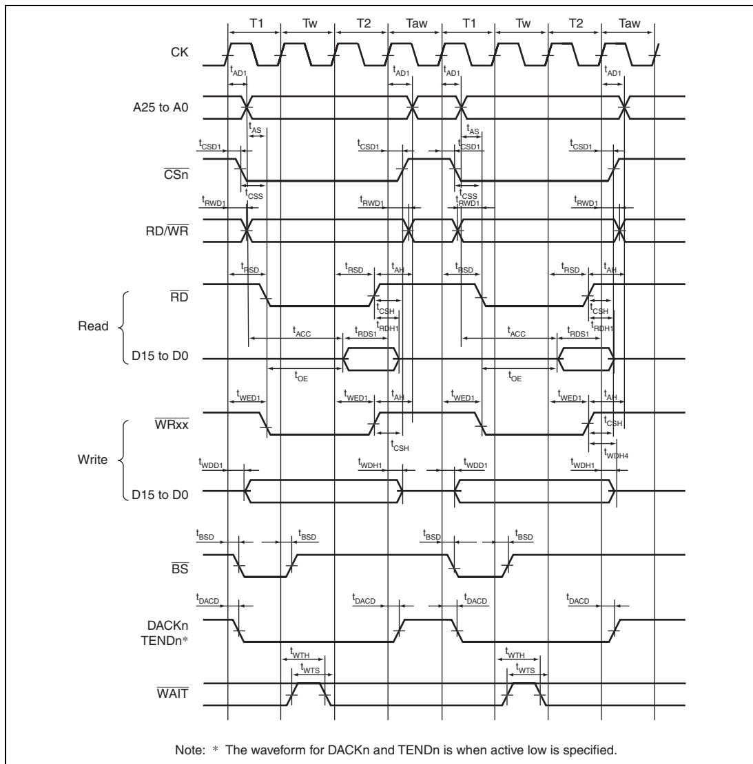
Figure 31.13 Basic Bus Timing for Normal Space (One Software Wait Cycle, External Wait Cycle Valid (WM Bit = 0), No Idle Cycle)
