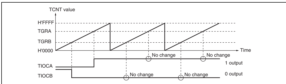
Figure 11.8 Example of 0 Output/1 Output Operation
