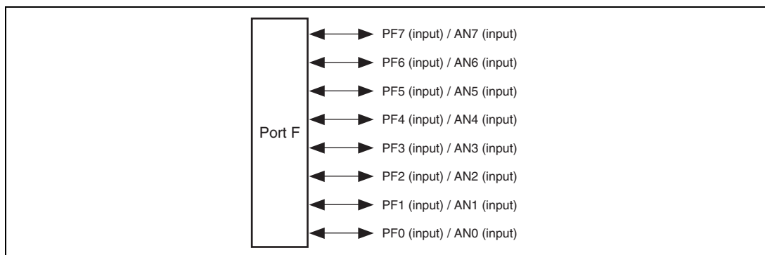
Figure 24.15 Port F (SH7243 and SH7285)
