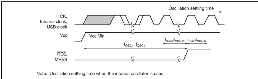
Figure 31.3 Power-On Oscillation Settling Time
