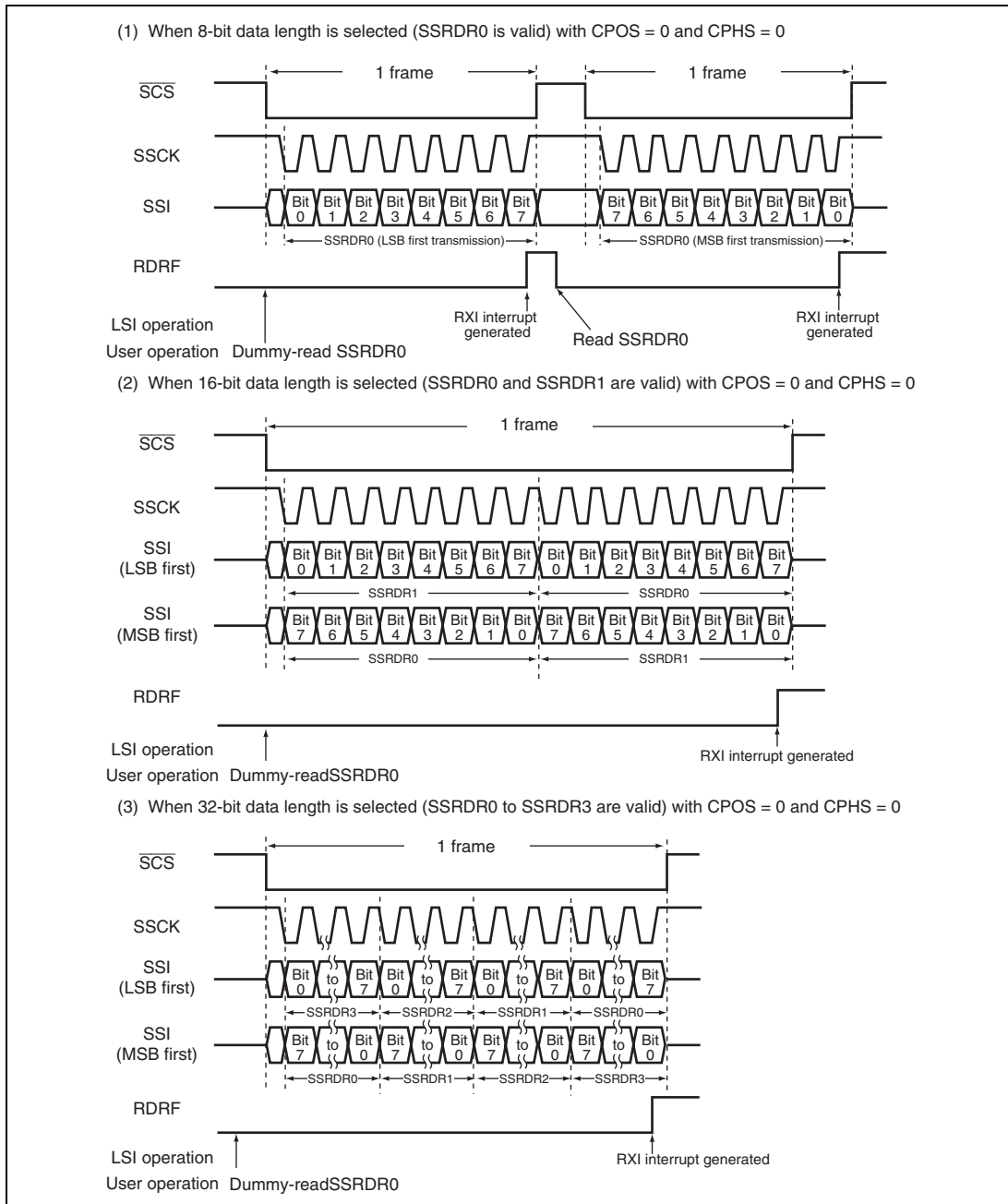
Figure 18.7 Example of Reception Operation (SSU Mode)
