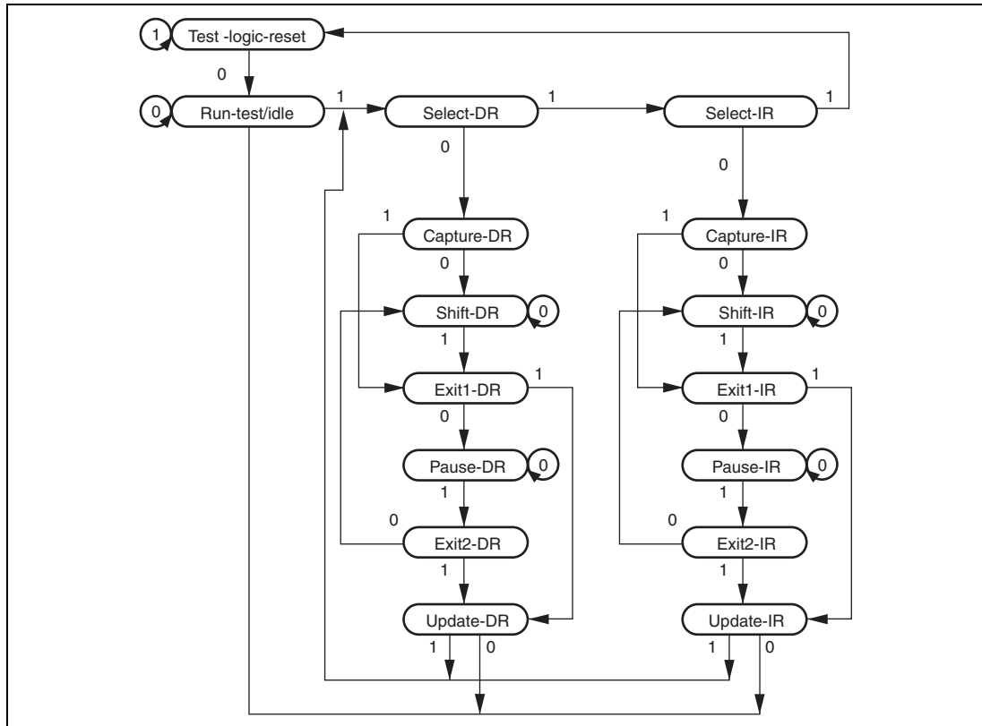
Figure 29.2 TAP Controller State Transitions
