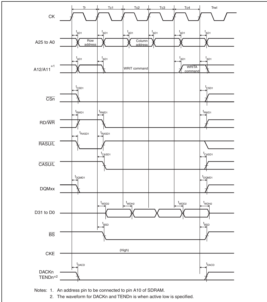
Figure 31.24 Synchronous DRAM Burst Write Bus Cycle (Four Write Cycles) (Auto Precharge, WTRCD = 0 Cycle, TRWL = 1 Cycle)
