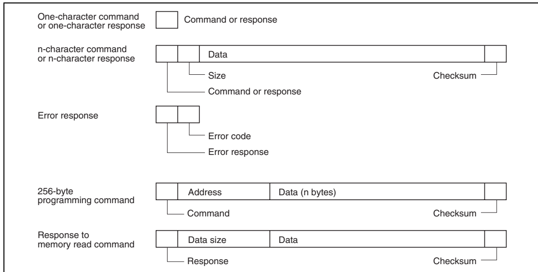
Figure 26.23 Formats in the Communications Protocol
