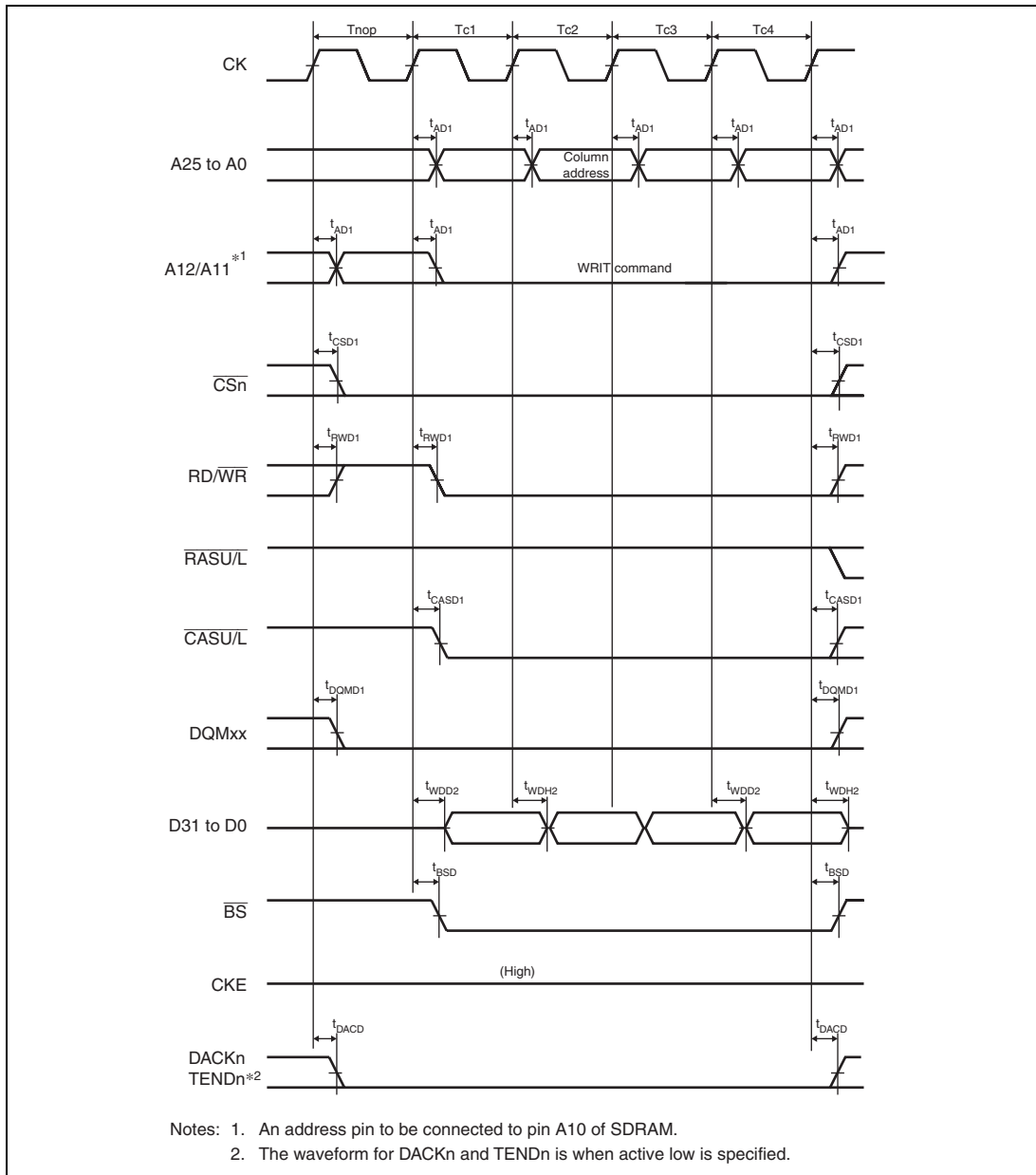
Figure 31.30 Synchronous DRAM Burst Write Bus Cycle (Four Write Cycles) (Bank Active Mode: WRITE Command, Same Row Address, WTRCD = 0 Cycle, TRWL = 0 Cycle)
