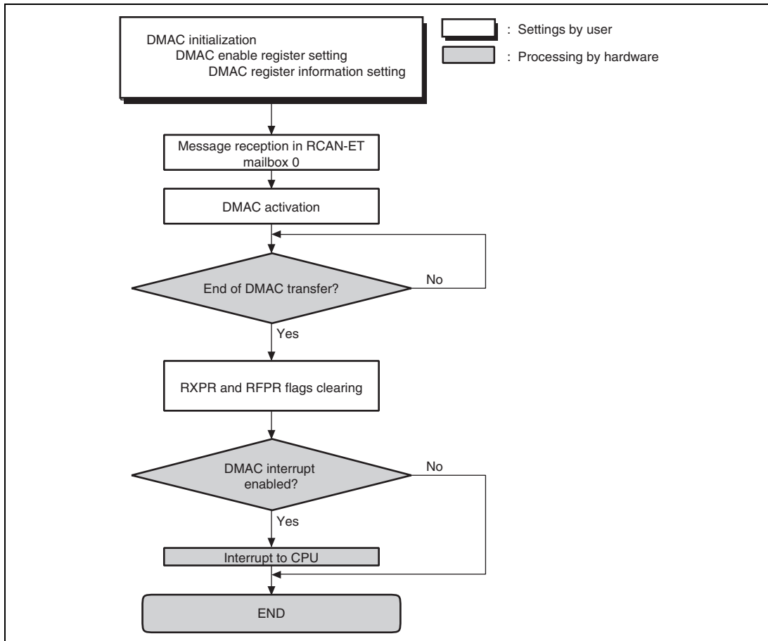
22.15 DMAC Transfer Flowchart
