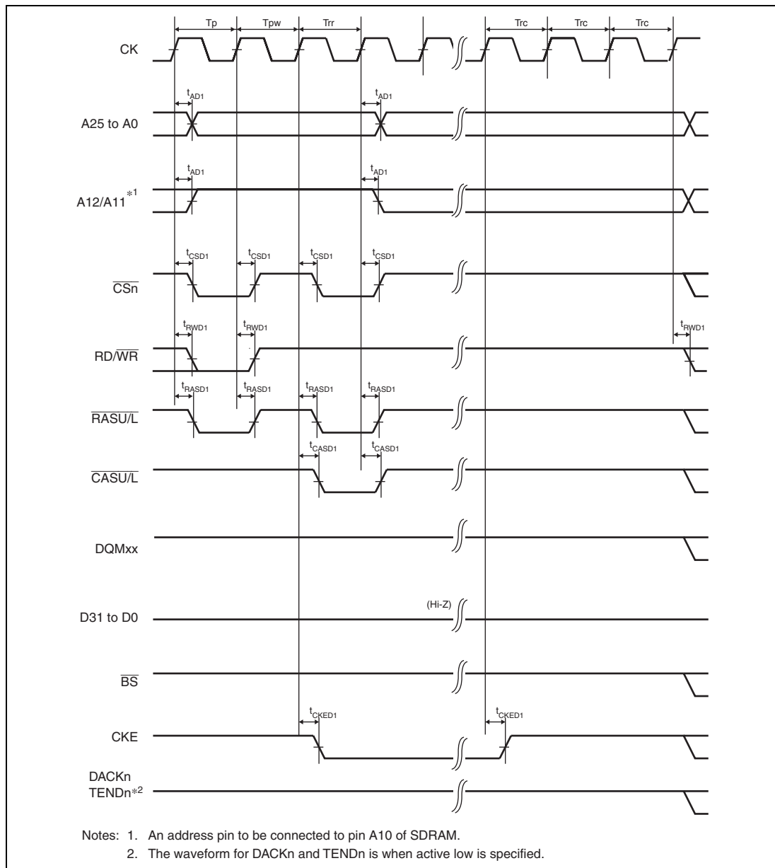
Figure 31.33 Synchronous DRAM Self-Refreshing Timing (WTRP = 1 Cycle)
