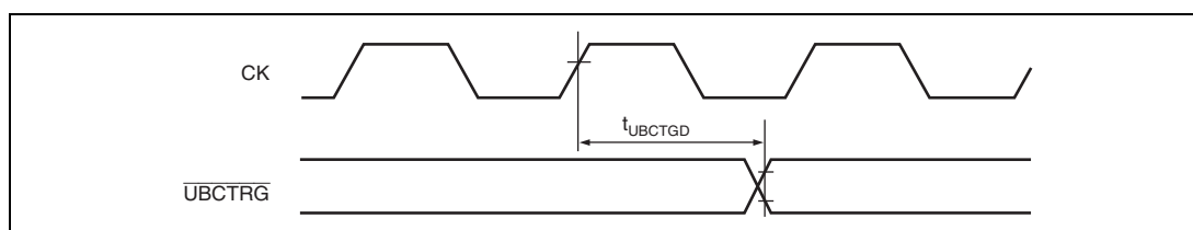
Figure 31.37 UBC Trigger Timing
