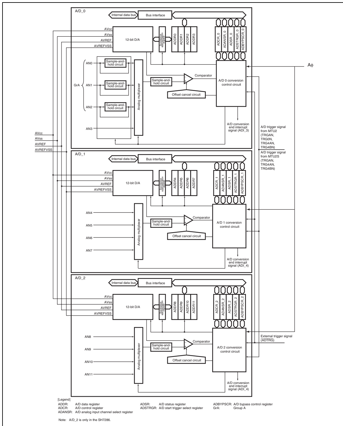
Figure 20.1 Block Diagram of A/D Converter
