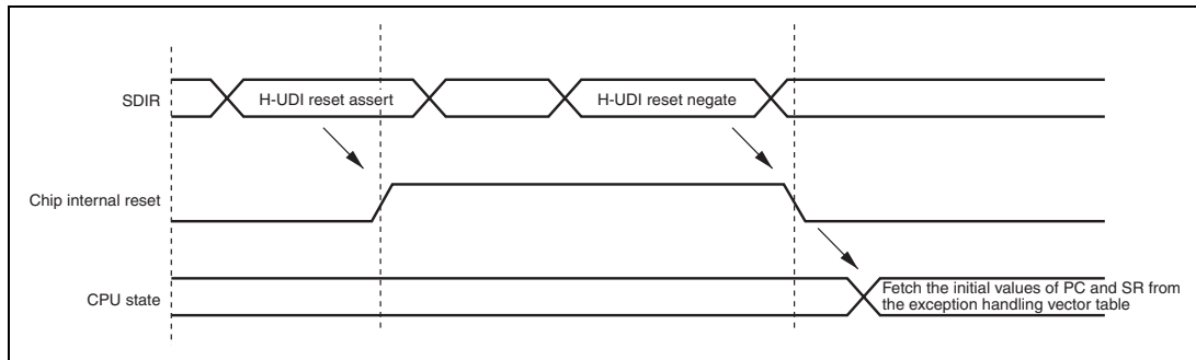
Figure 29.4 H-UDI Reset
