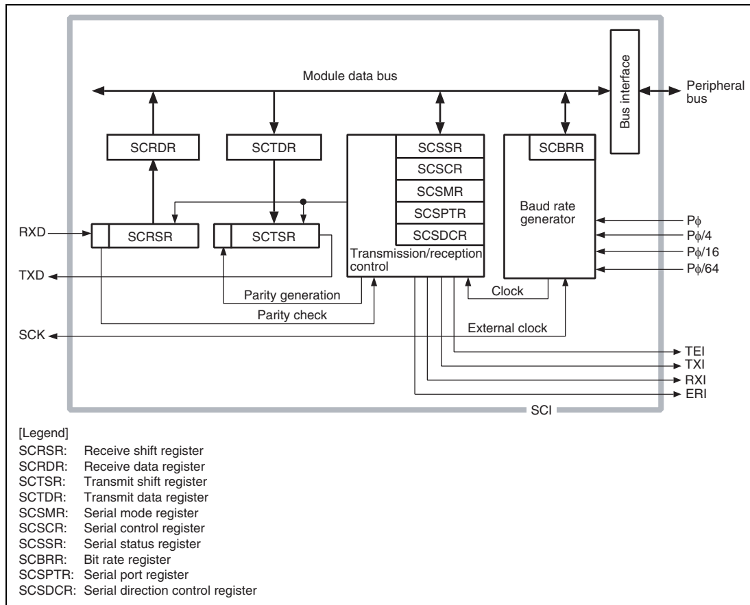
Figure 16.1 Block Diagram of SCI
