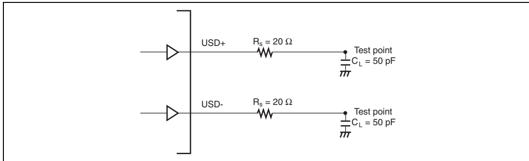
Figure 31.61 Test Load Circuit
