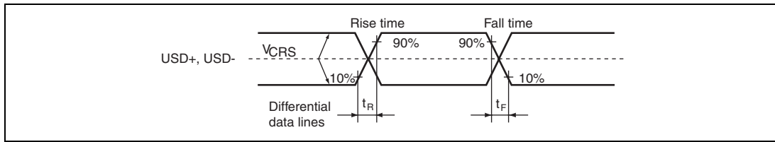
Figure 31.60 Data Signal Timing
