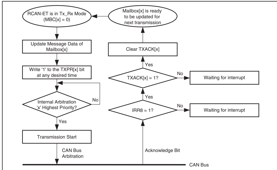
Figure 22.10 Transmission Request
