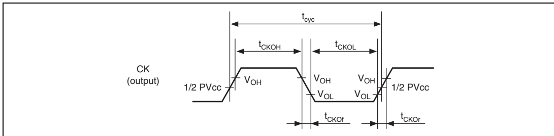
Figure 31.2 CK Clock Output Timing
