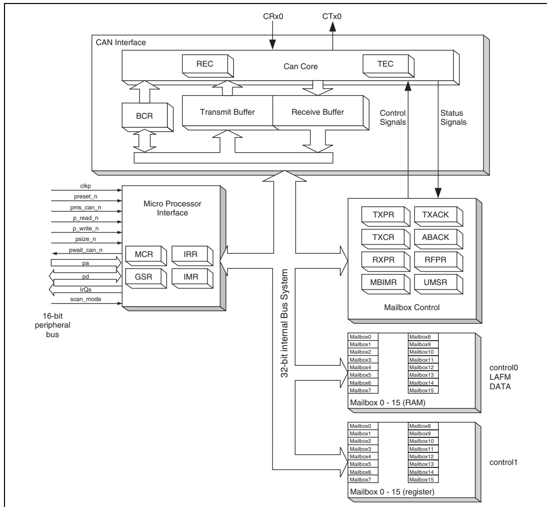
Figure 22.1 RCAN-ET Architecture
