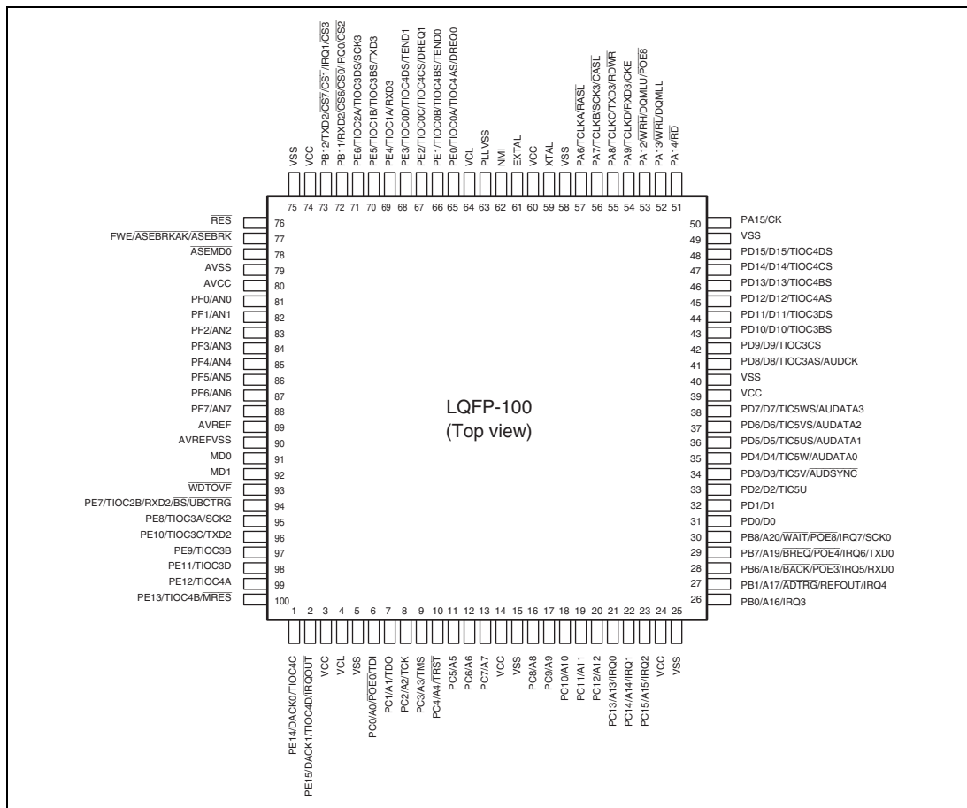
Figure 1.5 SH7243 Pin Assignment
