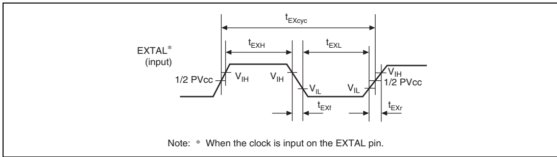
Figure 31.1 EXTAL Clock Input Timing
