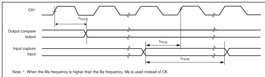
Figure 31.42 MTU2S Input/Output Timing
