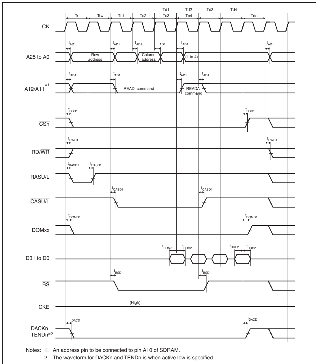
Figure 31.21 Synchronous DRAM Burst Read Bus Cycle (Four Read Cycles) (Auto Precharge, CAS Latency 2, WTRCD = 1 Cycle, WTRP = 0 Cycle)
