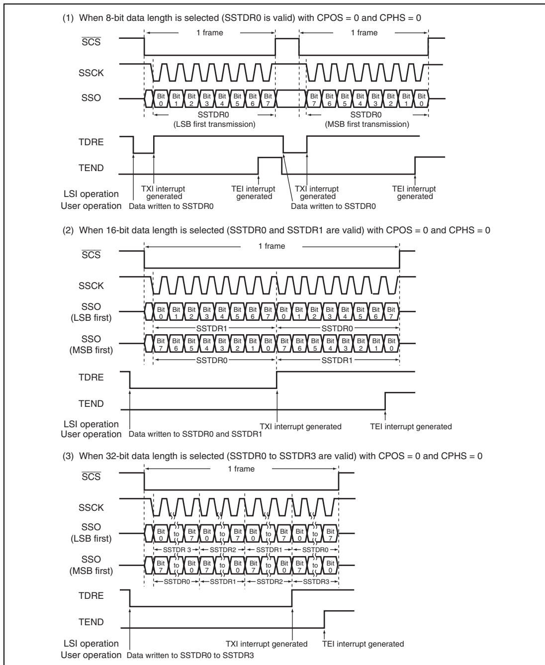
Figure 18.5 Example of Transmission Operation (SSU Mode)
