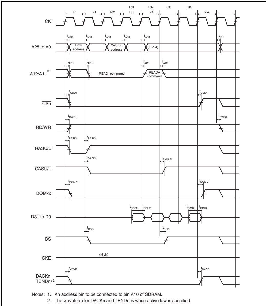
Figure 31.20 Synchronous DRAM Burst Read Bus Cycle (Four Read Cycles) (Auto Precharge, CAS Latency 2, WTRCD = 0 Cycle, WTRP = 1 Cycle)
