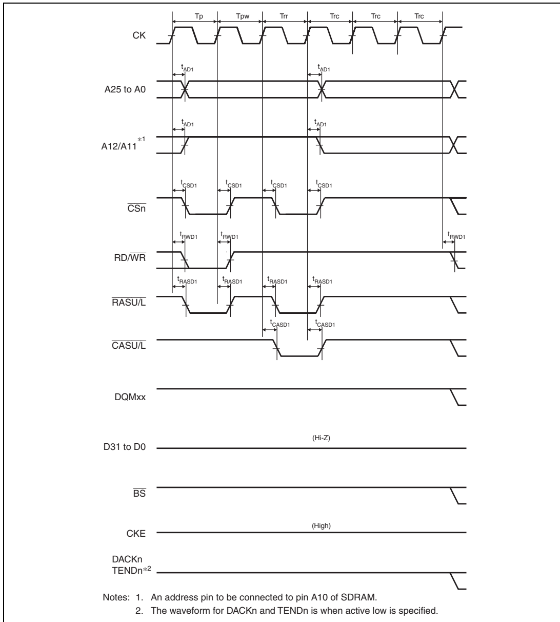
Figure 31.32 Synchronous DRAM Auto-Refreshing Timing (WTRP = 1 Cycle, WTRC = 3 Cycles)
