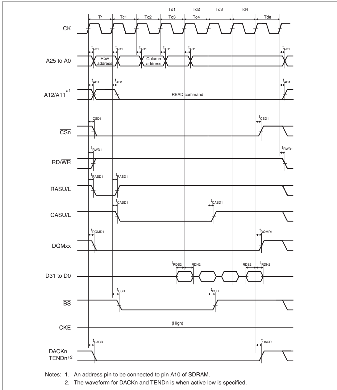
Figure 31.26 Synchronous DRAM Burst Read Bus Cycle (Four Read Cycles) (Bank Active Mode: ACT + READ Commands, CAS Latency 2, WTRCD = 0 Cycle)
