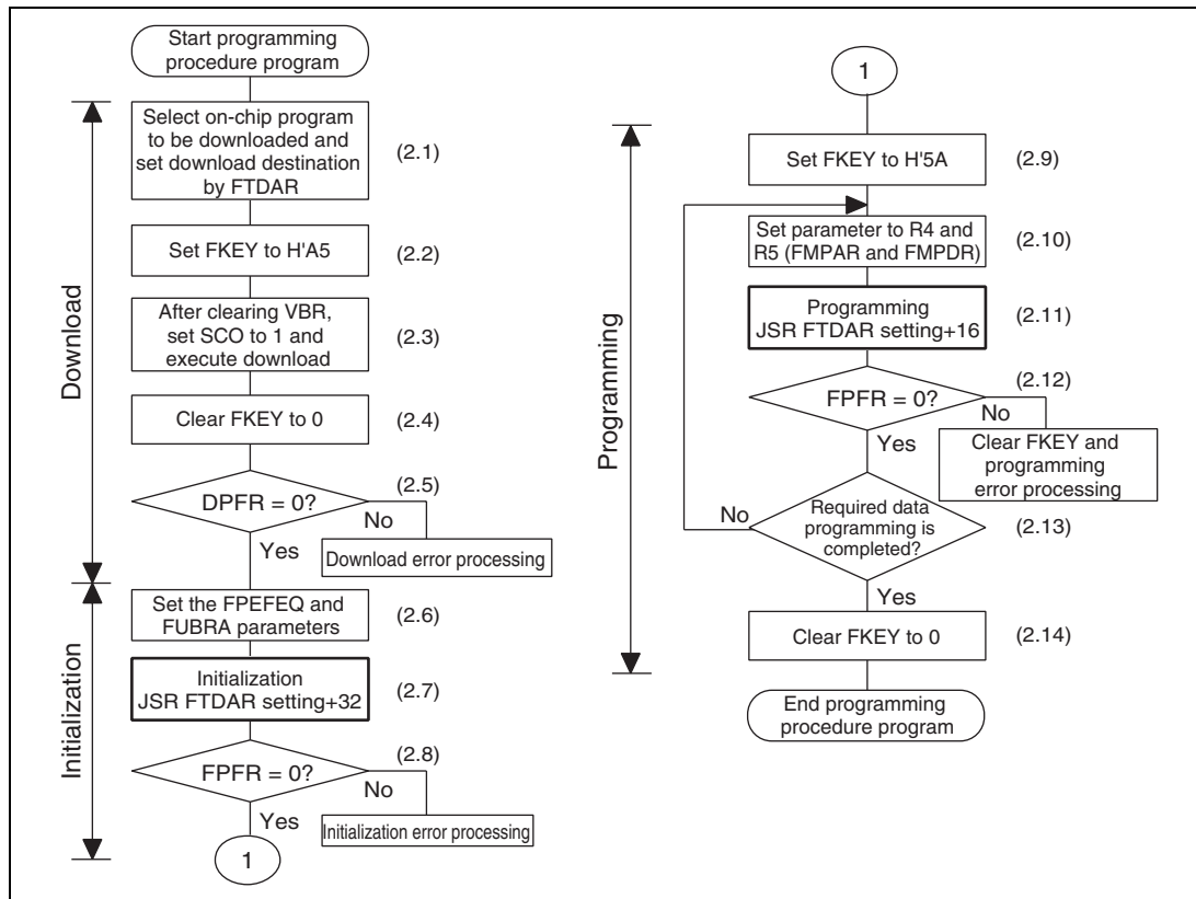
Figure 26.13 Programming Procedure
