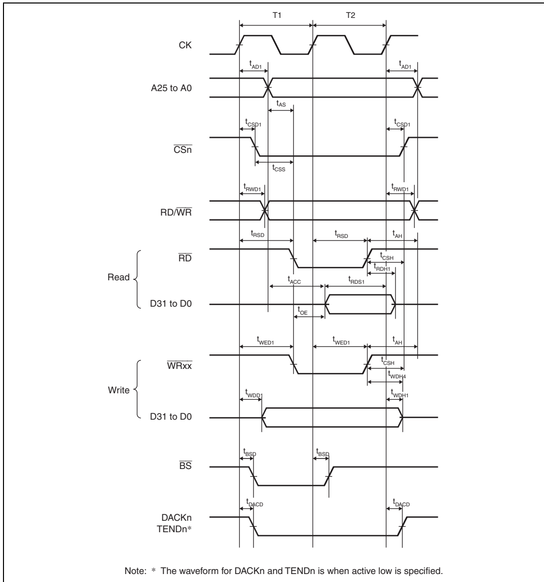
Figure 31.10 Basic Bus Timing for Normal Space (No Wait)
