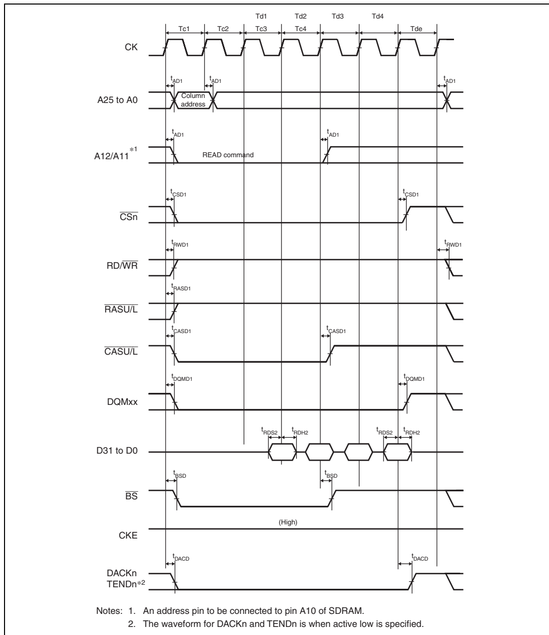
Figure 31.27 Synchronous DRAM Burst Read Bus Cycle (Four Read Cycles) (Bank Active Mode: READ Command, Same Row Address, CAS Latency 2, WTRCD = 0 Cycle)
