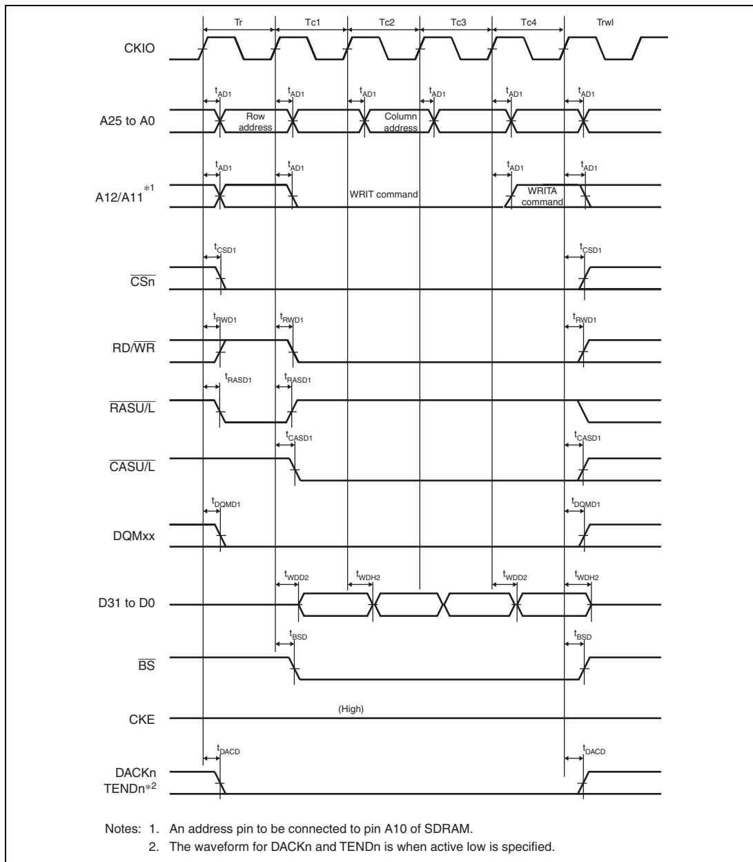
Figure 35.28 Synchronous DRAM Burst Write Bus Cycle (Four Write Cycles) (Auto Precharge, WTRCD = 0 Cycle, TRWL = 1 Cycle)
