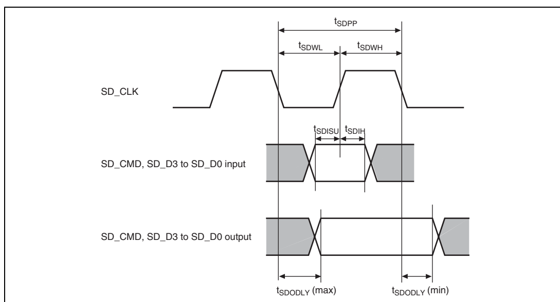
Figure 35.79 SD Card Interface
