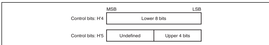
Figure 20.3 Locked Address Configuration
