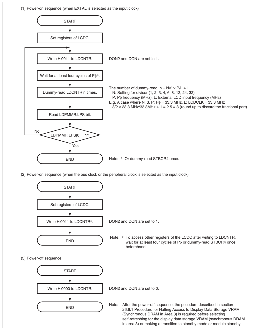
Figure 26.4 Flowchart for Power-Supply Control Sequences
