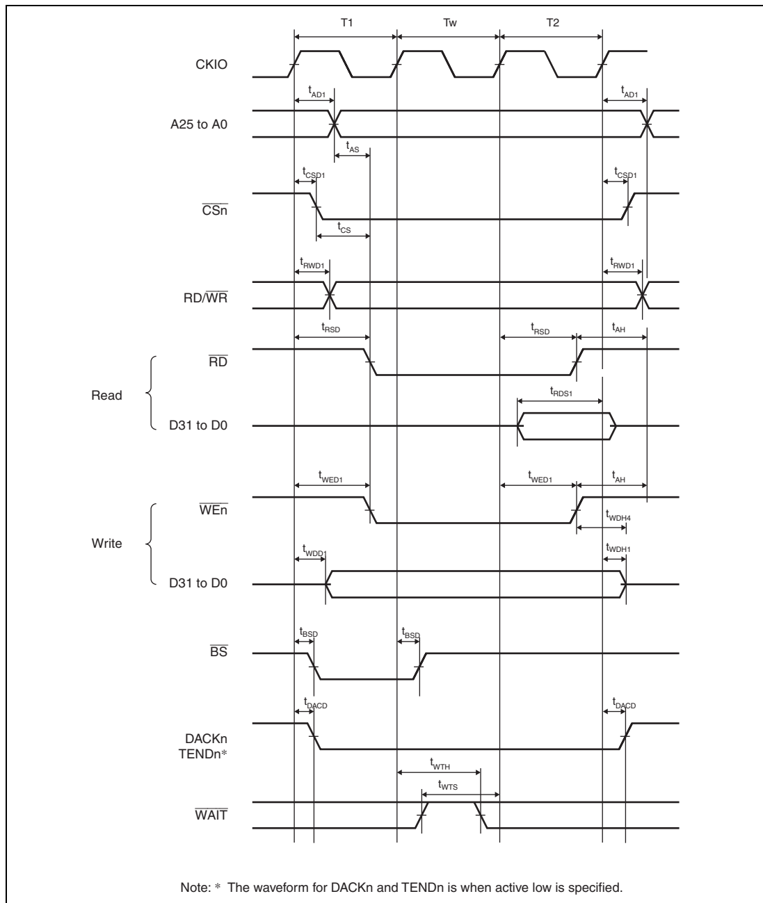
Figure 35.14 Basic Bus Timing for Normal Space (One Software Wait Cycle)
