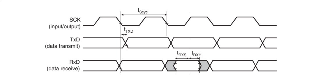
Figure 35.52 SCIF Input/Output Timing in Clocked Synchronous Mode
