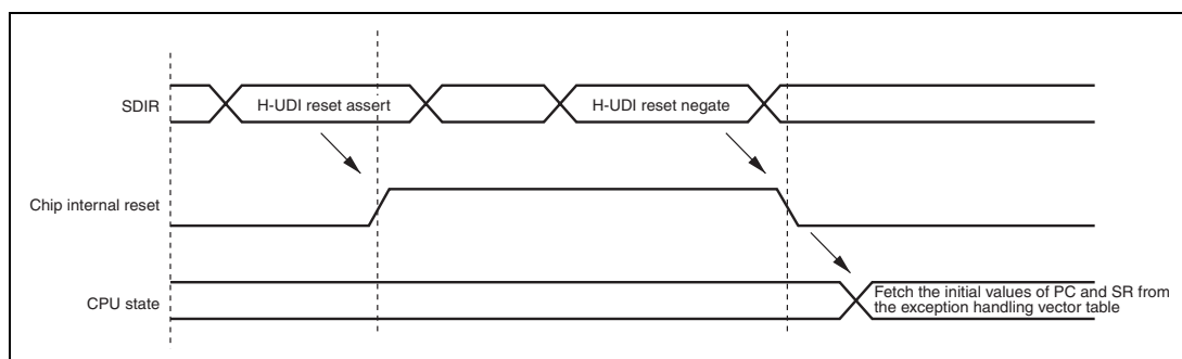
Figure 33.4 H-UDI Reset
