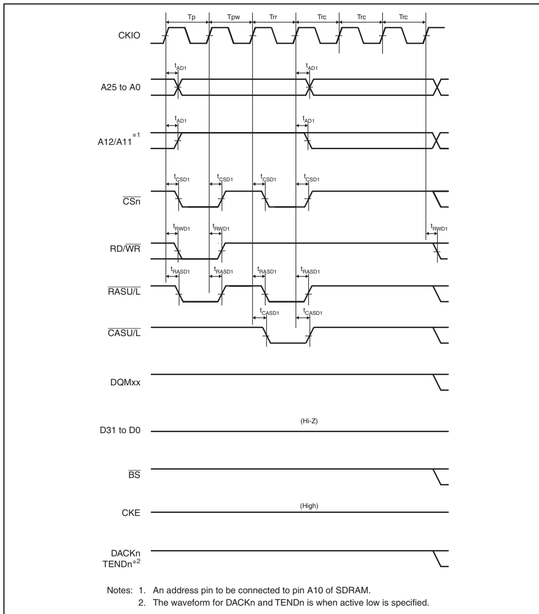
Figure 35.36 Synchronous DRAM Auto-Refreshing Timing (WTRP = 1 Cycle, WTRC = 3 Cycles)
