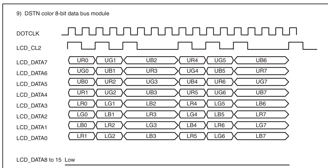
Figure 26.19 Clock and LCD Data Signal Example (DSTN Color 8-Bit Data Bus Module)
