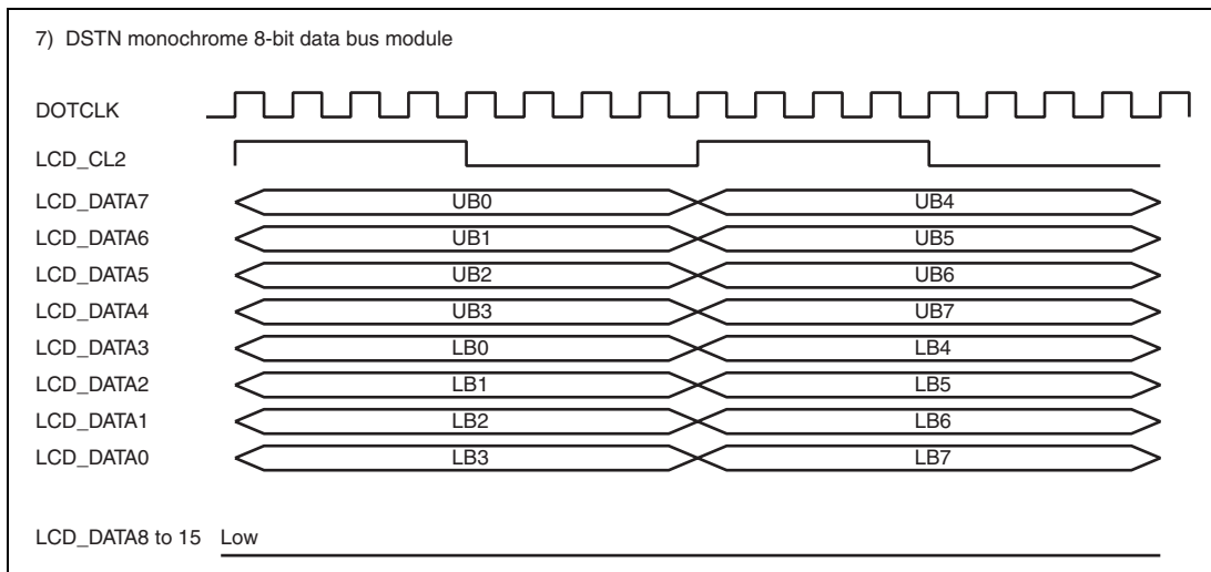
Figure 26.17 Clock and LCD Data Signal Example (DSTN Monochrome 8-Bit Data Bus Module)
