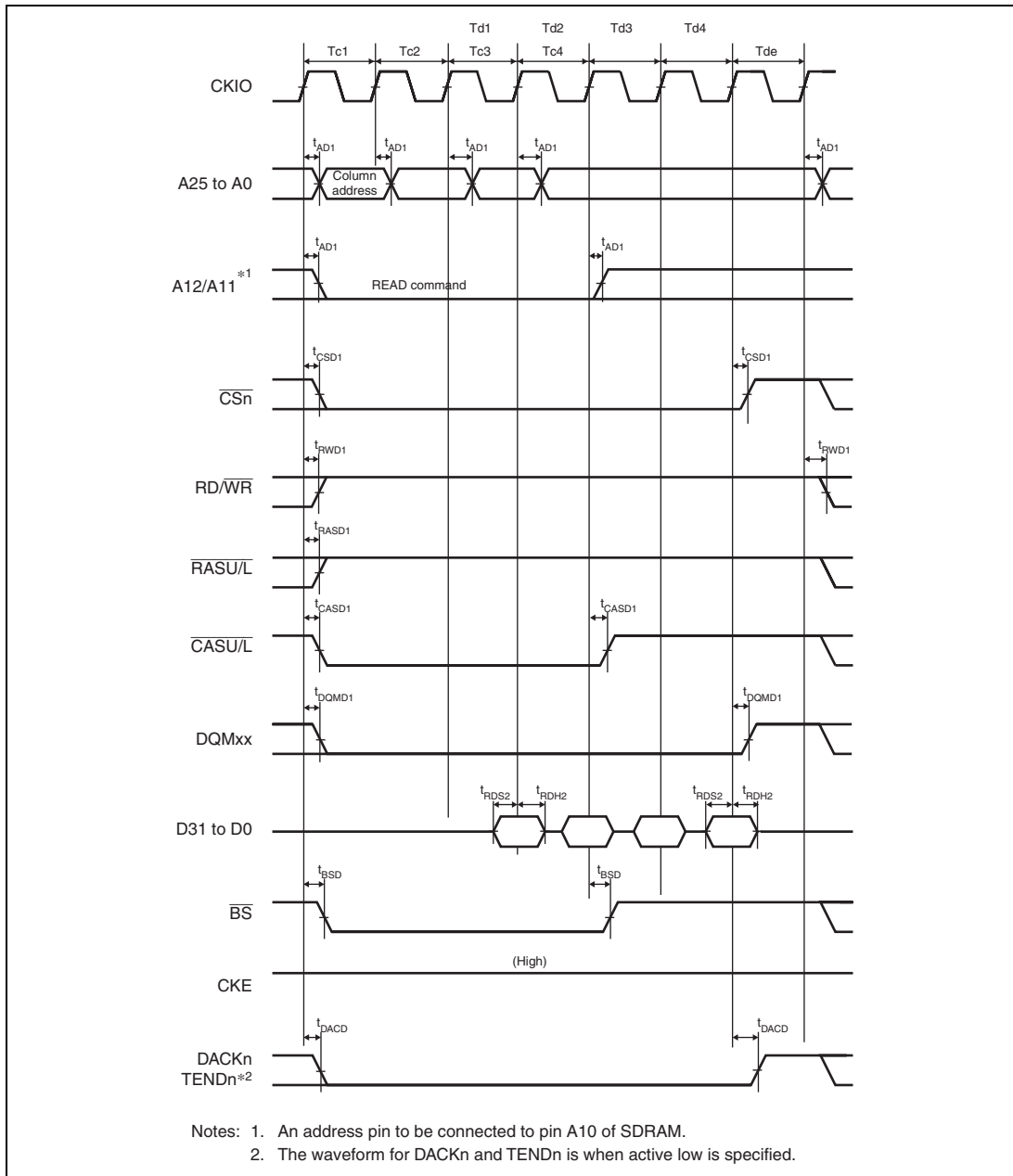
Figure 35.31 Synchronous DRAM Burst Read Bus Cycle (Four Read Cycles) (Bank Active Mode: READ Command, Same Row Address, CAS Latency 2, WTRCD = 0 Cycle)
