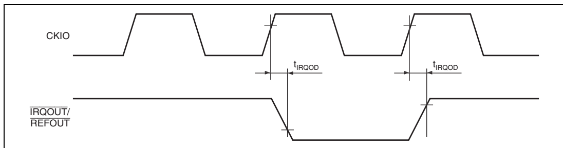
Figure 35.11 Interrupt Signal Output Timing
