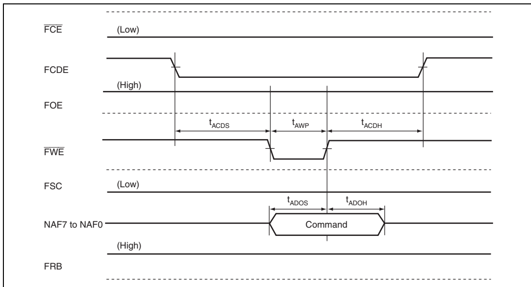
Figure 35.64 AND Type Flash Memory Command Issuance Timing
