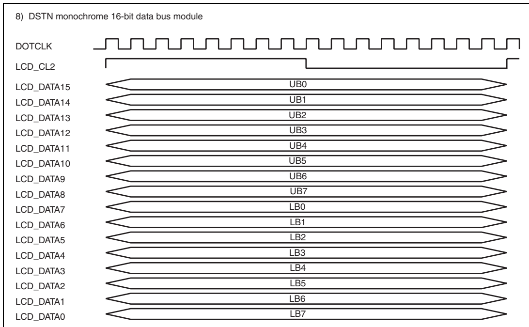
Figure 26.18 Clock and LCD Data Signal Example (DSTN Monochrome 16-Bit Data Bus Module)
