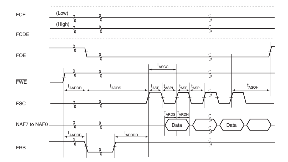
Figure 35.66 AND Type Flash Memory Data Read Timing
