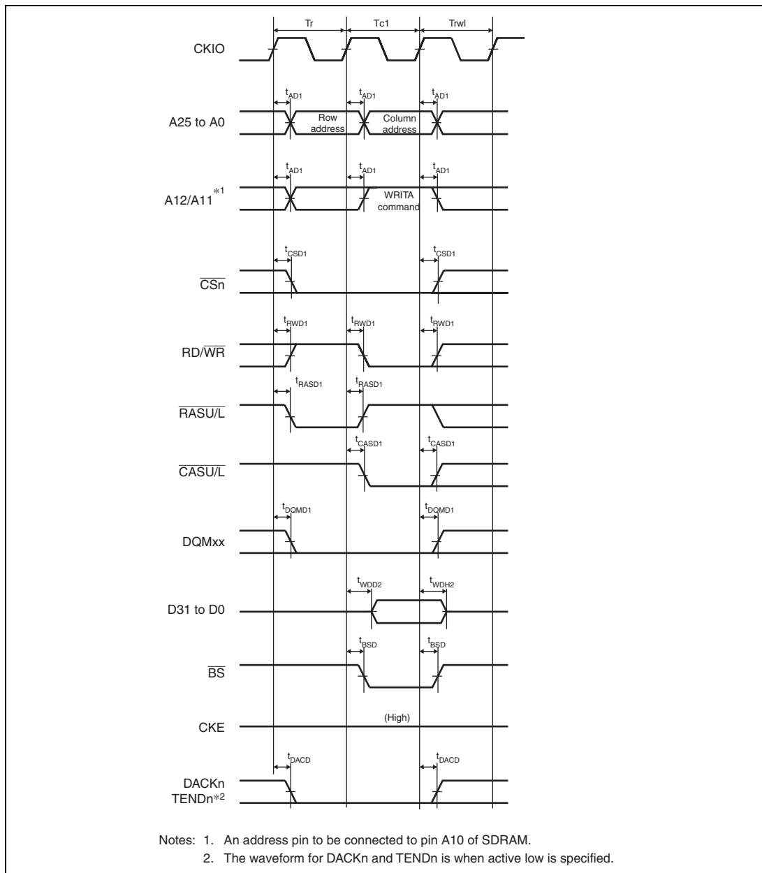
Figure 35.26 Synchronous DRAM Single Write Bus Cycle (Auto Precharge, TRWL = 1 Cycle)
