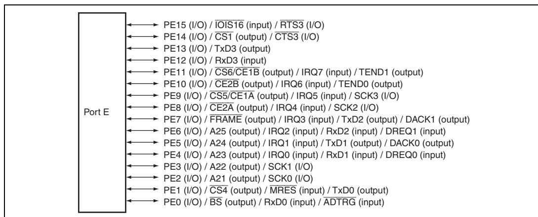
Figure 30.5 Port E
