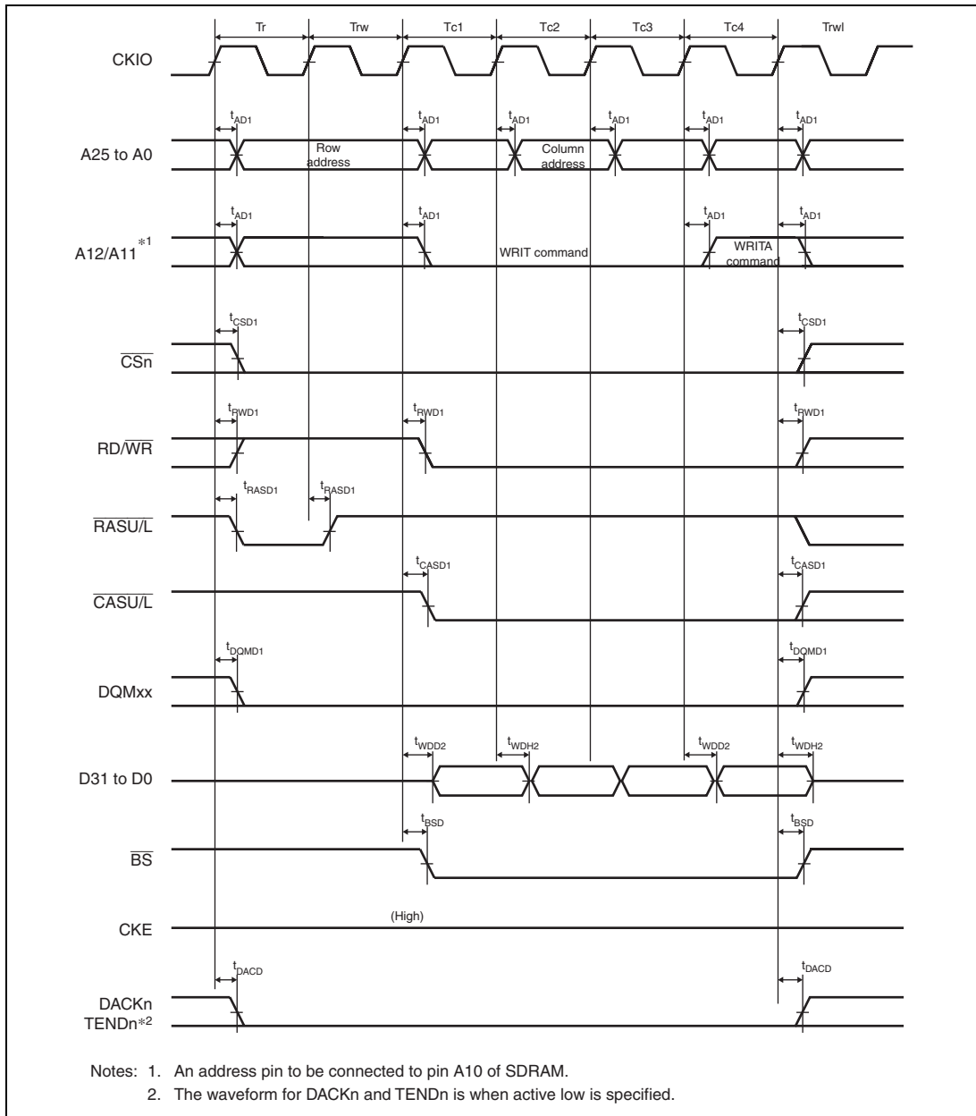
Figure 35.29 Synchronous DRAM Burst Write Bus Cycle (Four Write Cycles) (Auto Precharge, WTRCD = 1 Cycle, TRWL = 1 Cycle)
