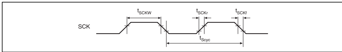
Figure 35.51 SCK Input Clock Timing
