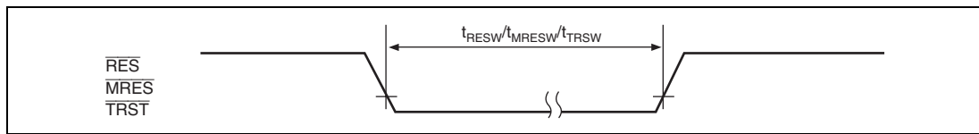
Figure 35.9 Reset Input Timing
