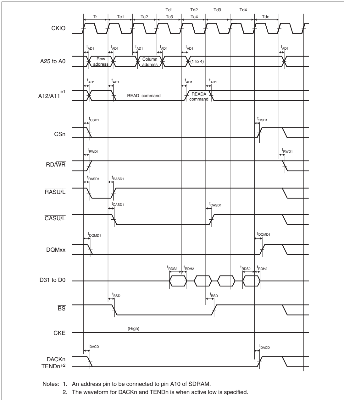
Figure 35.24 Synchronous DRAM Burst Read Bus Cycle (Four Read Cycles) (Auto Precharge, CAS Latency 2, WTRCD = 0 Cycle, WTRP = 1 Cycle)
