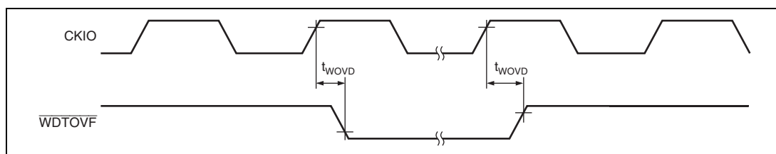
Figure 35.50 WDT Timing
