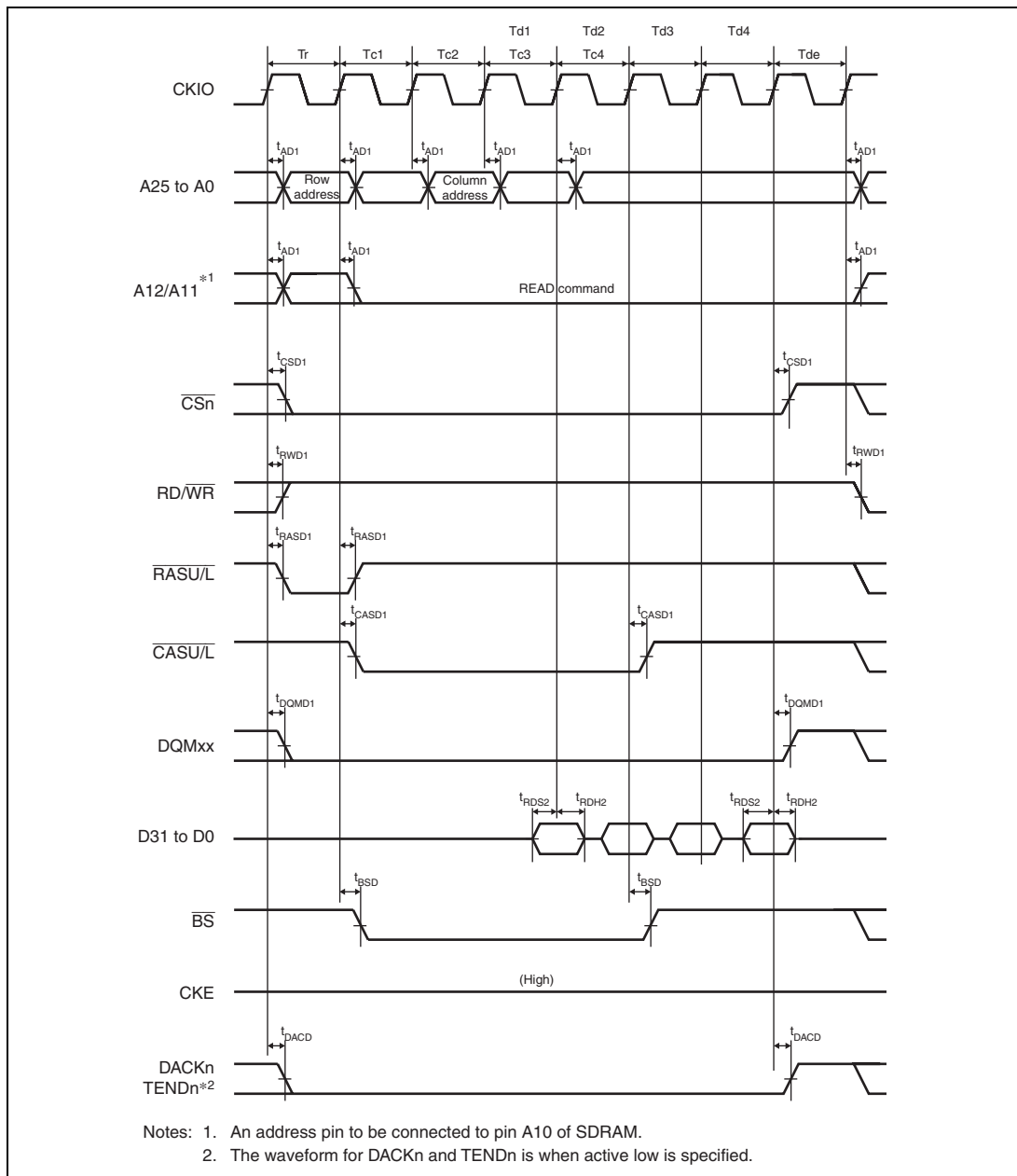
Figure 35.30 Synchronous DRAM Burst Read Bus Cycle (Four Read Cycles) (Bank Active Mode: ACT + READ Commands, CAS Latency 2, WTRCD = 0 Cycle)
