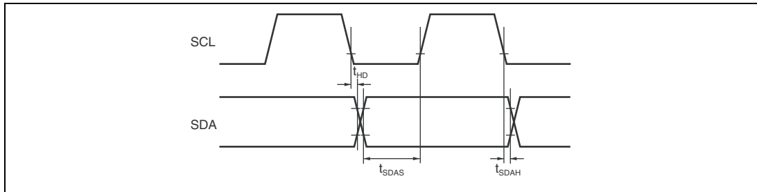
Figure 35.57 (3) Transmission and Reception Timing
