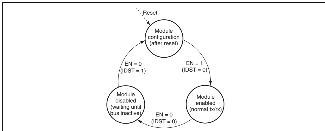
Figure 18.19 Operation Modes
