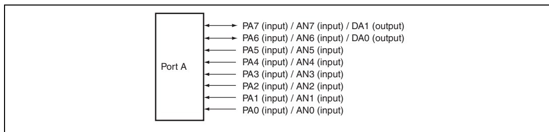
Figure 30.1 Port A
