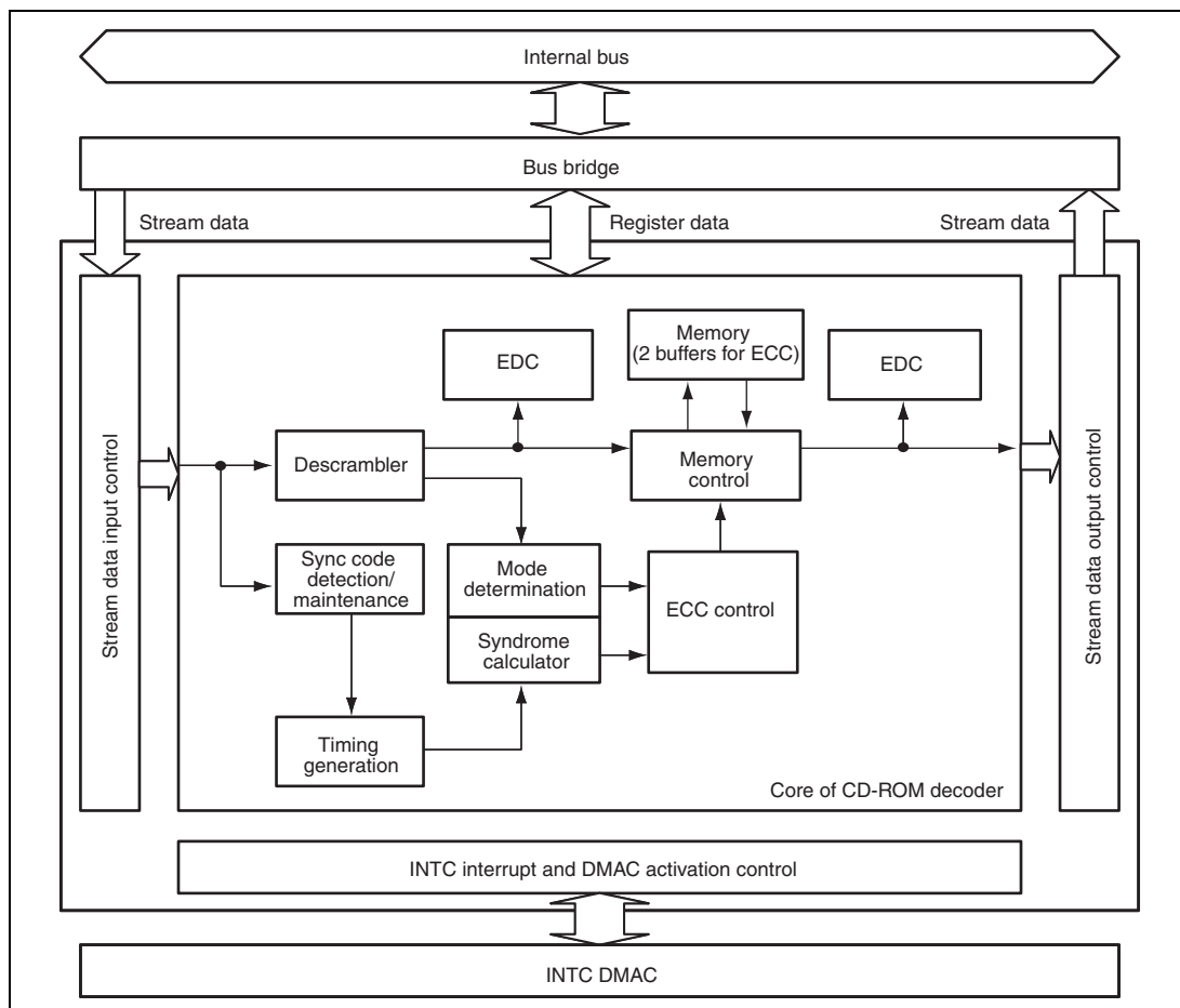
Figure 21.2 ROM-DEC Block Diagram
