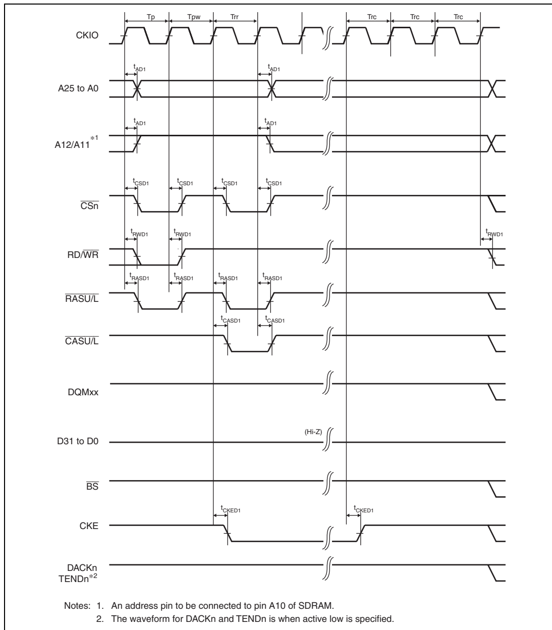
Figure 35.37 Synchronous DRAM Self-Refreshing Timing (WTRP = 1 Cycle)
