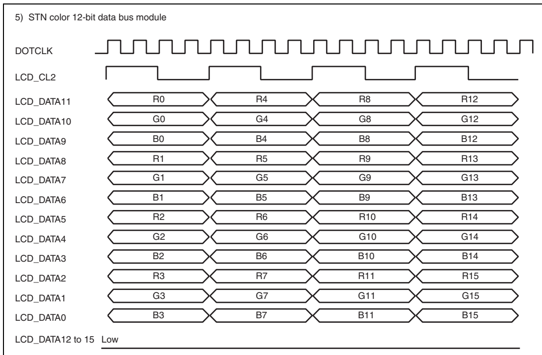
Figure 26.15 Clock and LCD Data Signal Example (STN Color 12-Bit Data Bus Module)
