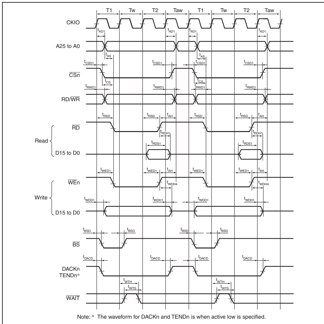
Figure 35.16 Basic Bus Timing for Normal Space (One Software Wait Cycle, External Wait Cycle Valid (WM Bit = 0), No Idle Cycle)
