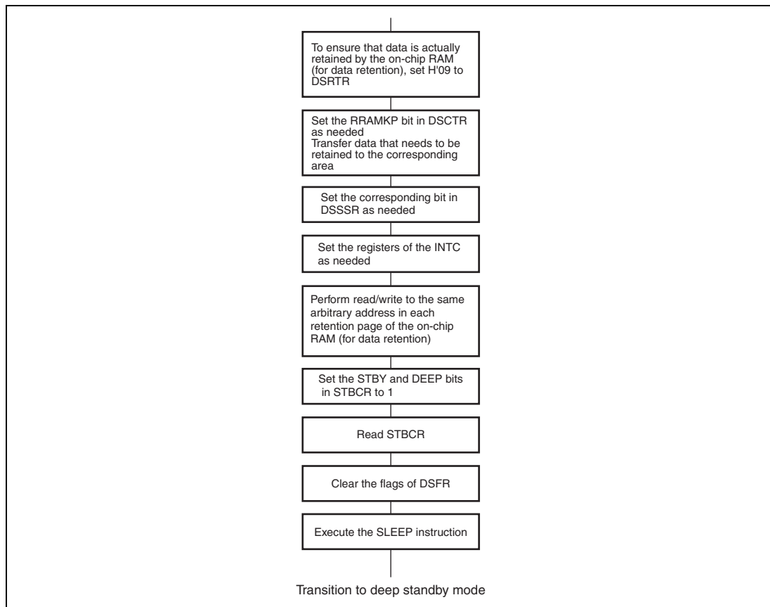
Figure 32.2 Flowchart of Transition to Deep Standby Mode
