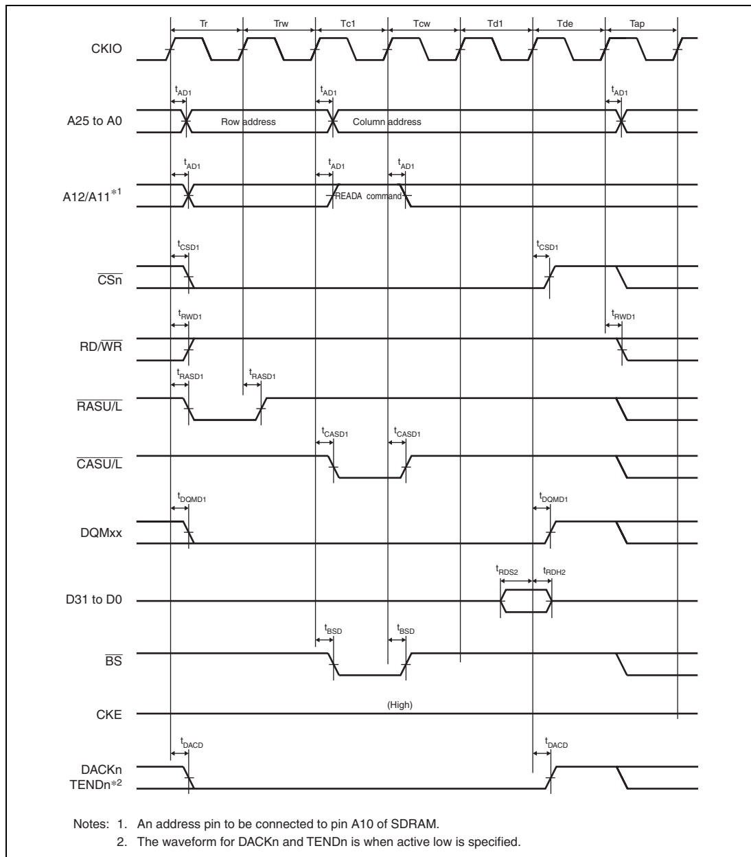
Figure 35.23 Synchronous DRAM Single Read Bus Cycle (Auto Precharge, CAS Latency 2, WTRCD = 1 Cycle, WTRP = 1 Cycle)
