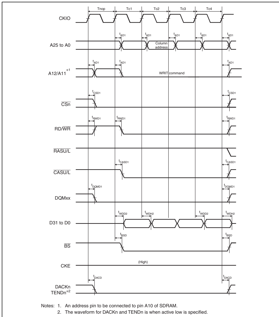
Figure 35.34 Synchronous DRAM Burst Write Bus Cycle (Four Write Cycles) (Bank Active Mode: WRITE Command, Same Row Address, WTRCD = 0 Cycle, TRWL = 0 Cycle)
