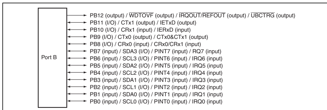
Figure 30.2 Port B
