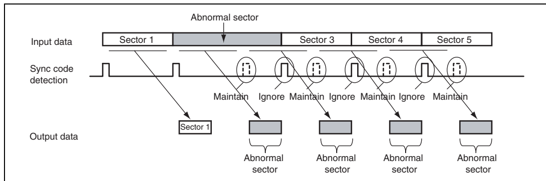
Figure 21.12 Operation in Interpolated Sync Mode
