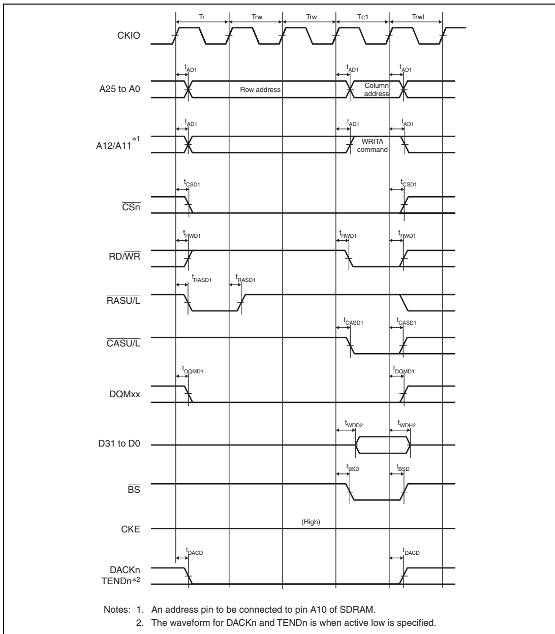
Figure 35.27 Synchronous DRAM Single Write Bus Cycle (Auto Precharge, WTRCD = 2 Cycles, TRWL = 1 Cycle)
