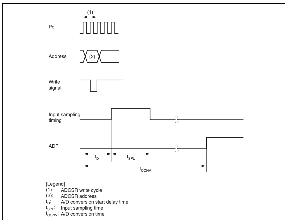
Figure 22.5 A/D Conversion Timing
