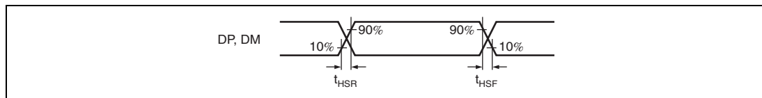
Figure 35.76 DP and DM Output Timing (High-Speed)
