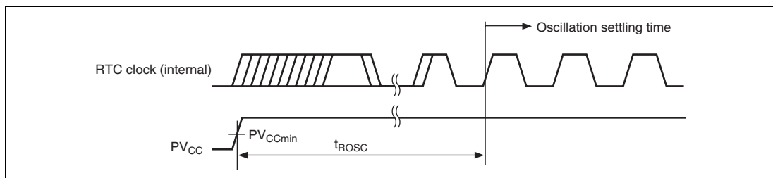
Figure 35.8 RTC Clock Oscillation Settling Time
