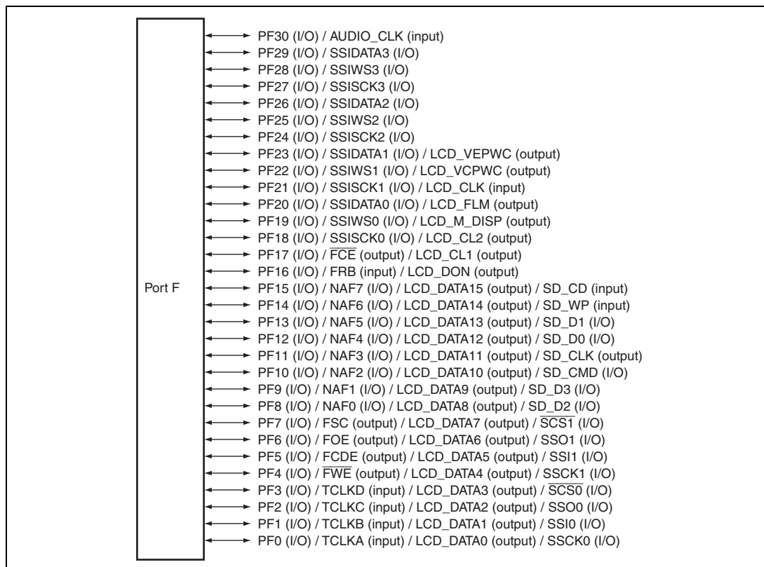
Figure 30.6 Port F
