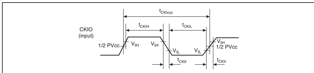
Figure 35.3 CKIO Clock Input Timing
