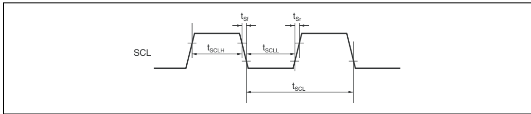
Figure 35.57 (2) Clock Input/Output Timing
