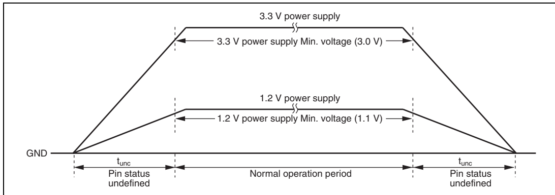
Figure 35.1 Power-on/Power-off Sequence
