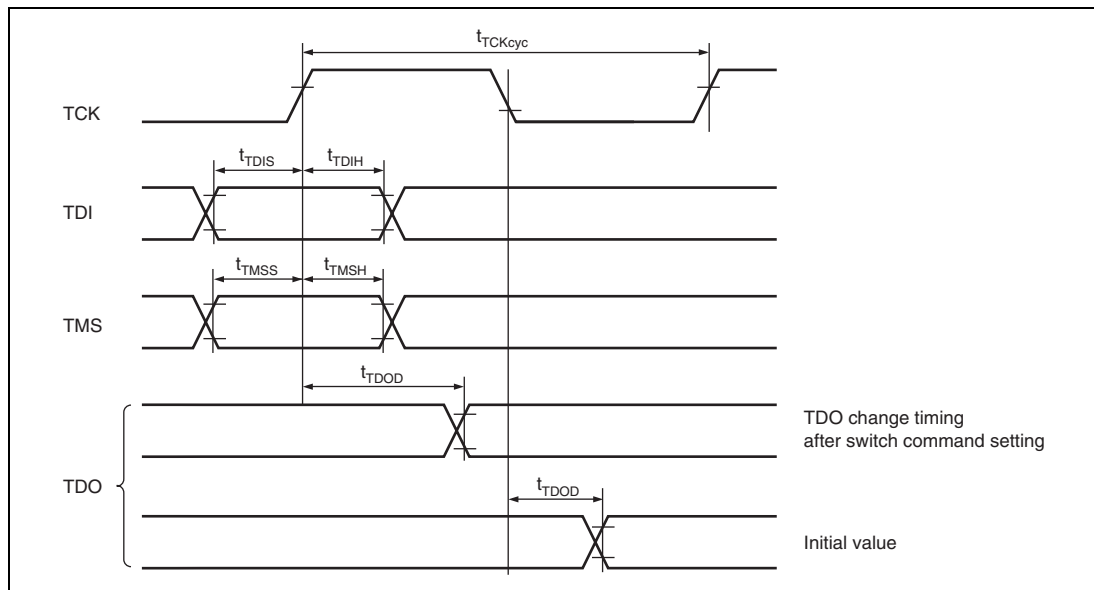
Figure 35.82 H-UDI Data Transfer Timing
