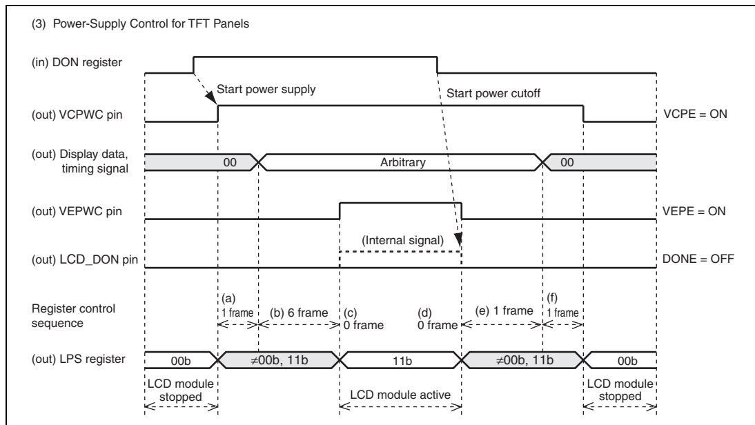
Figure 26.7 Power-Supply Control Sequence and States of the LCD Module
