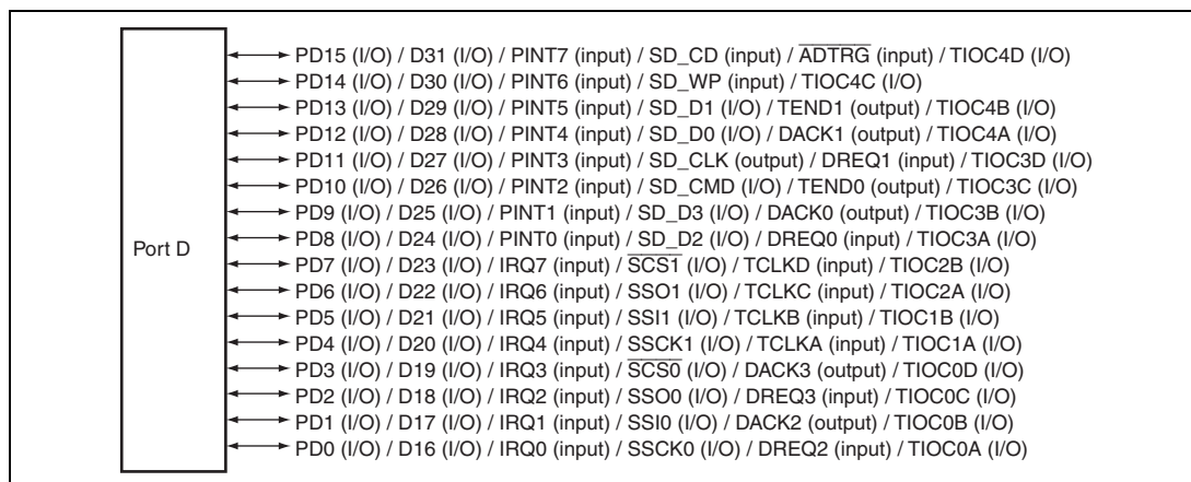
Figure 30.4 Port D
