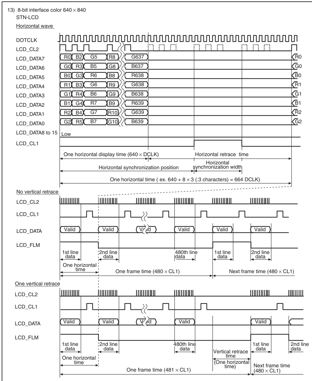
Figure 26.23 Clock and LCD Data Signal Example (8-Bit Interface Color 640 × 480)
