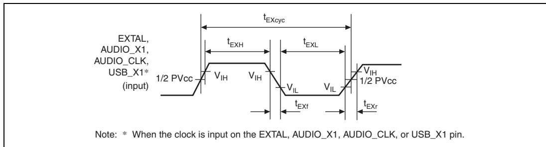
Figure 35.2 EXTAL, AUDIO_X1, AUDIO_CLK, and USB_X1 Clock Input Timing
