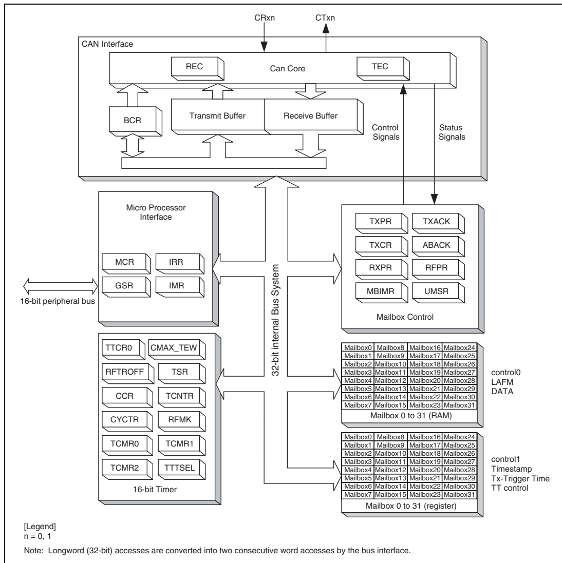
Figure 19.1 RCAN-TL1 architecture
