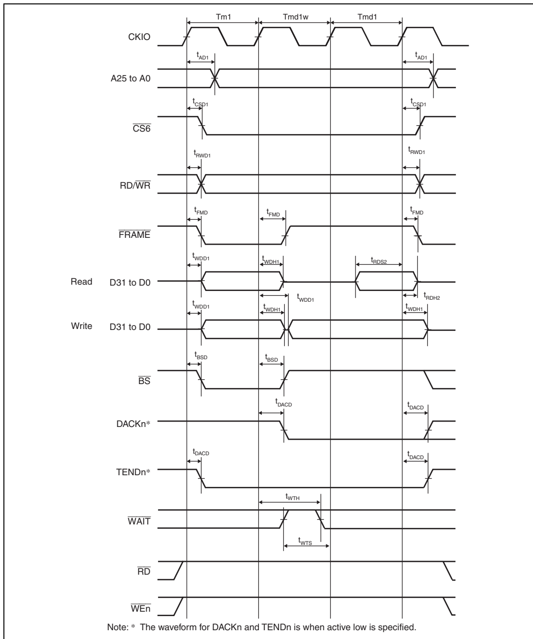
Figure 35.18 Burst MPX-I/O Interface Bus Cycle Single Read Write (One Address Cycle, One Software Wait Cycle)
