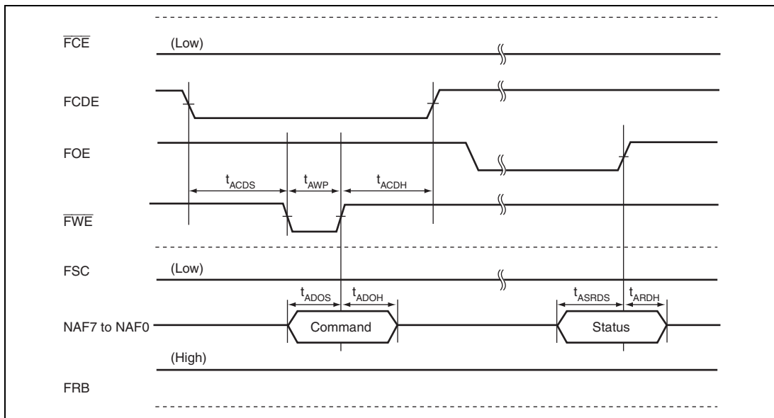
Figure 35.68 AND Type Flash Memory Status Read Timing
