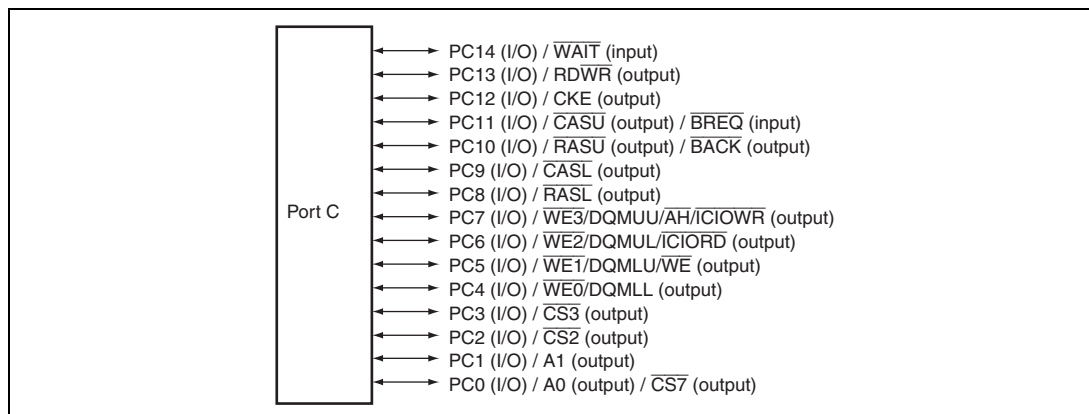
Figure 30.3 Port C
