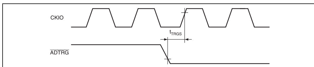
Figure 35.63 A/D Converter External Trigger Input Timing
