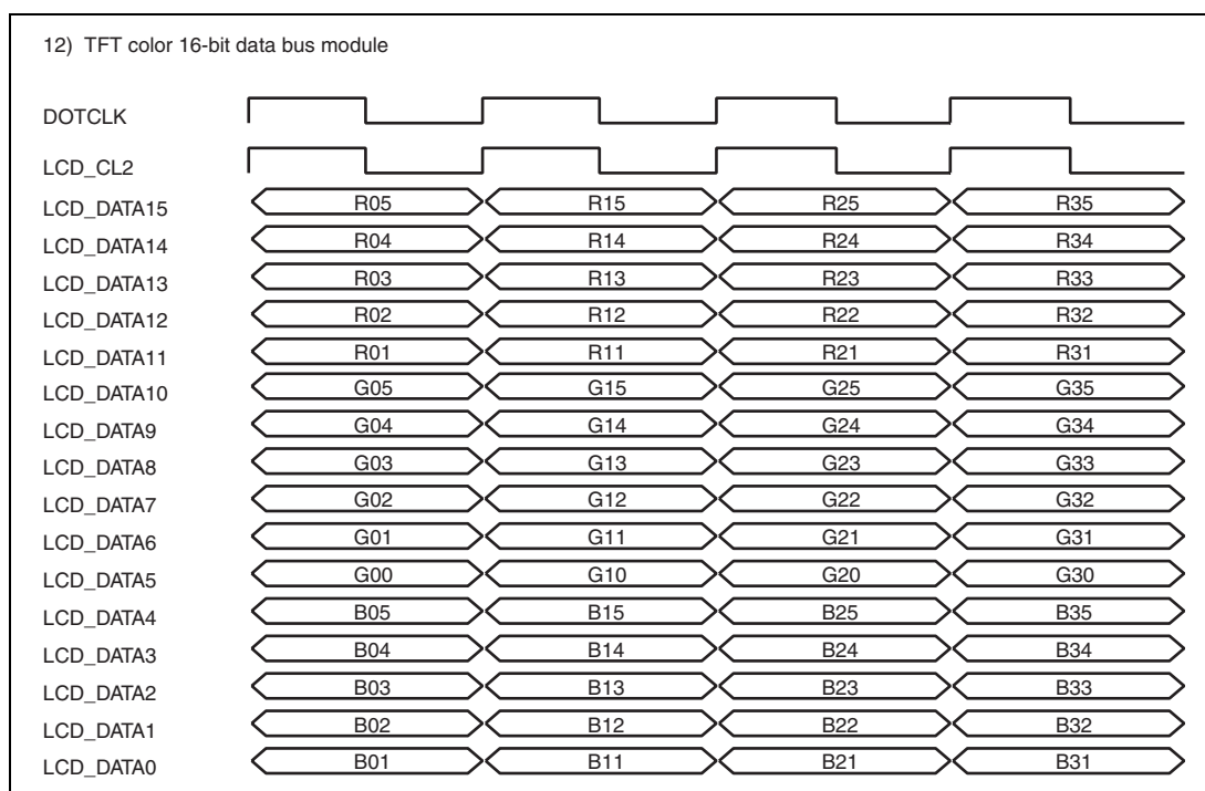
Figure 26.22 Clock and LCD Data Signal Example (TFT Color 16-Bit Data Bus Module)
