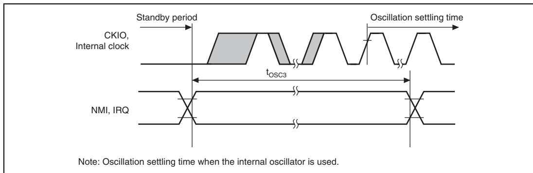
Figure 35.7 Oscillation Settling Time on Return from Standby (Return by NMI or IRQ)
