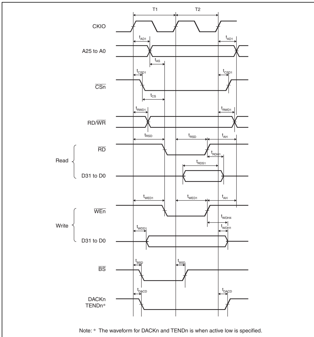
Figure 35.13 Basic Bus Timing for Normal Space (No Wait)
