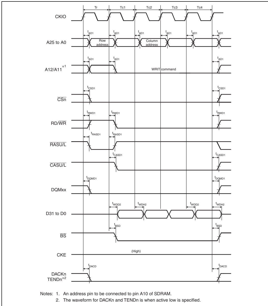
Figure 35.33 Synchronous DRAM Burst Write Bus Cycle (Four Write Cycles) (Bank Active Mode: ACT + WRITE Commands, WTRCD = 0 Cycle, TRWL = 0 Cycle)
