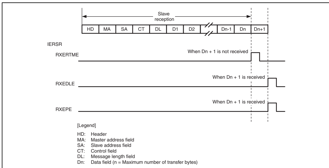
Figure 20.19 Timing of Operations when Reception Has Not Been Completed Within the Maximum Number of Transfer Bytes
