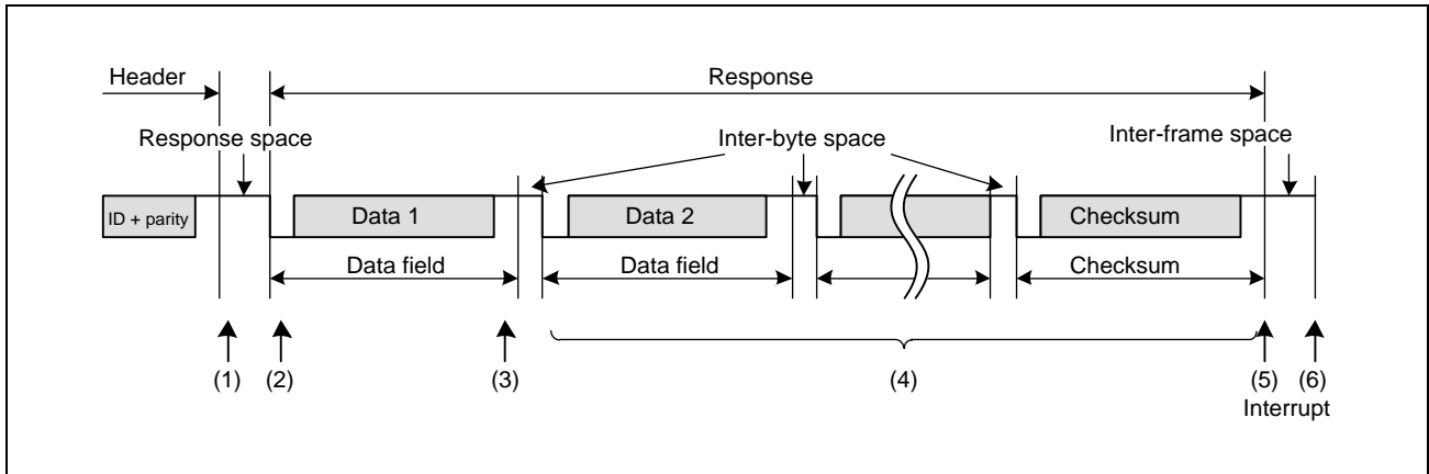
Figure 22.12 Operation in Response Reception
