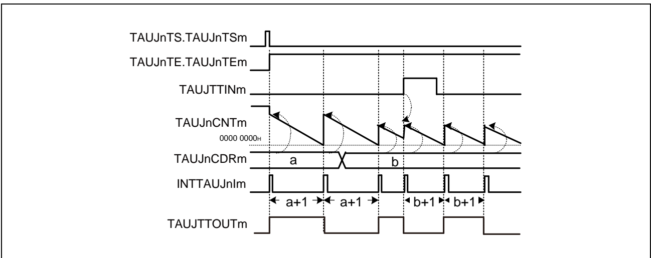
Figure 33.23 General Timing Diagram for TAUJTTINm Input Interval Timer Function
