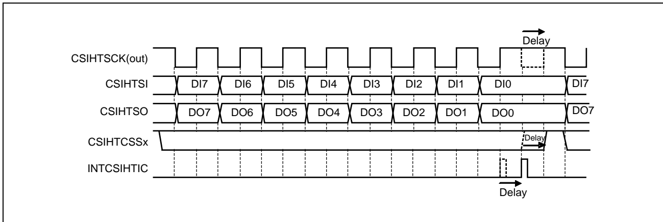
Figure 20.2 Interrupt Delay Function (CSIH n CTL1.CSIH n SIT = 1)
