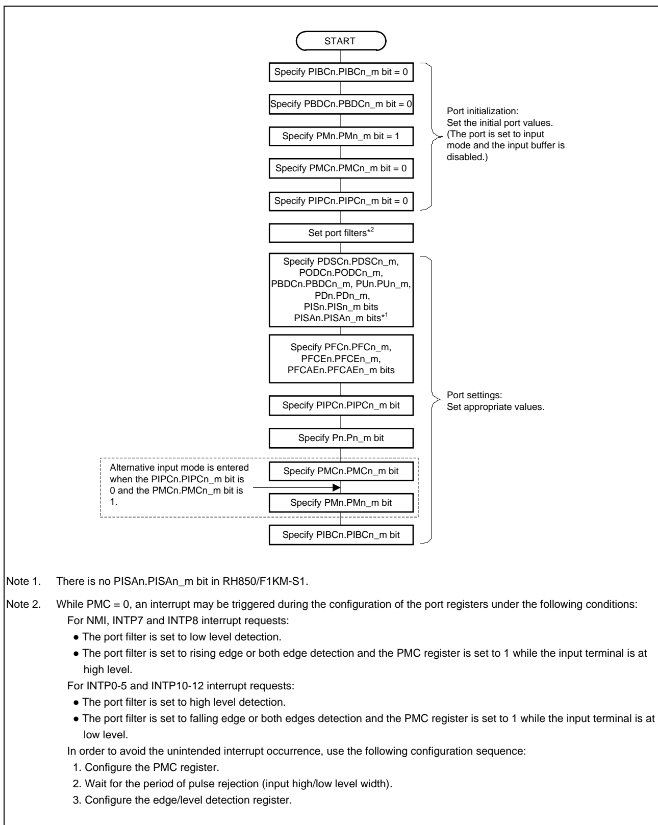
Figure 2C.6 Example of Port Settings (When Specified in Batch)
