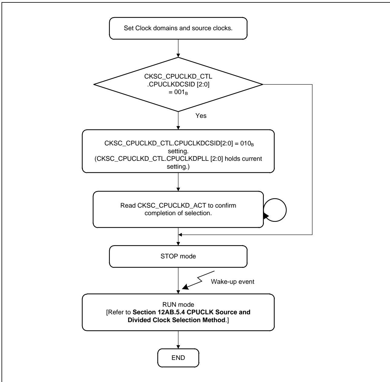
Figure 12AB.11 CPUCLK Setting in STOP Mode Method
