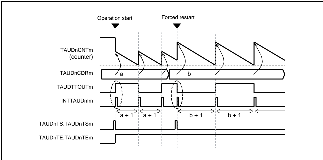
Figure 32.33 Forced Restart Operation (TAUDnCMORm.TAUDnMD0 = 1)
