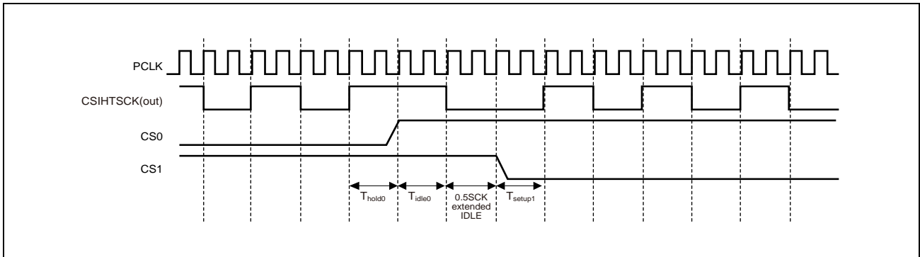
Figure 20.16 Clock Phase Timing with PCLK/4 , T_{hold0} = T_{setup1} = 0.5CSIHTSCK , T_{idle0} = 0.5CSIHTSCK , CSIHnCFG0.CSIHnCKP0 = 0 (CSIHTCSS0) → CSIHnCFG1.CSIHnCKP1 = 1 (CSIHTCSS1)
