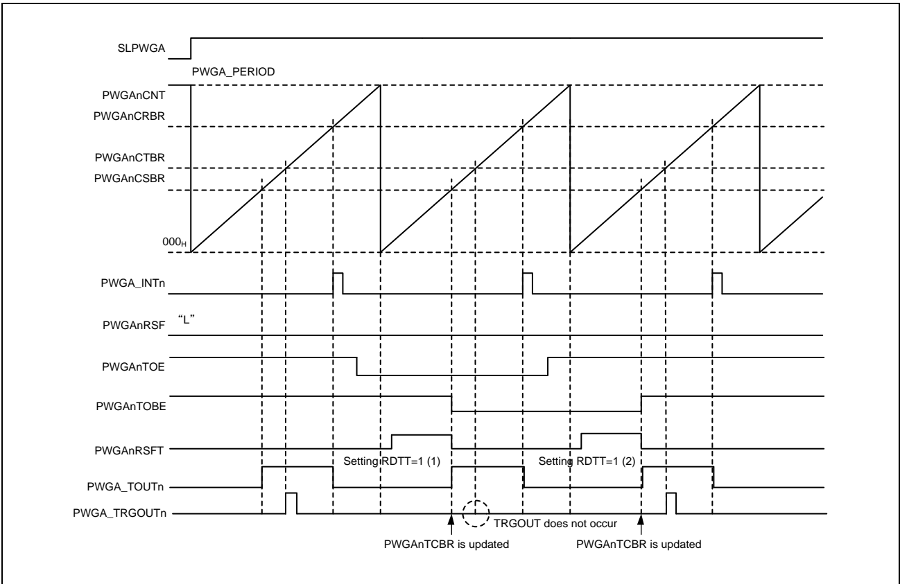
Figure 37.8 Waveform when PWGAnTCBR Register Rewrite is Executed (PWGAOCL = 0, PWGAnTCUT = 01B)
