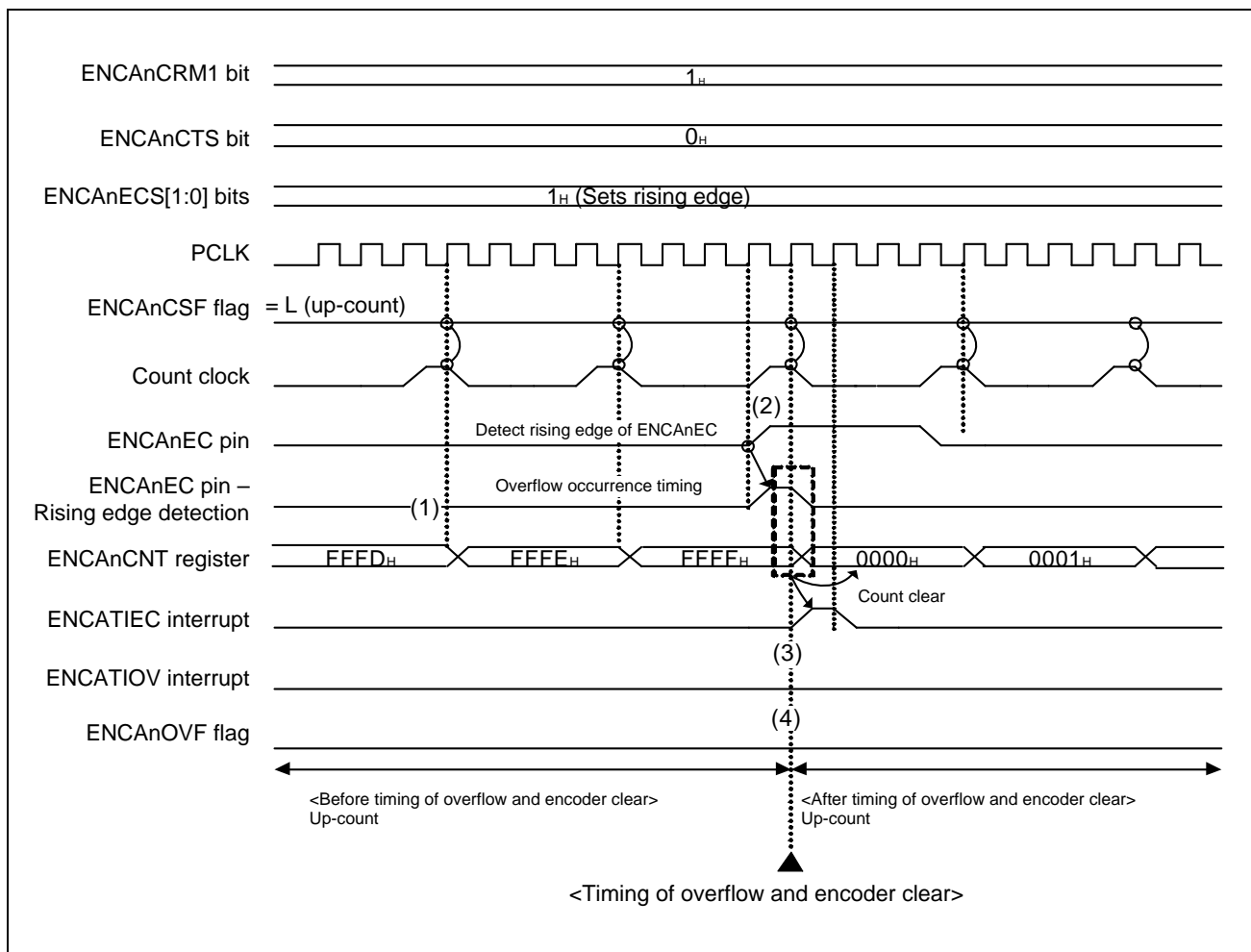
Figure 35.14 Conflict between Overflow Occurrence and Clear Operation by Encoder Clear Input (ENCA n EC pin)
