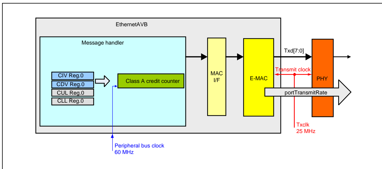
Figure 26.48 Example of CBS Settings
