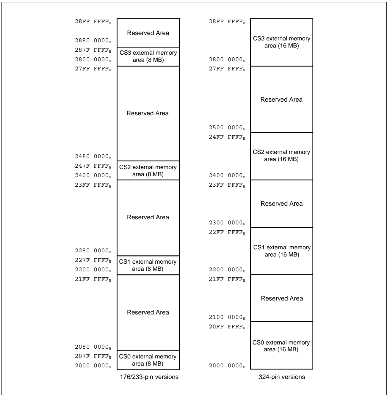
Figure 16.1 External Memory Map (RH850/F1KH-D8)
