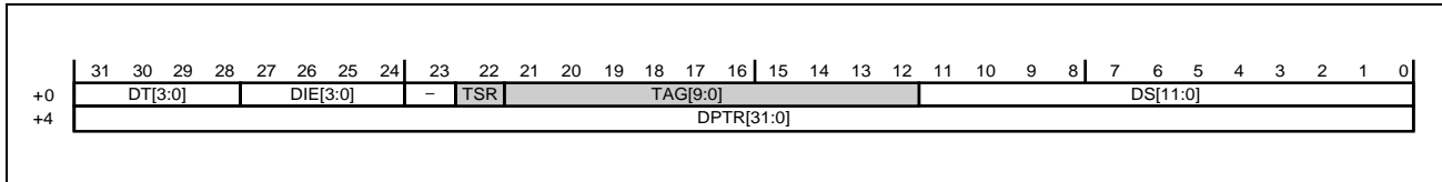
Figure 26.34 Configuration of Descriptor for a Transmitted Frame
