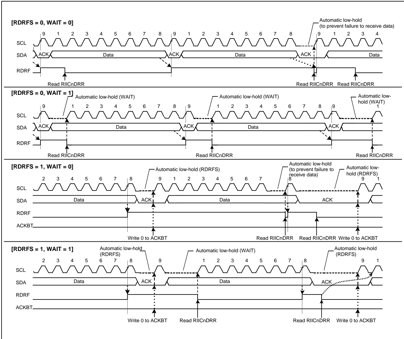
Figure 23.31 Automatic Low-Hold Operation in Receive Mode (Using RDRFS and WAIT Bits)
