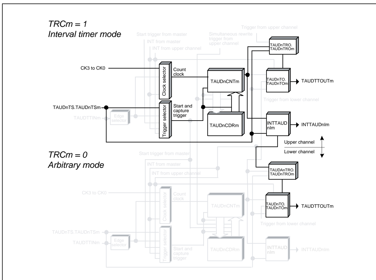
Figure 32.80 Block Diagram of Real-Time Output Function Type 1
