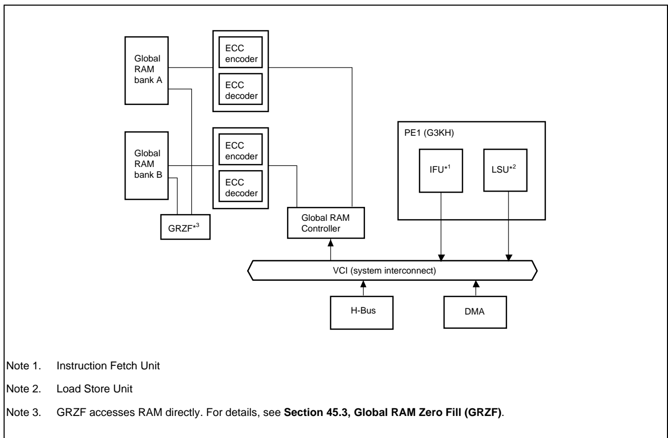
Figure 40B.2 Block Diagram of Global RAM ECC
