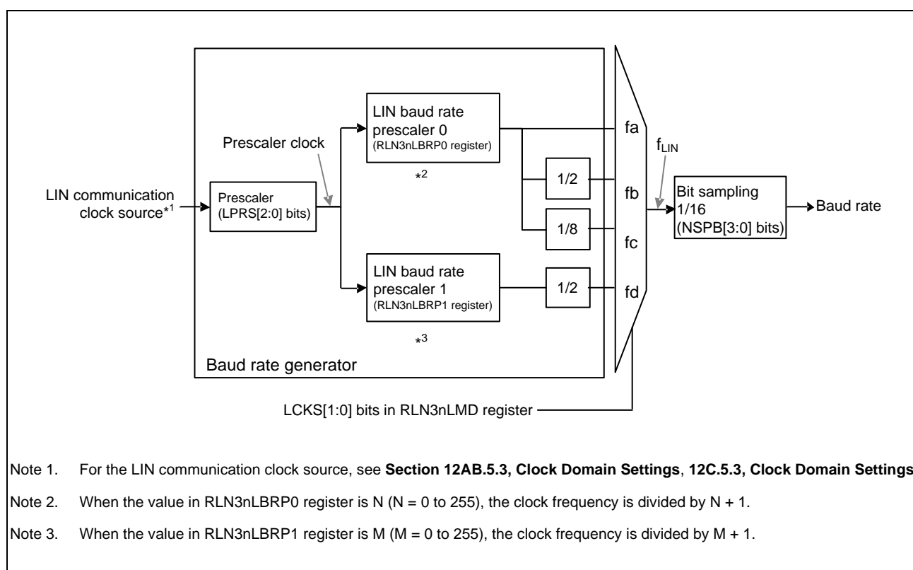
Figure 22.36 Block Diagram of Baud Rate Generation in LIN Master Mode
