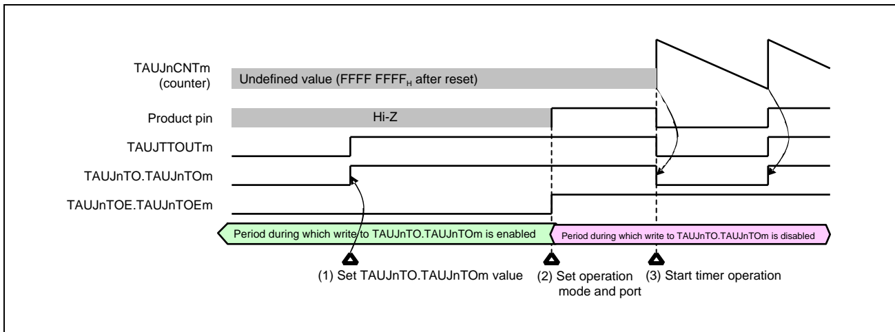
Figure 33.8 General Procedure for Specifying a TAUJTTOUT m Channel Output Mode
