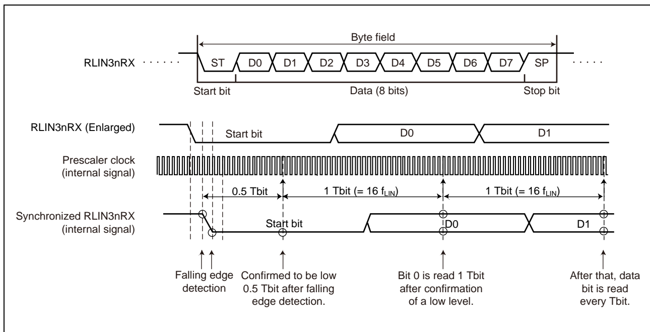
Figure 22.29 Example of Data Reception Timing (When 1 Tbit = 16 samplings)
