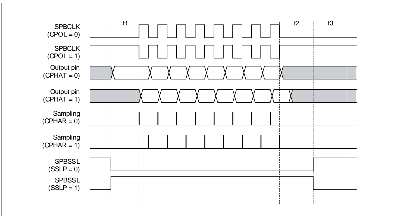
Figure 17.15 Transfer Format
