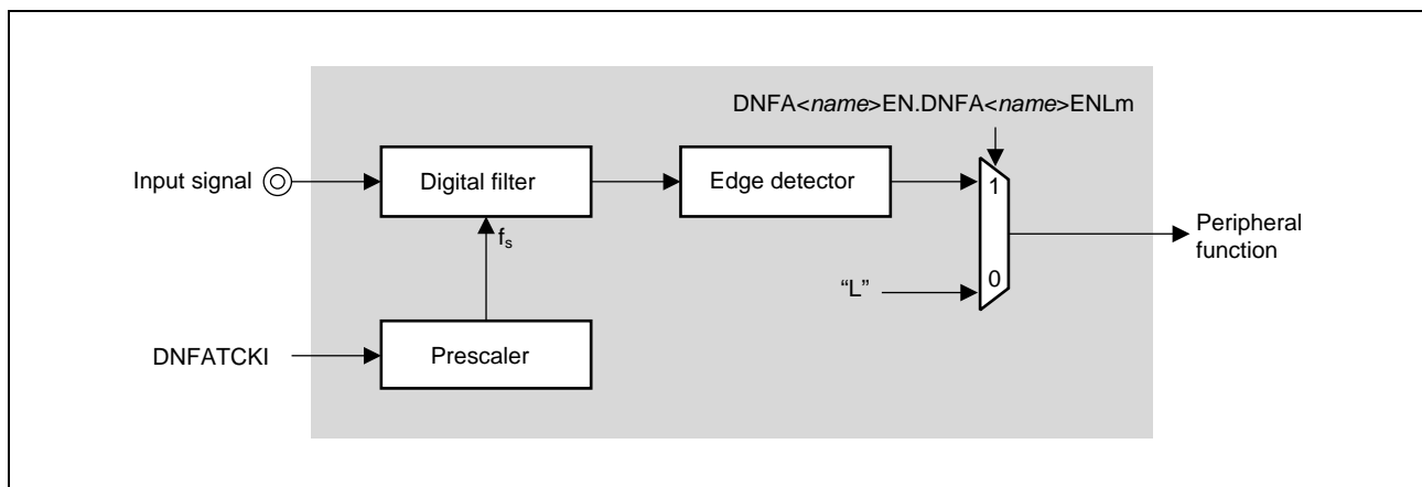
Figure 2A.16 Block Diagram of Digital Filter Type D
