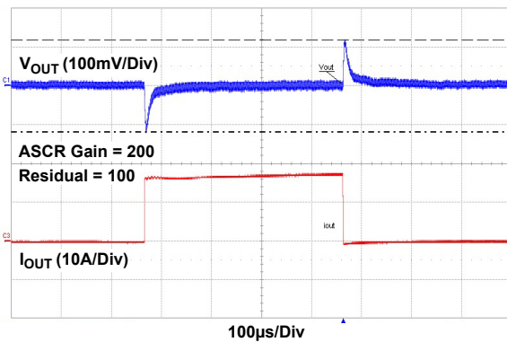
Figure 14. 12V_{IN} to 3.3V_{OUT} , f_{SW} = 615kHz , C_{OUT} = 4 \times 100\mu F Ceramic + 1 \times 470\mu F POSCAP
