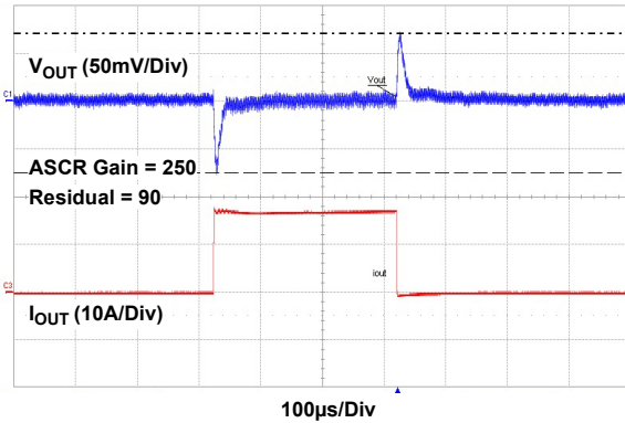
Figure 12. 12V_{IN} to 1.5V_{OUT} , f_{SW} = 471kHz , C_{OUT} = 7 \times 100\mu F Ceramic + 2 \times 470\mu F POSCAP
