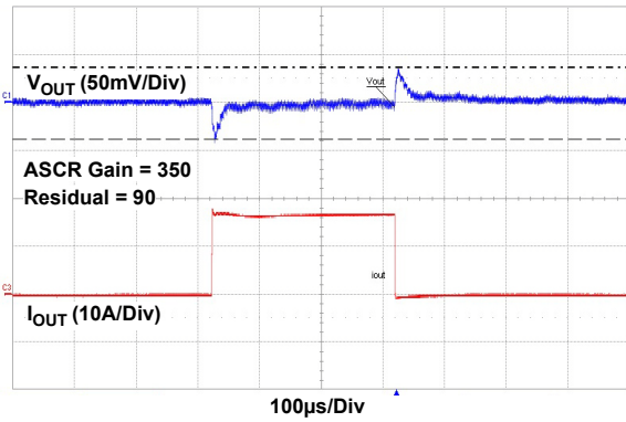
Figure 9. 5V_{IN} to 0.9V_{OUT} , f_{SW} = 364kHz , C_{OUT} = 12 \times 100\mu F Ceramic + 5 \times 470\mu F POSCAP
