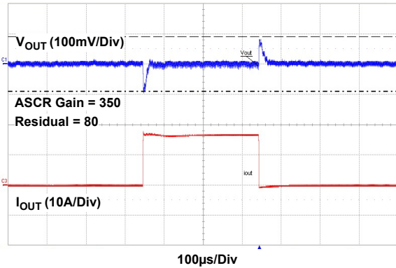
Figure 11. 12V_{IN} to 1V_{OUT} , f_{SW} = 615kHz , C_{OUT} = 4 \times 100\mu F Ceramic + 4 \times 470\mu F POSCAP
