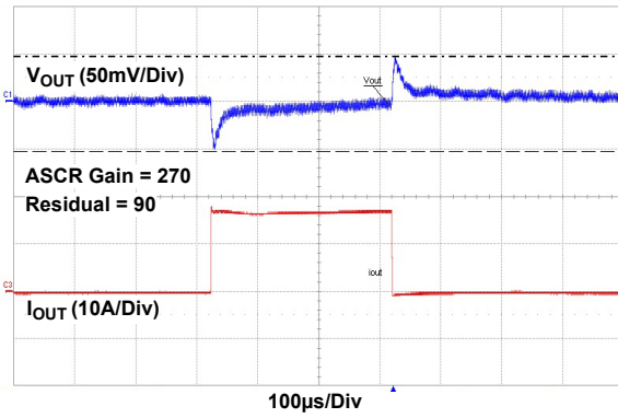
Figure 10. 5V_{IN} to 1.2V_{OUT} , f_{SW} = 364kHz , C_{OUT} = 10 \times 100\mu F Ceramic + 4 \times 470\mu F POSCAP
