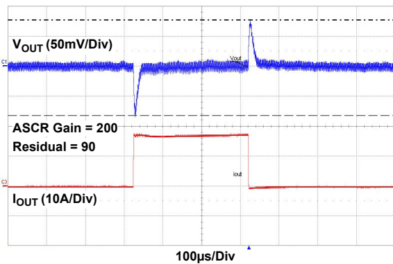
Figure 13. 12V_{IN} to 1.8V_{OUT} , f_{SW} = 471kHz , C_{OUT} = 6 \times 100\mu F Ceramic + 2 \times 470\mu F POSCAP
