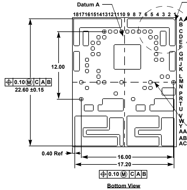
Bottom View
