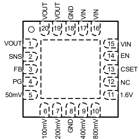
3.5×3.5 QFN Top View
