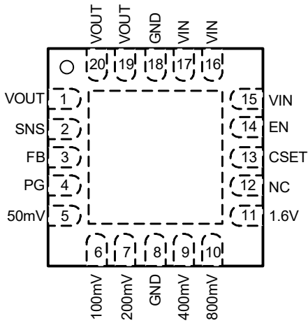
5×5 QFN Top View
