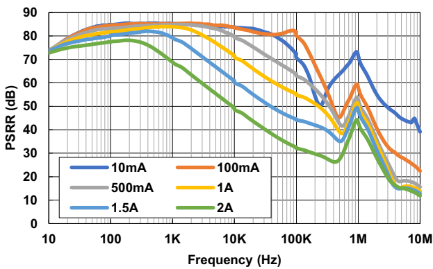
Figure 25. PSRR vs Frequency for Various I_{OUT} ( V_{IN} = 3.3V , V_{OUT} = 2.5V )
