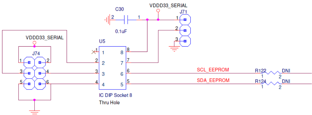
Figure 19. EEPROM Schematic
