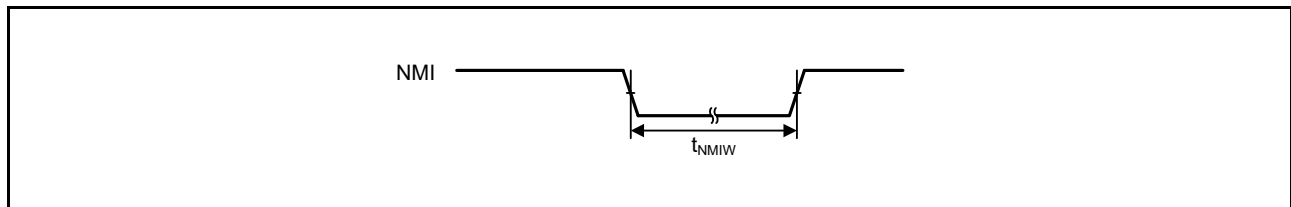
Figure 48.34 NMI interrupt input timing
