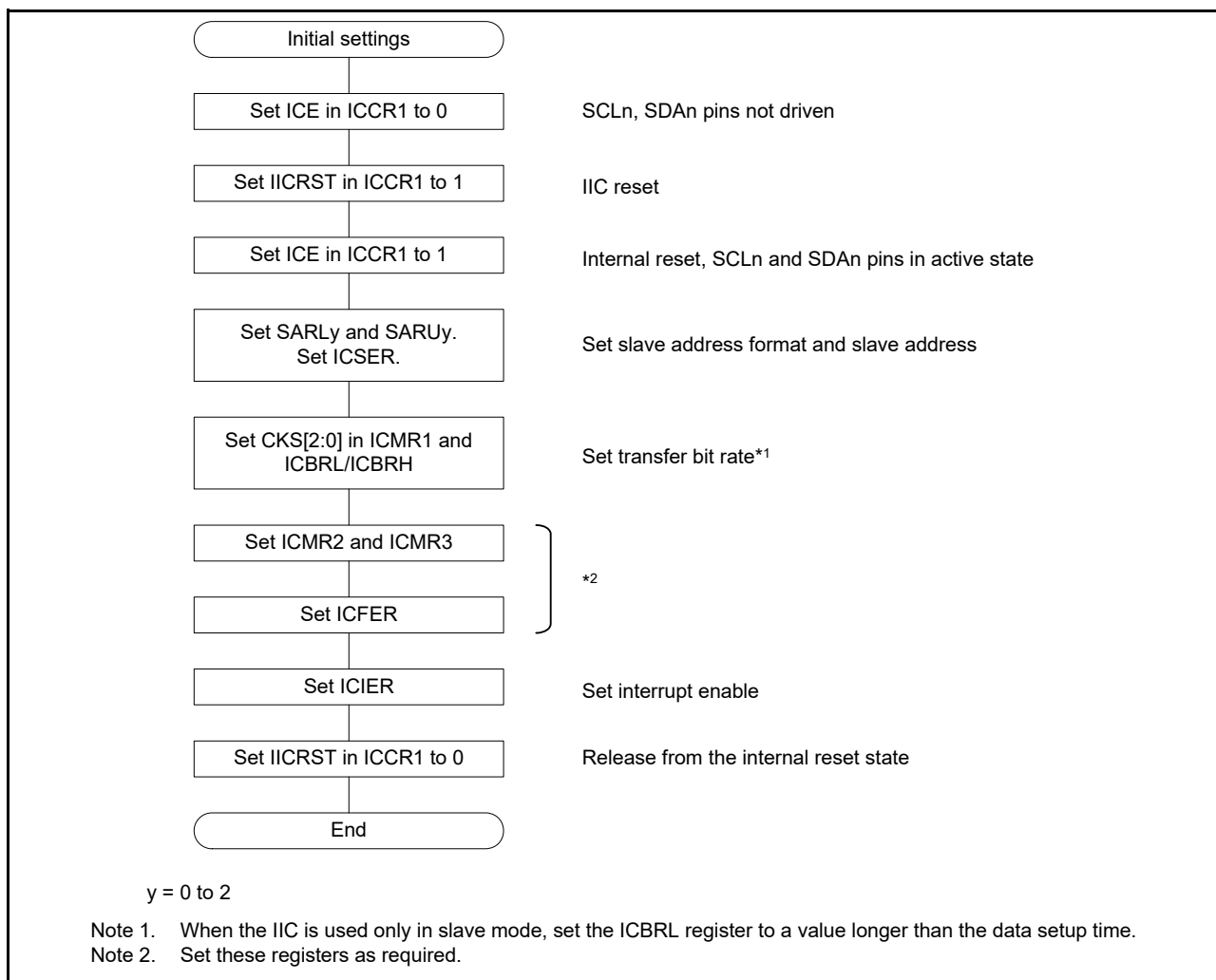
Figure 30.5 Example of IIC initialization flow
