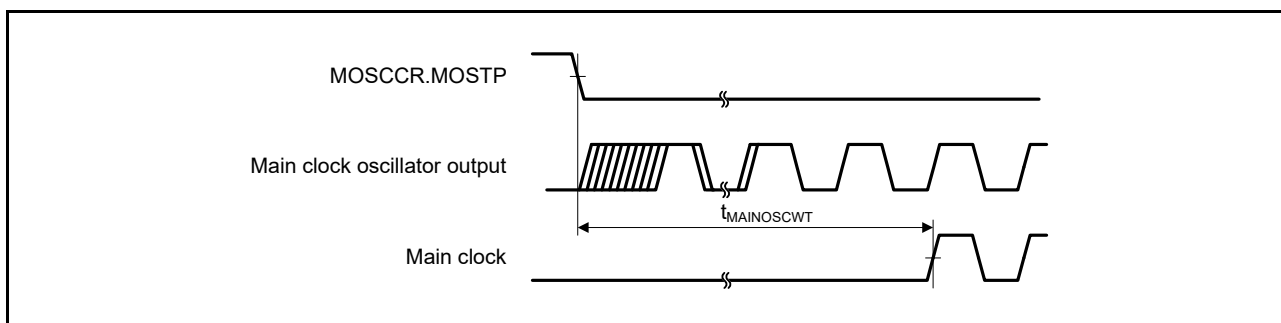
Figure 48.26 Main clock oscillation start timing
