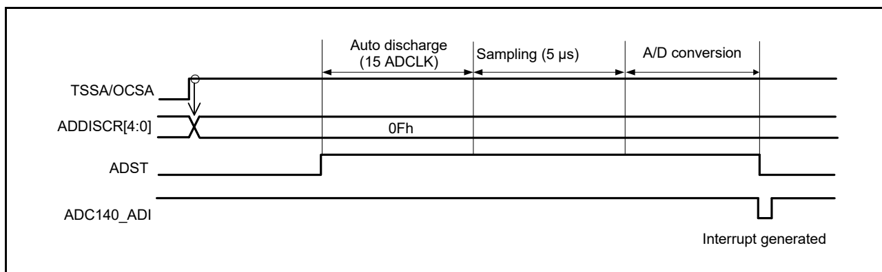
Figure 34.8 Example of basic operation in single scan mode when AN004 and temperature sensor output or internal reference voltage is selected
