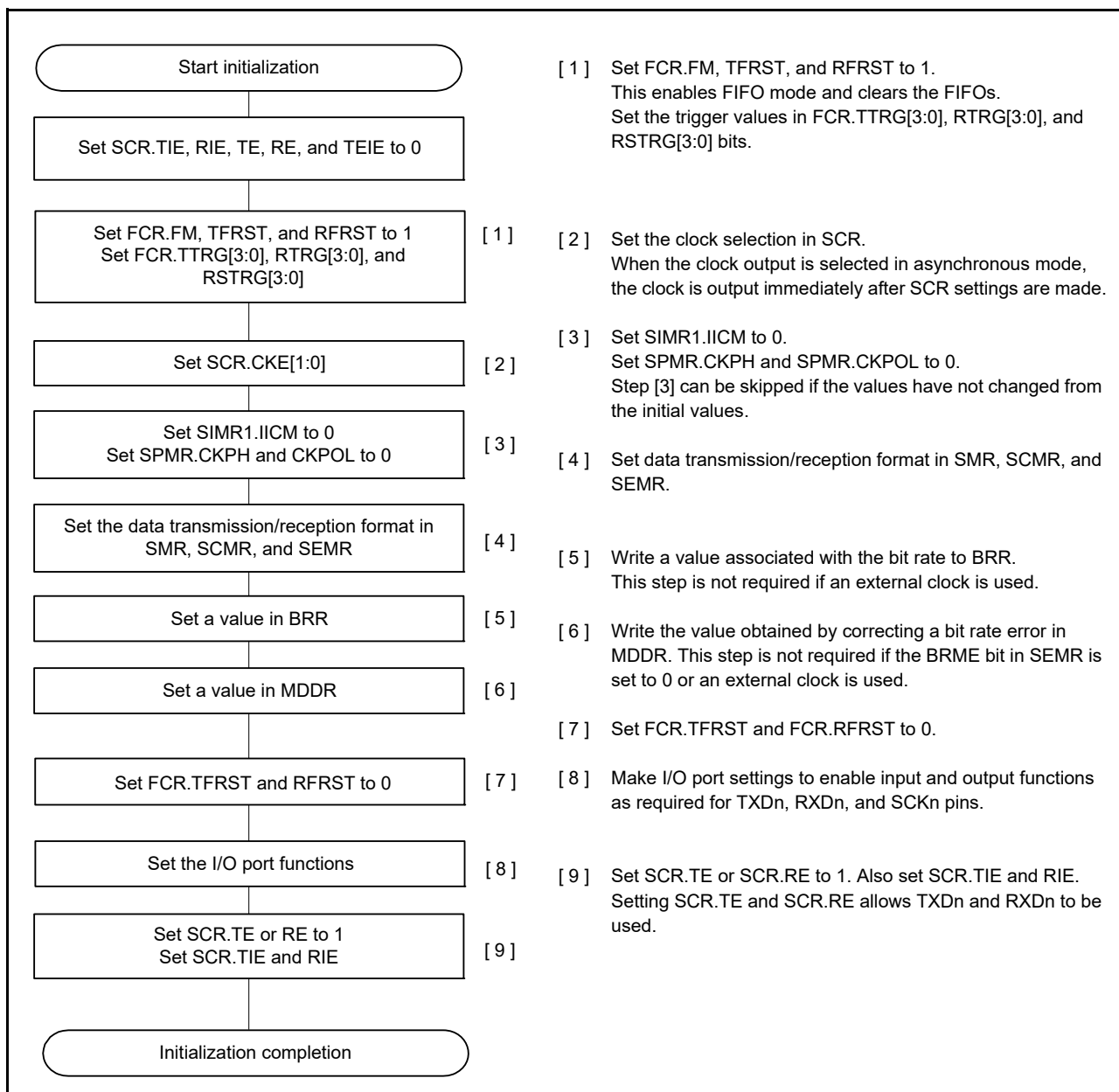
Figure 29.8 Example SCI initialization flow in synchronous mode with FIFO selected
