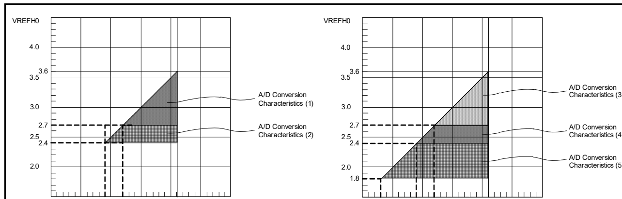
Figure 48.63 AVCC0 to VREFH0 voltage range
