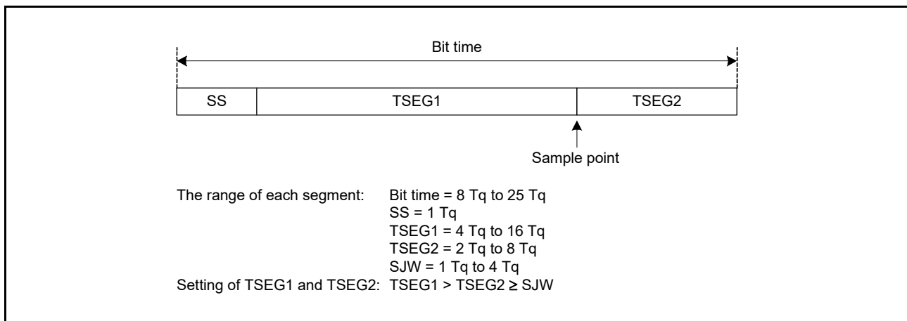
Figure 31.12 Bit timing
