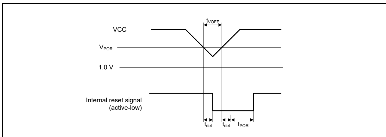
Figure 48.68 Voltage detection reset timing
