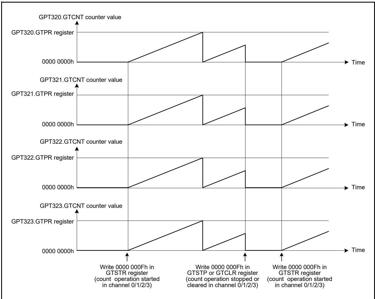
Figure 23.57 Example of a simultaneous start, stop, and clear by software with the same count cycle (GTPR register value)
