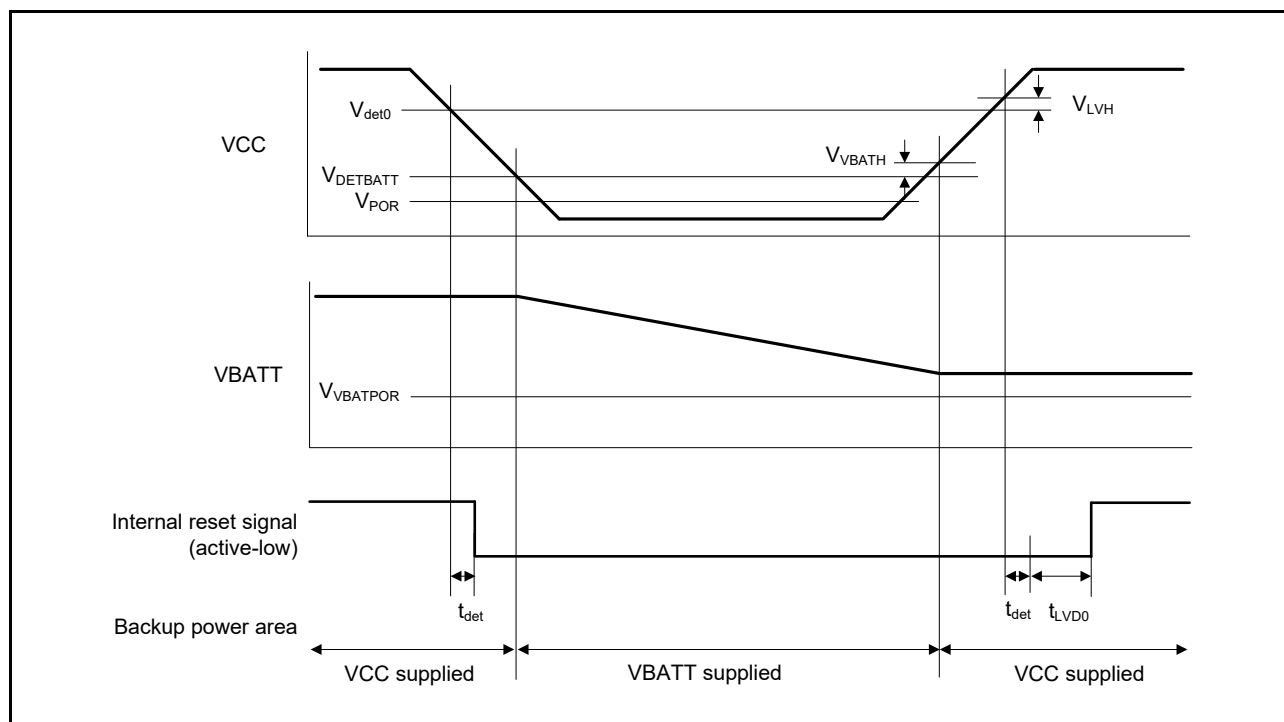
Figure 48.72 Power supply switching and LVD0 reset timing
