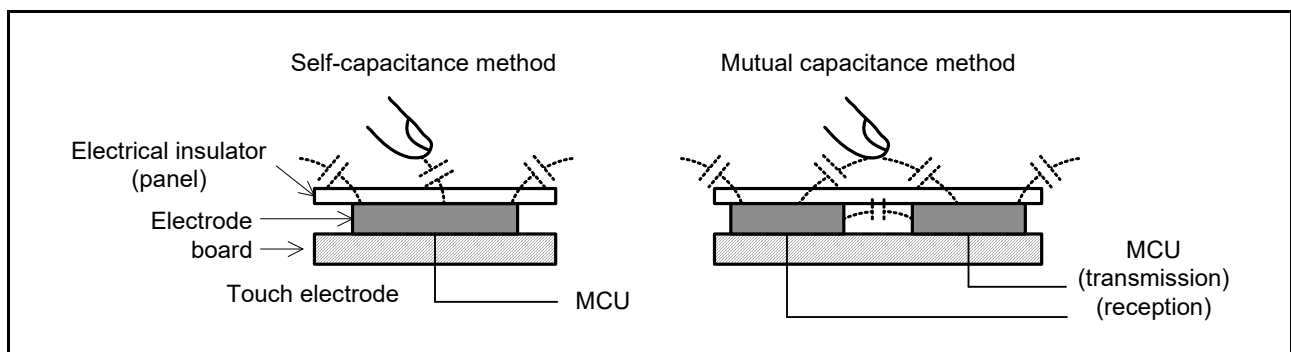
Figure 40.2 Self-capacitance and mutual-capacitance methods
