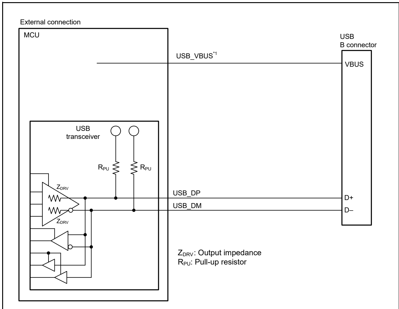
Figure 28.5 Example device connection in bus-powered state 2
