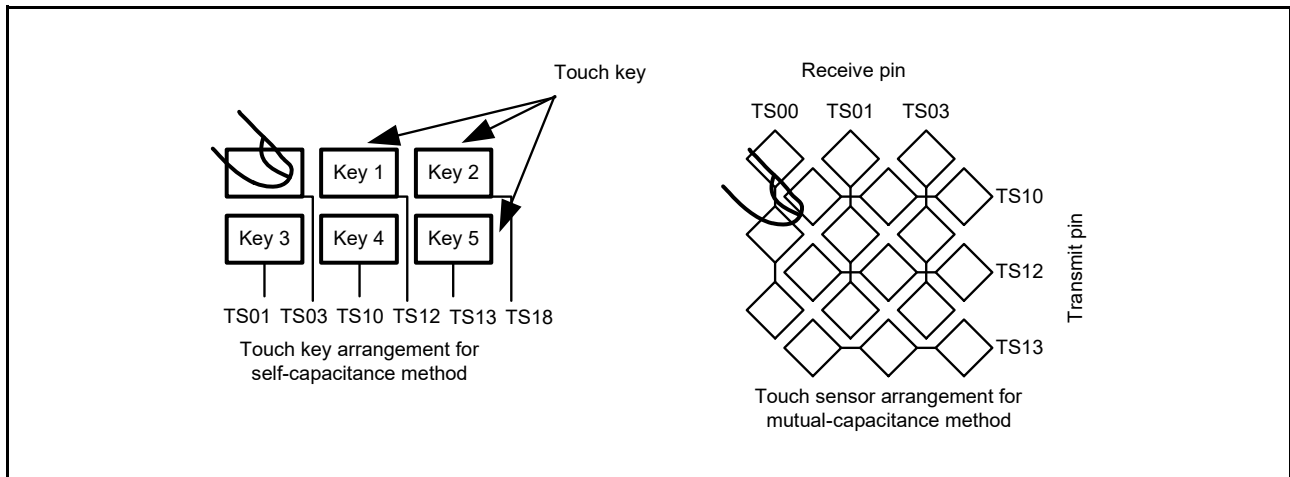
Figure 40.8 Overview of self-capacitance method and mutual-capacitance method
