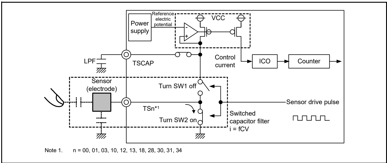
Figure 40.6 Discharging operation
