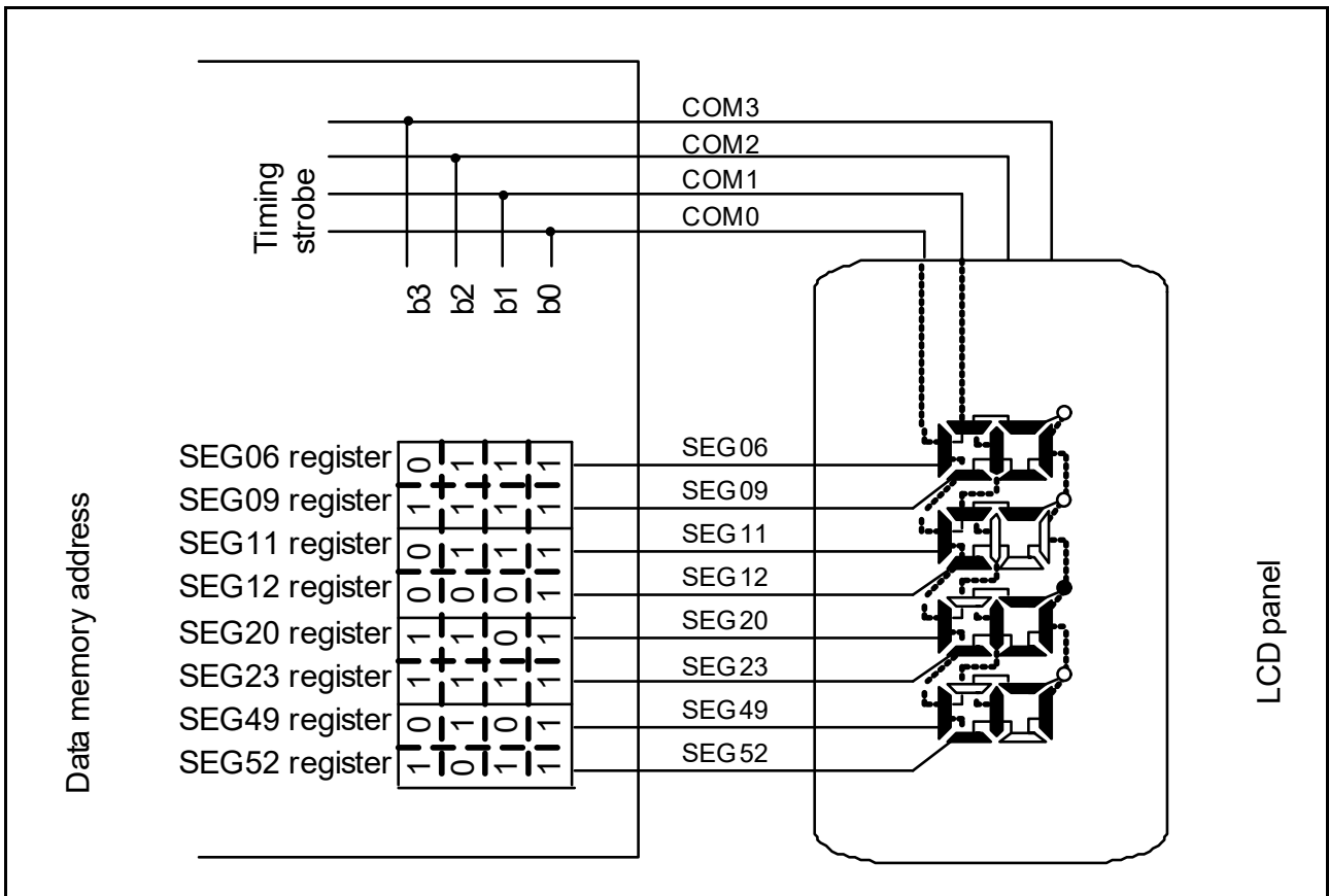
Figure 44.14 Example for connecting four-time-slice LCD panel
