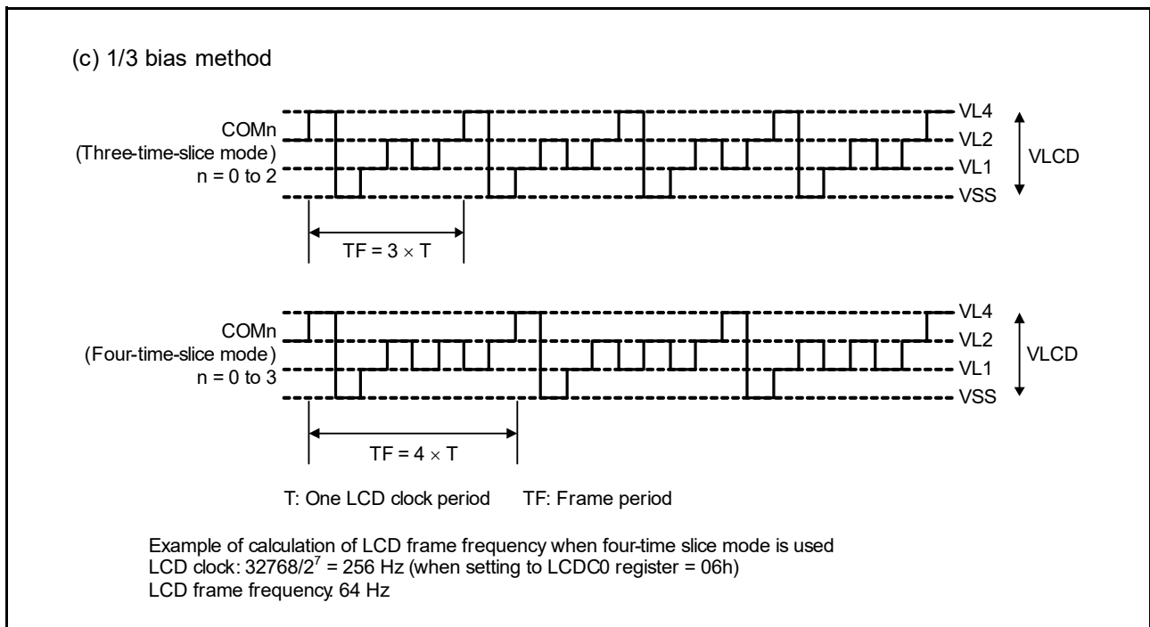
Figure 44.10 Common signal waveforms (2 of 2)
