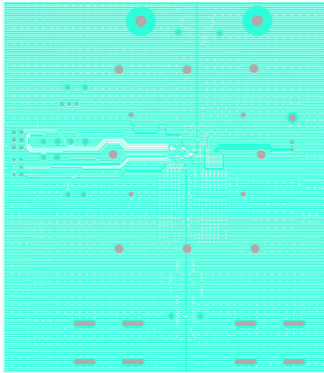
Figure 17. Inner Layer 3
