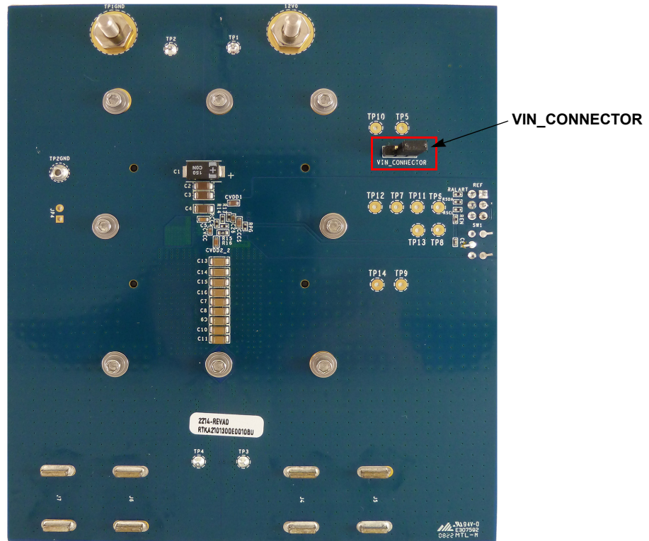
Figure 12. Bottom of Board
