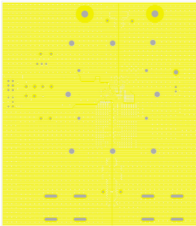
Figure 18. Inner Layer 4
