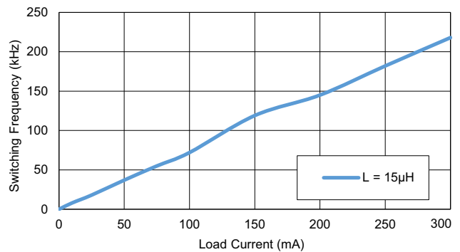
Figure 3. Switching Frequency (V IN : 24V) vs. Load Current
