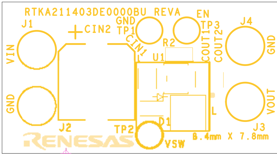
Figure 6. Silkscreen Top
