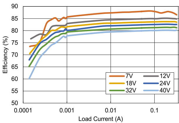
Figure 20. Efficiency
