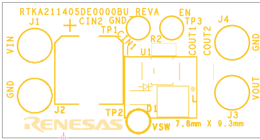
Figure 6. Silkscreen Top
