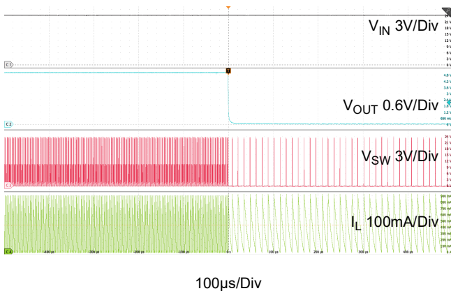
Figure 14. Short-Circuit
