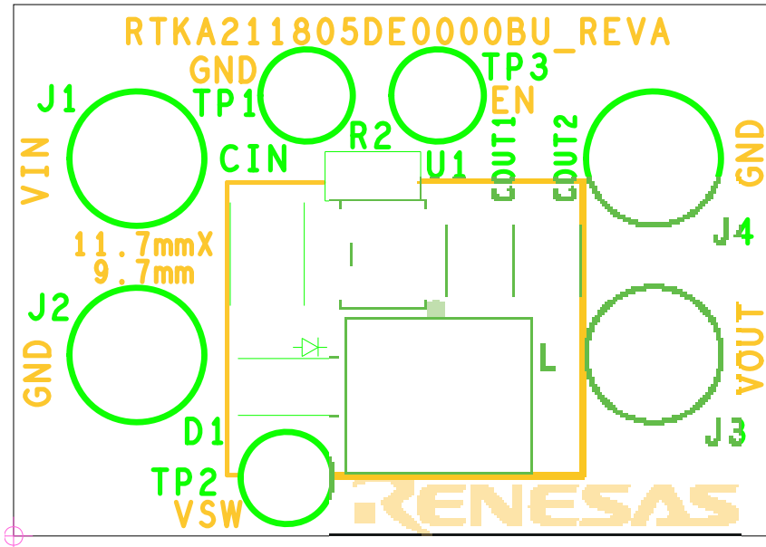
Figure 6. Silkscreen Top
