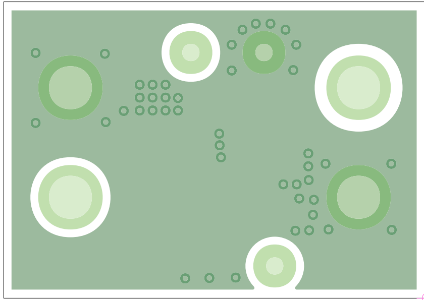
Figure 8. Bottom Layer
