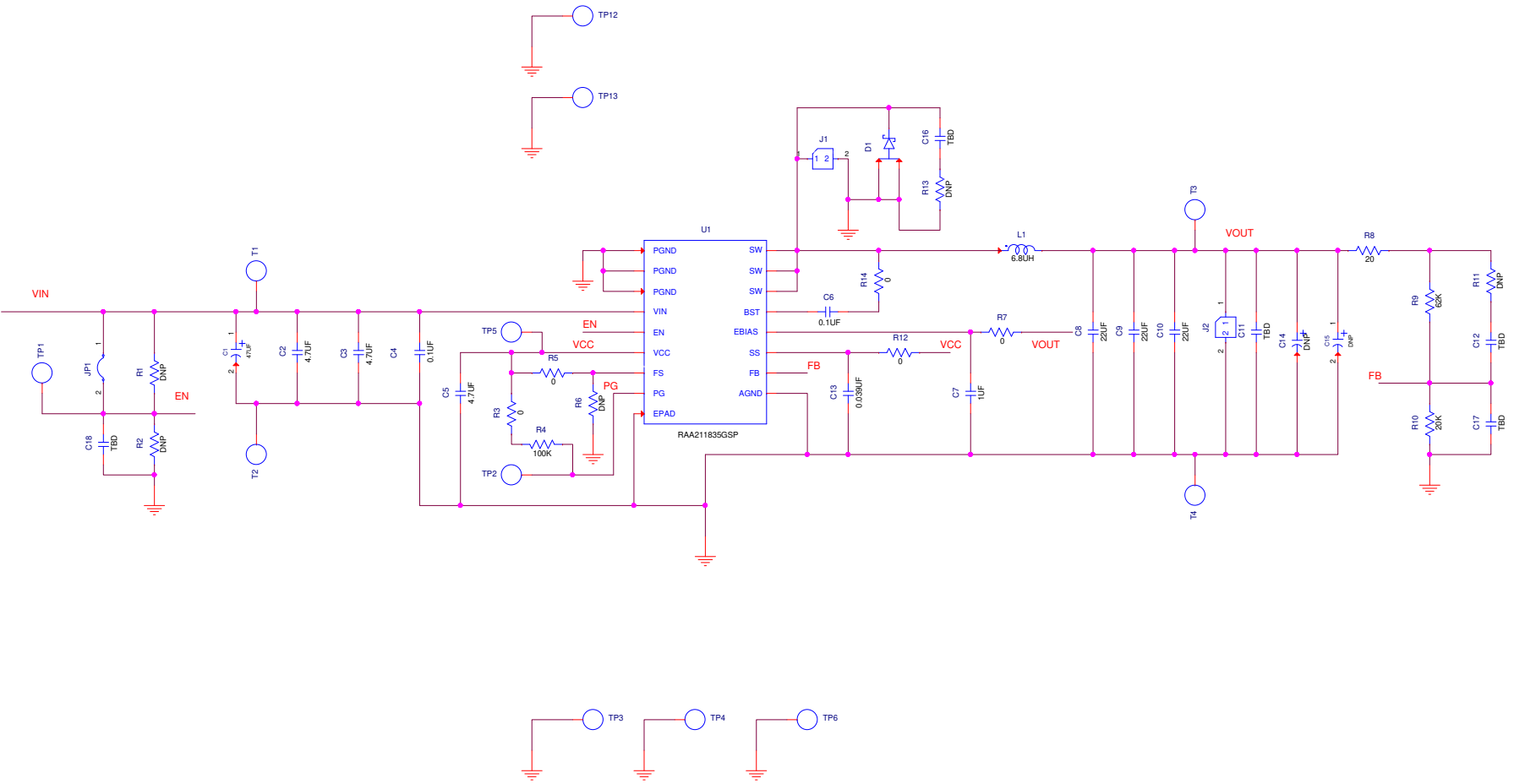
Figure 4. RTKA211835DE0010BU Schematic
