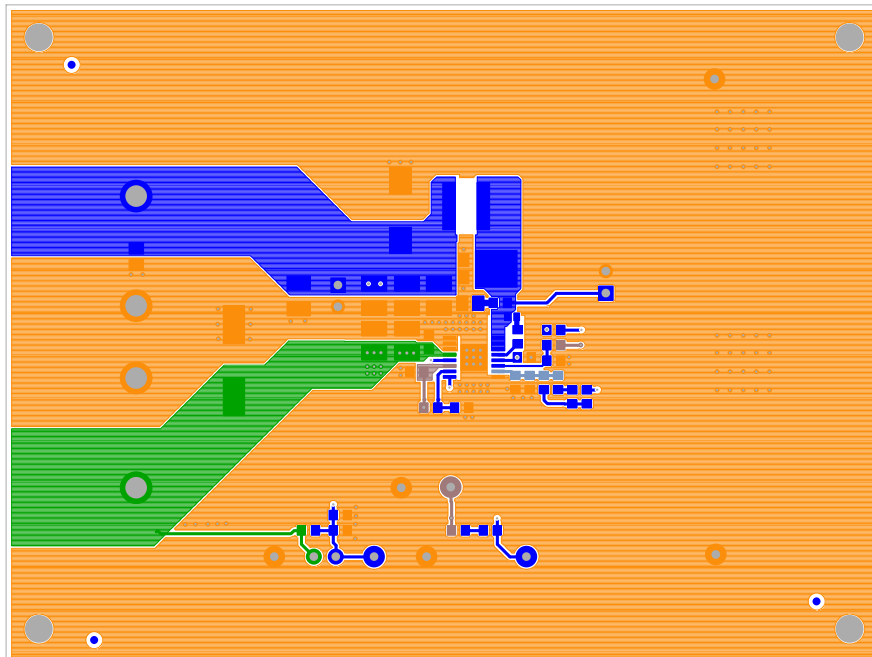
Figure 6. Top Layer
