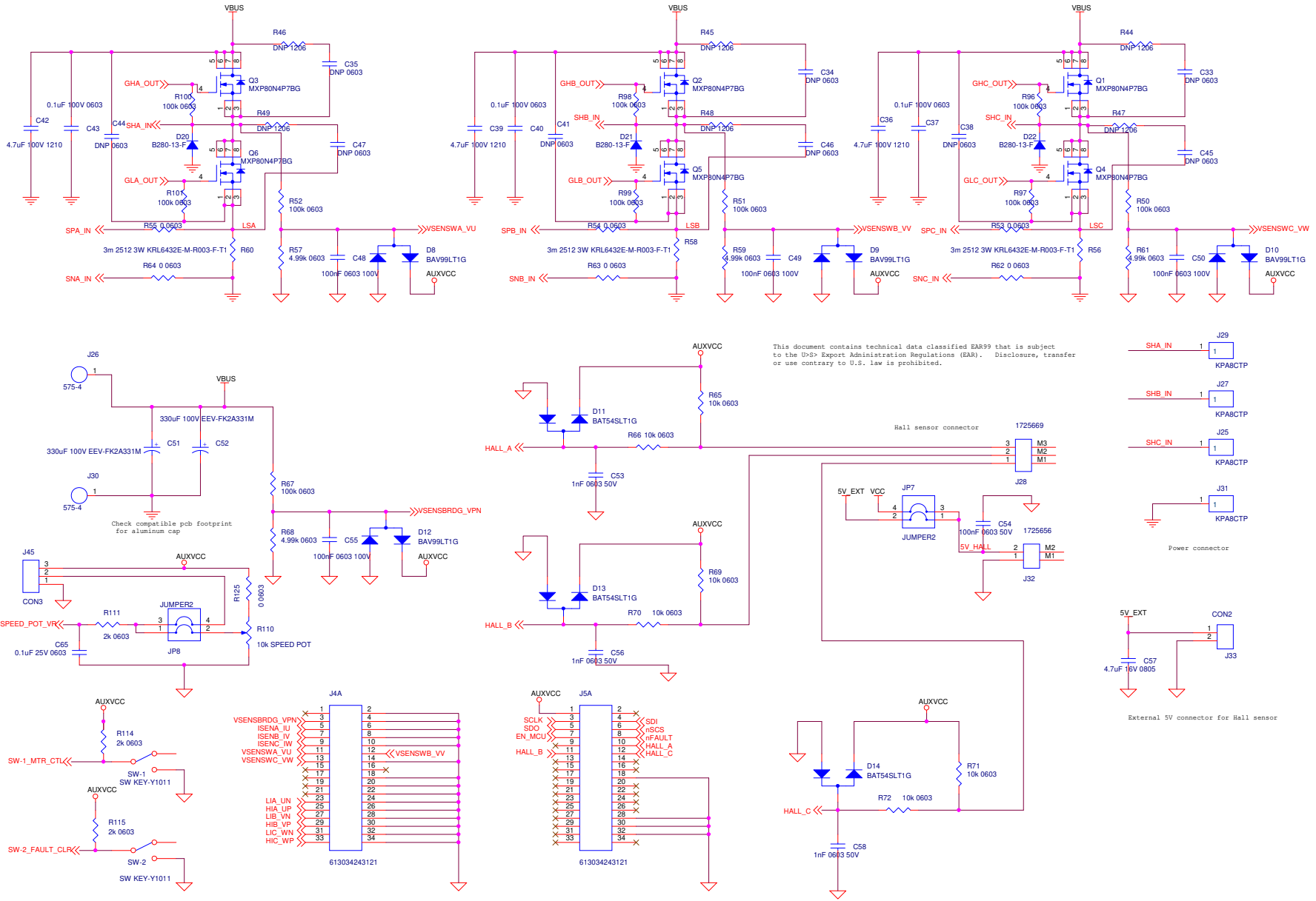
Figure 5. RTKA227063DE0000BU Evaluation Board Schematic (Page 2)
