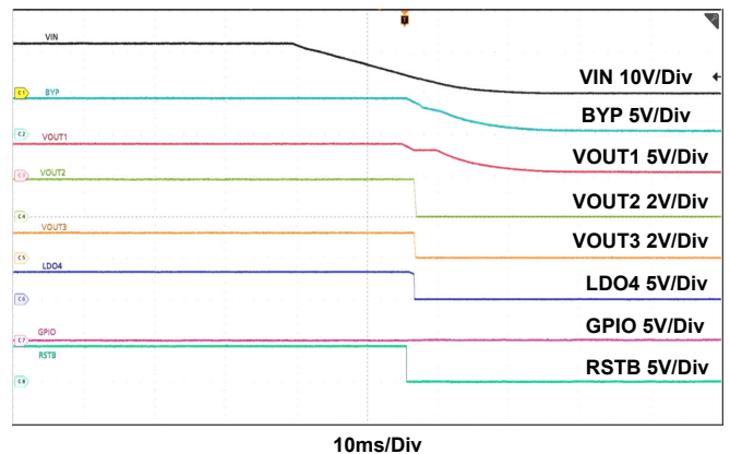
Figure 37. Shutdown using V_{IN} ramp, EN connected to V_{IN}
