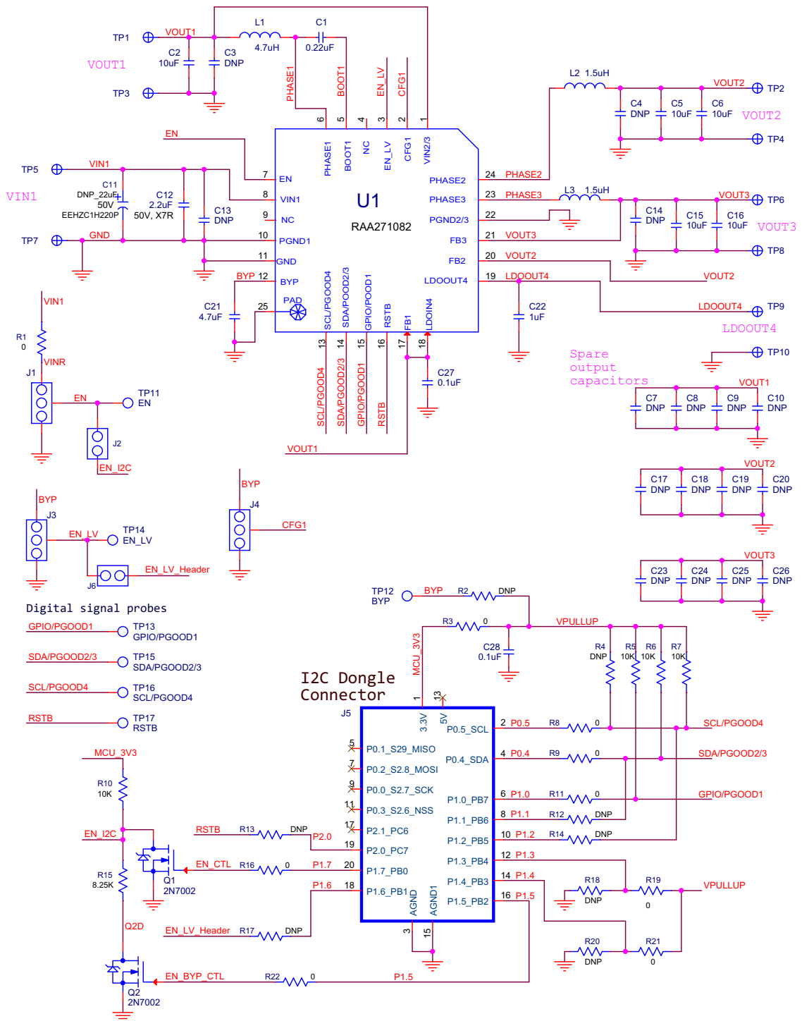
Figure 19. RTKA271082DE000BU Schematic
