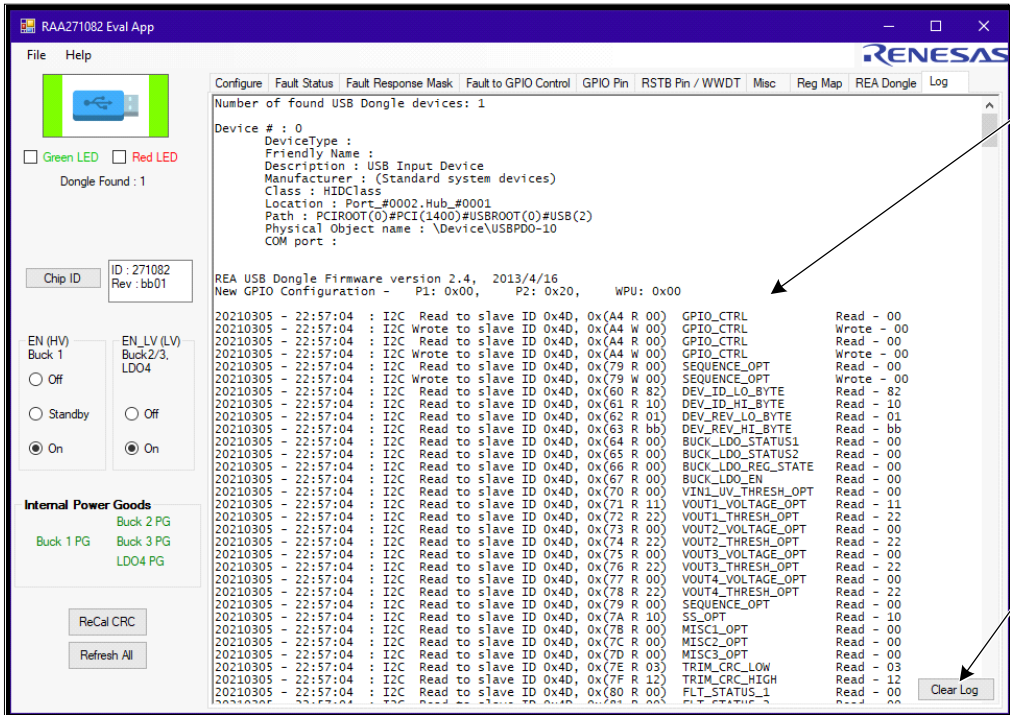
Figure 15. Log Tab with Labels
