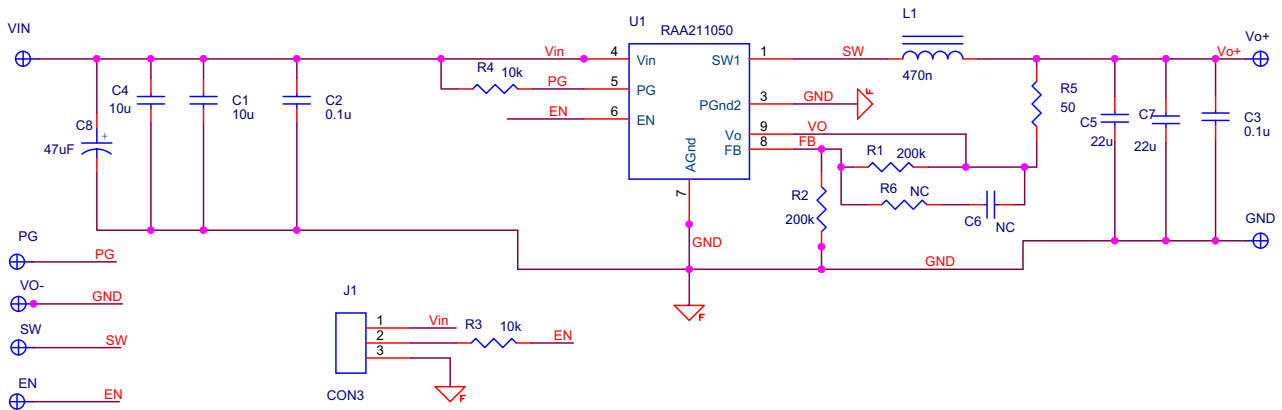
Figure 3. RTKA808015DE0000BU Schematic
