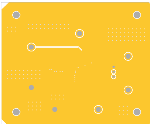
Figure 8. Bottom Layer
