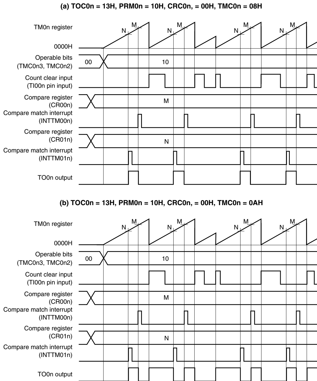
Figure 7-28. Timing Example of Clear & Start Mode Entered by TIO0n Pin Valid Edge Input (CR00n: Compare Register, CR01n: Compare Register)
