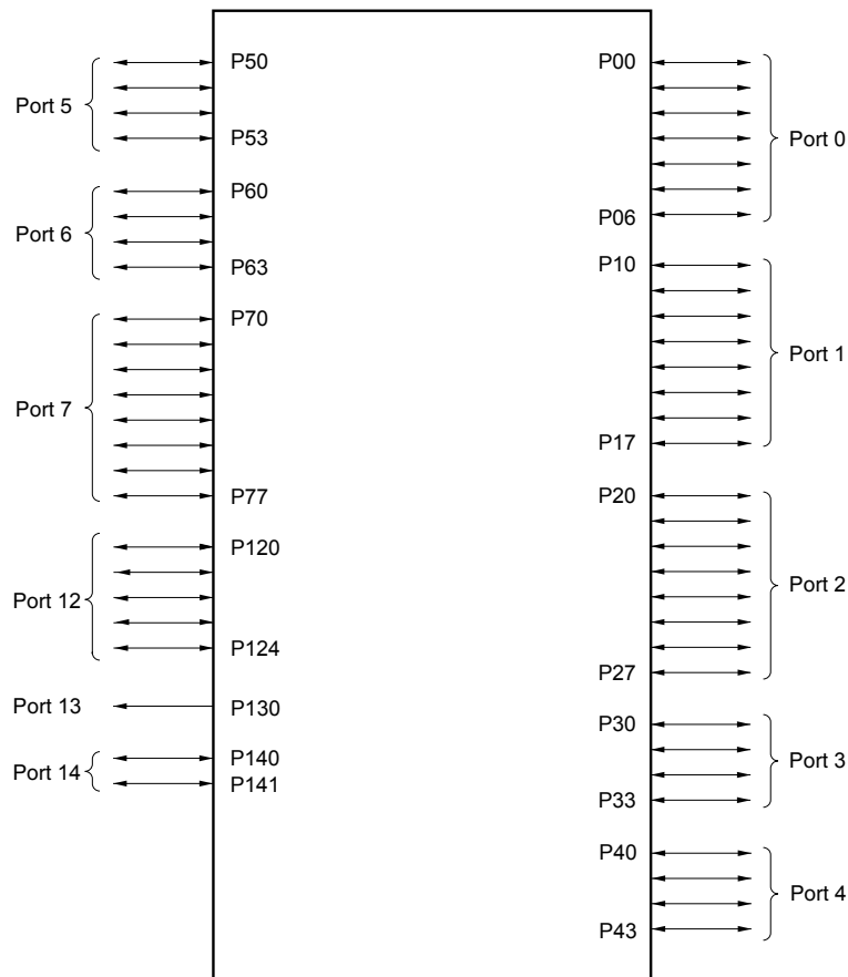
Figure 5-1. Port Types
