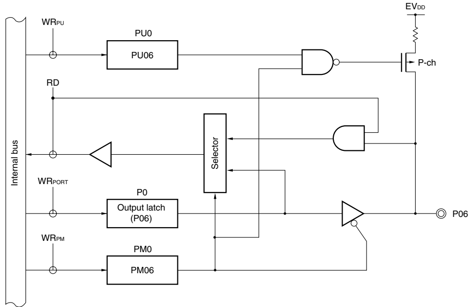
Figure 5-7. Block Diagram of P06
