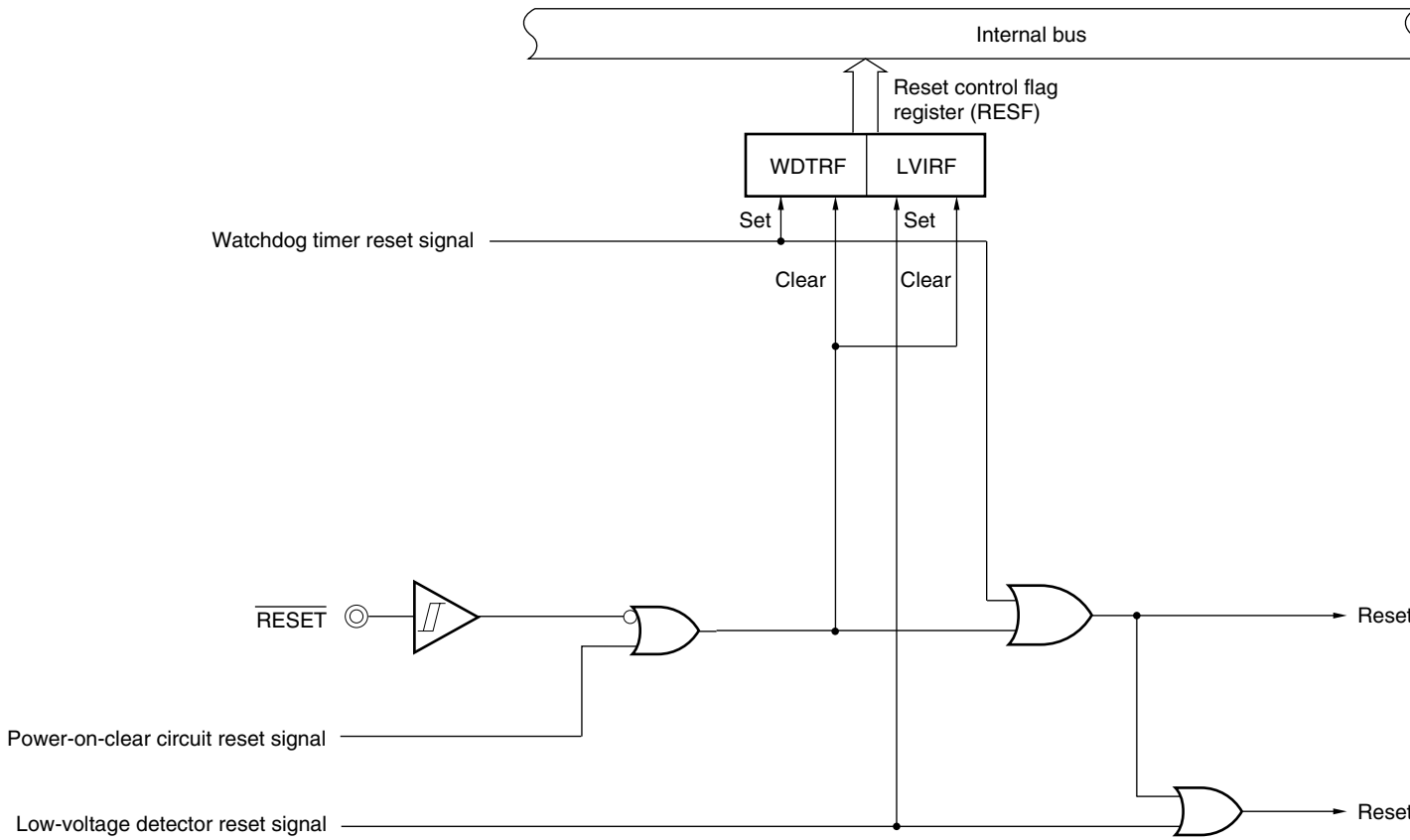
Figure 22-1. Block Diagram of Reset Function
