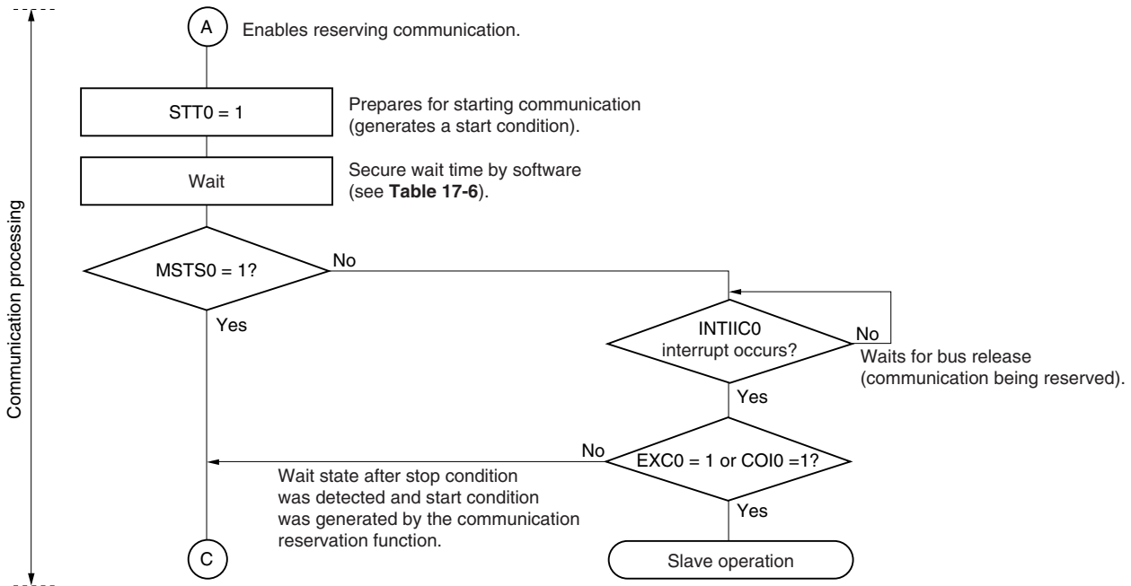
Figure 17-24. Master Operation Flowchart (Multi-Master System) (2/3)
