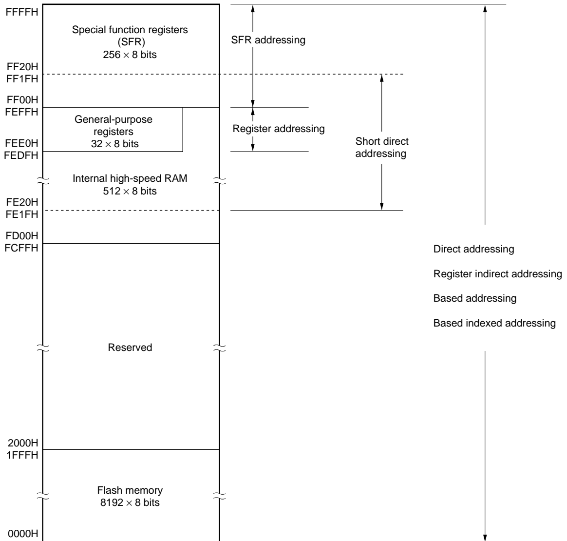
Figure 3-5. Correspondence Between Data Memory and Addressing ( \mu PD78F0741, 78F0743, 78F0745, 78F0751, 78F0753, 78F0755)
