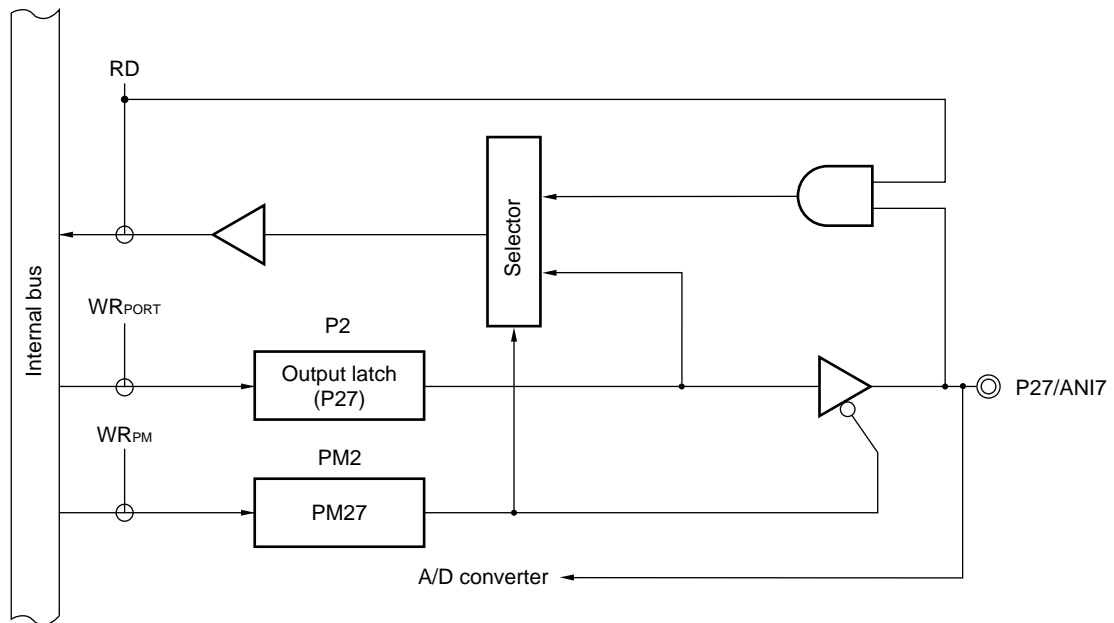
Figure 4-11. Block Diagram of P27
