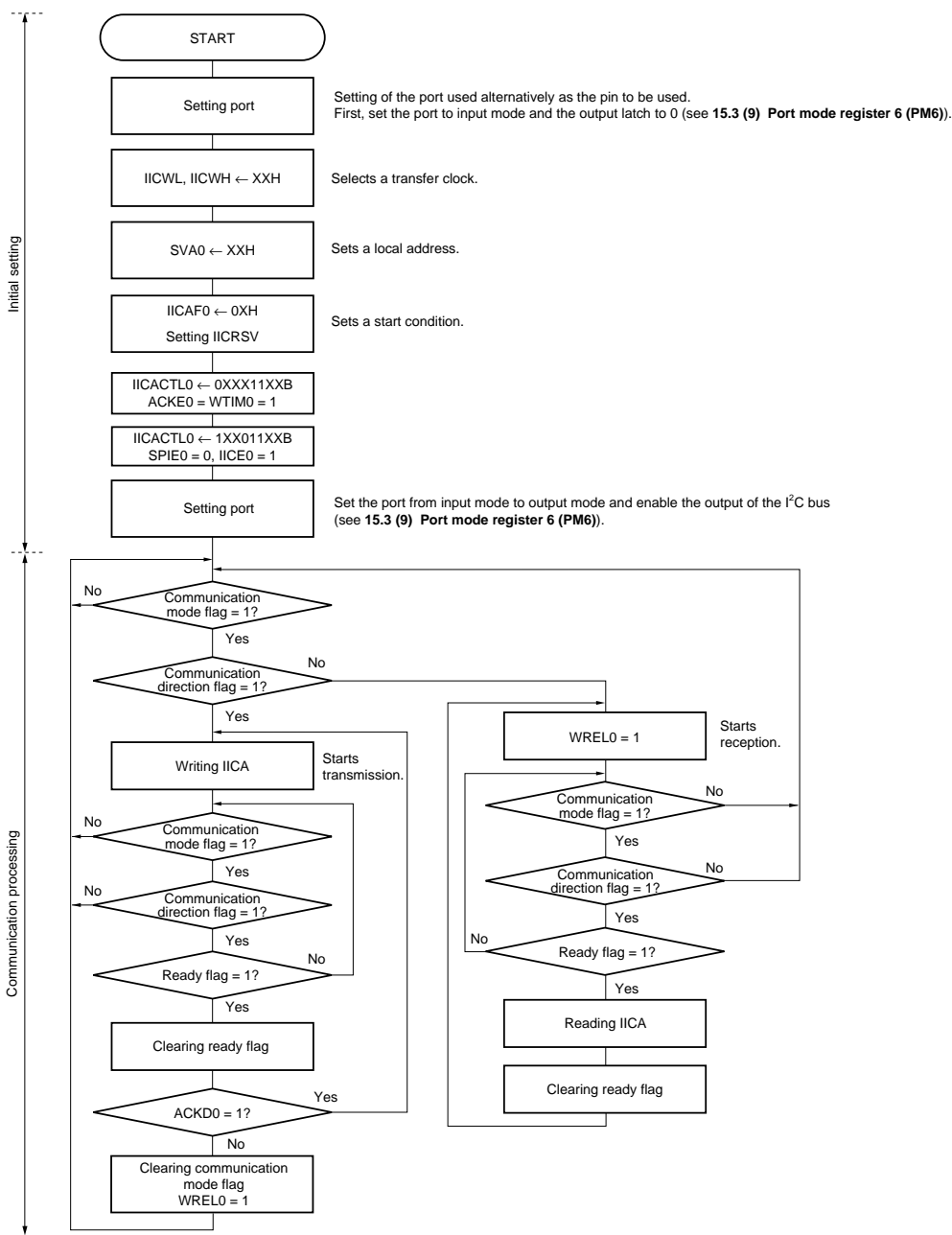
Figure 15-31. Slave Operation Flowchart (1)
