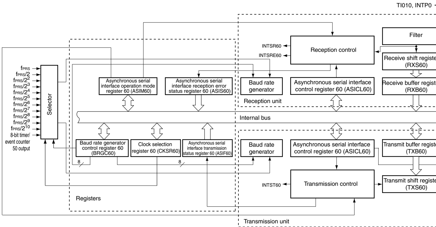
Figure 13-5. Block Diagram of Serial Interface UART60
