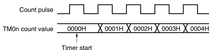
Figure 6-44. Start Timing of TM0n Count
