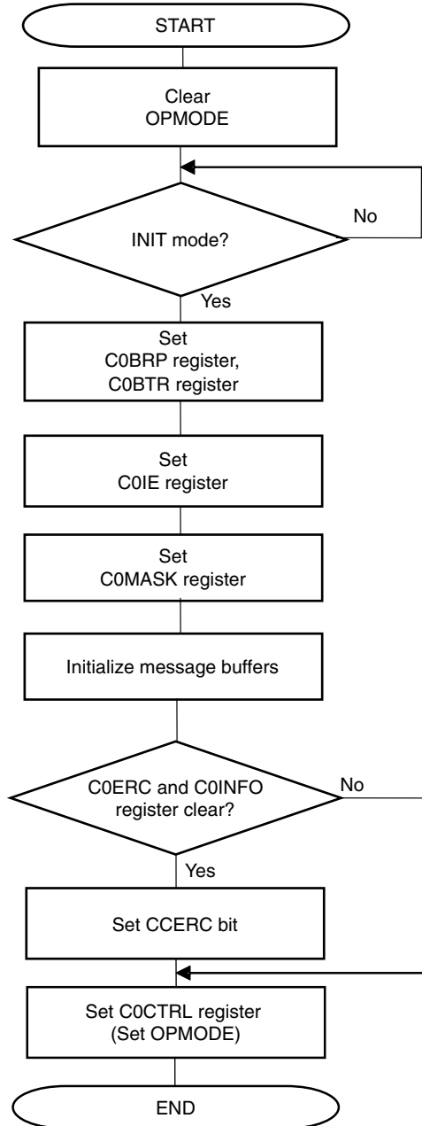
Figure 15-38. Re-initialization
