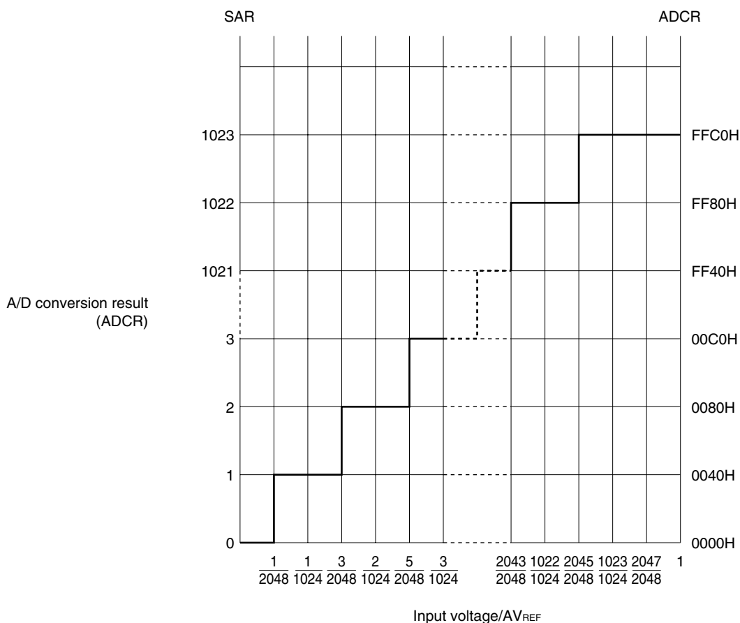
Figure 12-13. Relationship Between Analog Input Voltage and A/D Conversion Result
