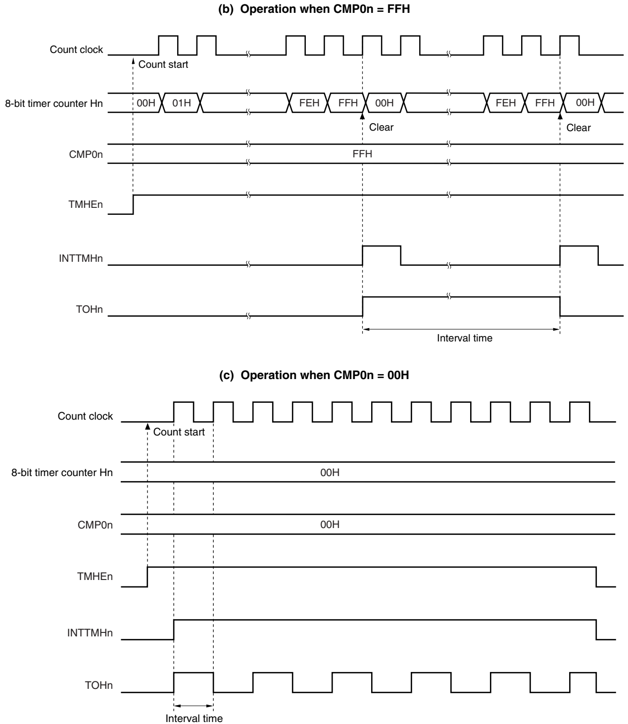
Figure 8-10. Timing of Interval Timer/Square-Wave Output Operation (2/2)
