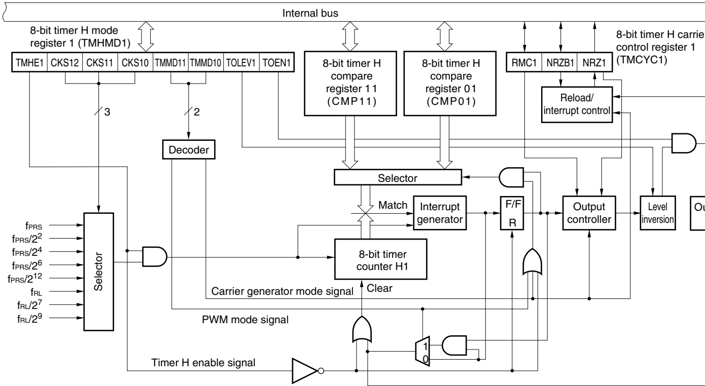
Figure 8-2. Block Diagram of 8-Bit Timer H1
