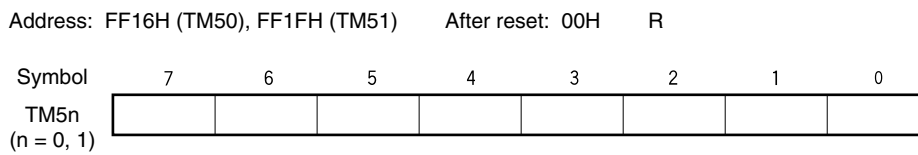
Figure 7-3. Format of 8-Bit Timer Counter 5n (TM5n)
