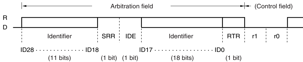
Figure 15-7. Arbitration Field (in Extended Format Mode)
