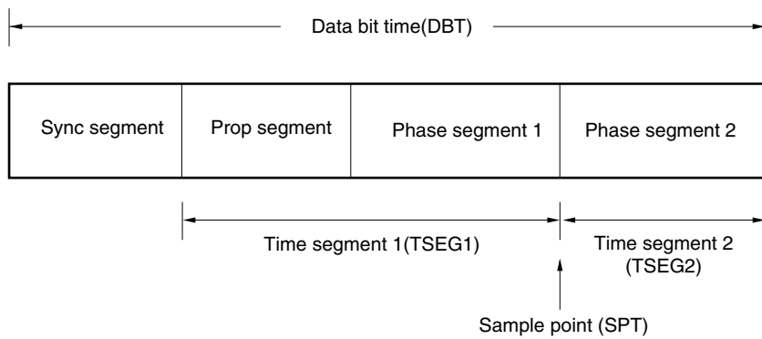
Figure 15-18. Segment Setting
