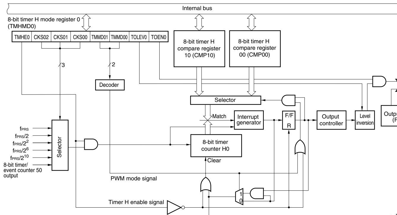
Figure 8-1. Block Diagram of 8-Bit Timer H0
