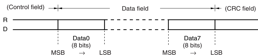
Figure 15-9. Data Field
