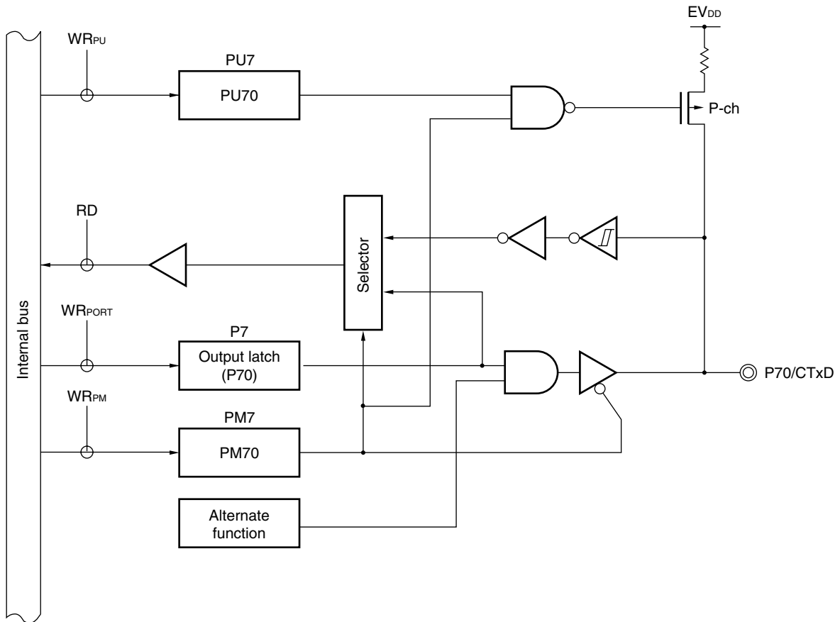
Figure 4-12. Block Diagram of P70
