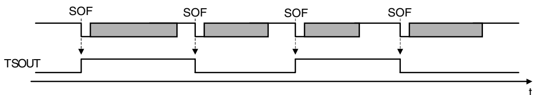
Figure 15-35. Timing Diagram of Capture Signal TSOUT
