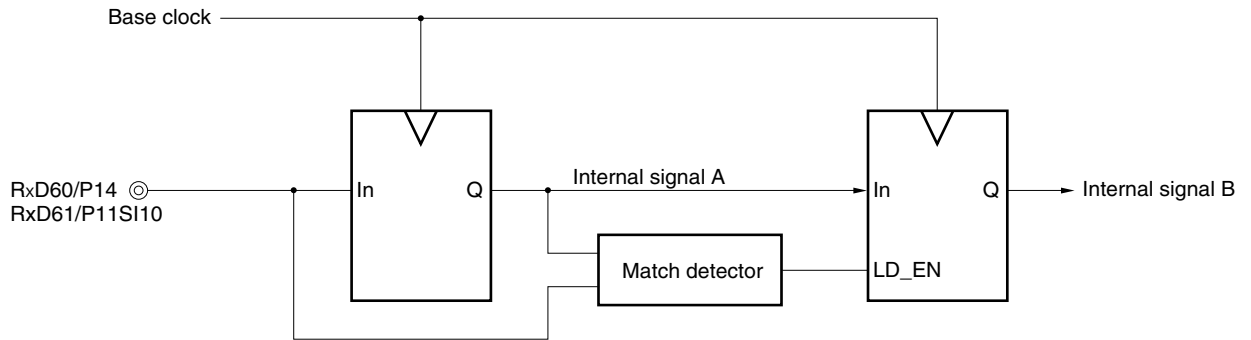
Figure 13-29. Noise Filter Circuit
