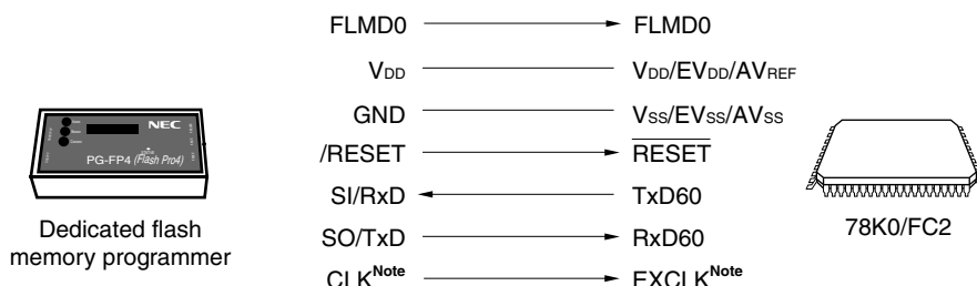
Figure 23-9. Communication with Dedicated Flash Memory Programmer (UART60)
