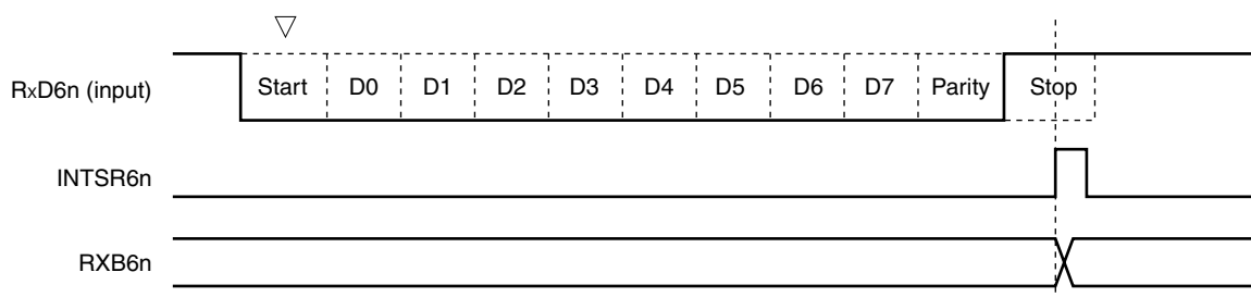
Figure 13-27. Reception Completion Interrupt Request Timing
