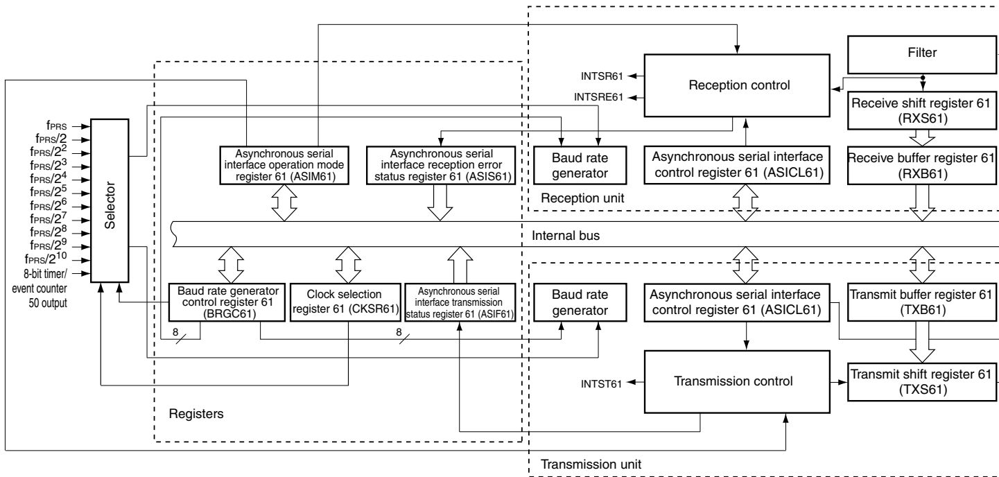
Figure 13-6. Block Diagram of Serial Interface UART61
