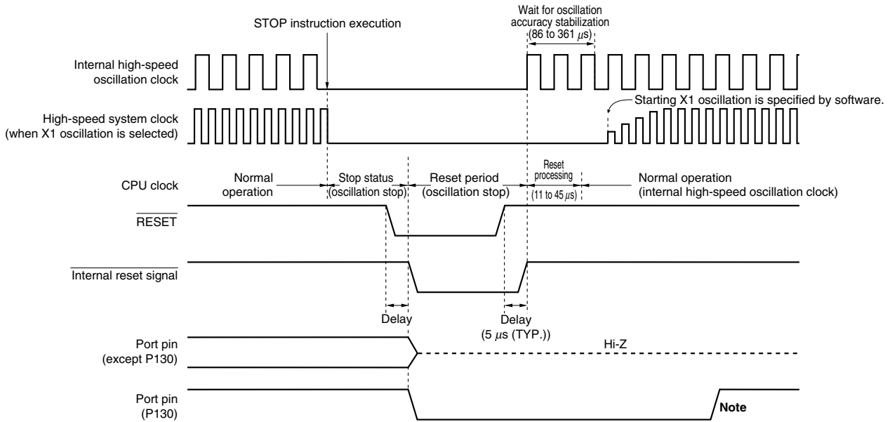
Figure 18-4. Timing of Reset in STOP Mode by \overline{\text{RESET}} Input
