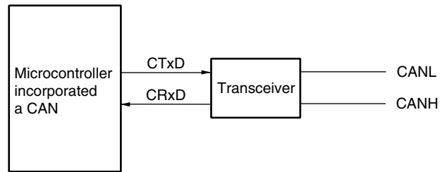
Figure 15-22. Connection to CAN Bus
