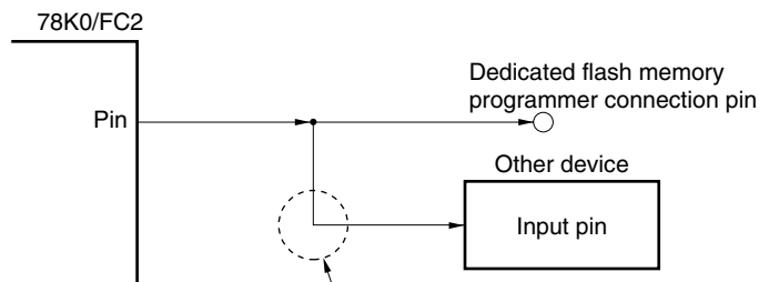
Figure 23-12. Malfunction of Other Device
