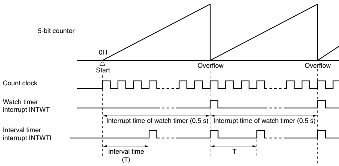
Figure 9-3. Operation Timing of Watch Timer/Interval Timer
