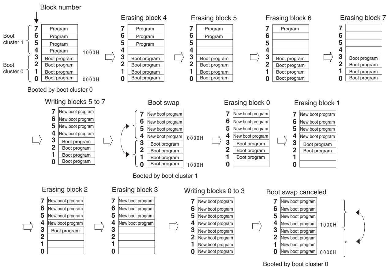
Figure 23-23. Example of Executing Boot Swapping
