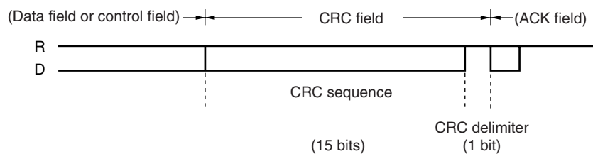
Figure 15-10. CRC Field
