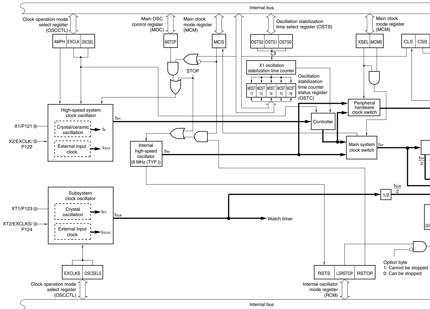
Figure 5-1. Block Diagram of Clock Generator
