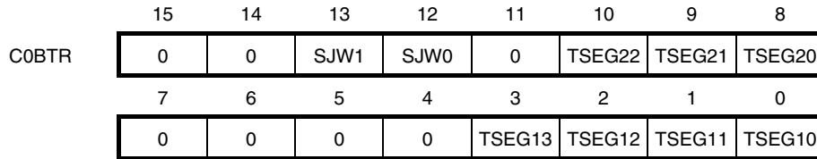
Figure 15-26. Data Bit Time
