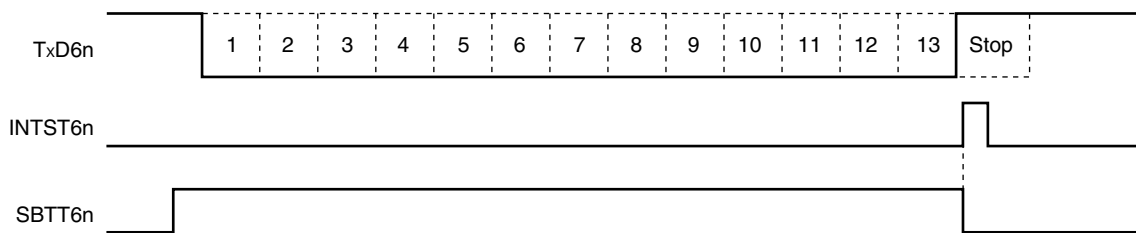
Figure 13-30. SBF Transmission
