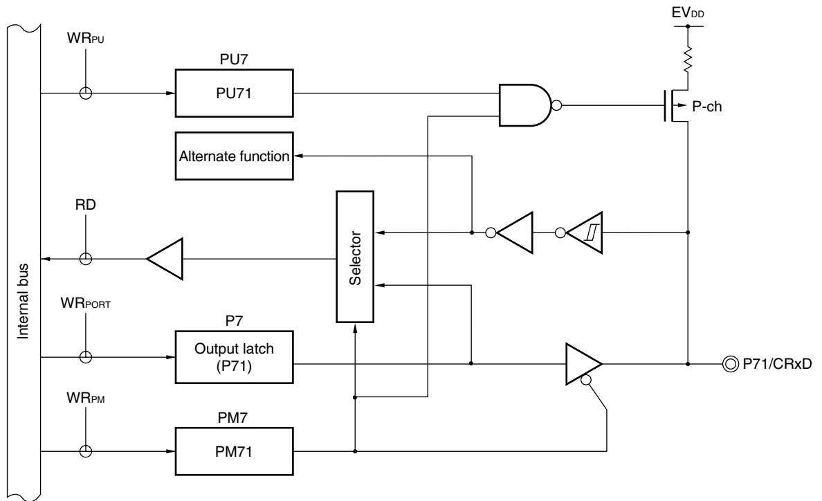
Figure 4-13. Block Diagram of P71
