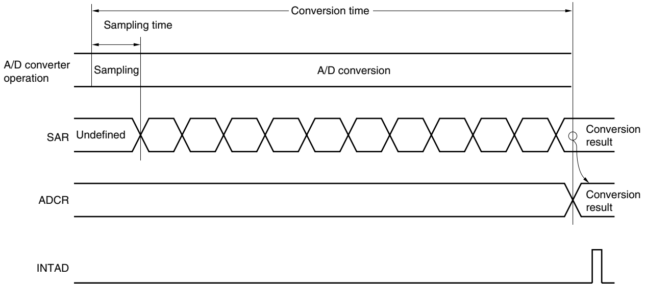
Figure 12-12. Basic Operation of A/D Converter
