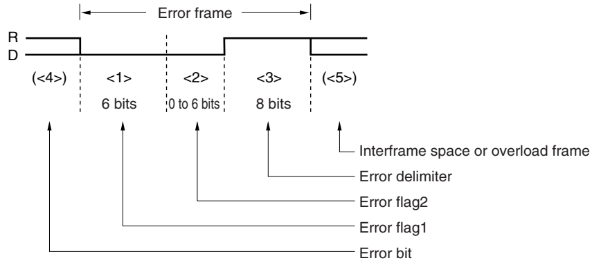
Figure 15-15. Error Frame
