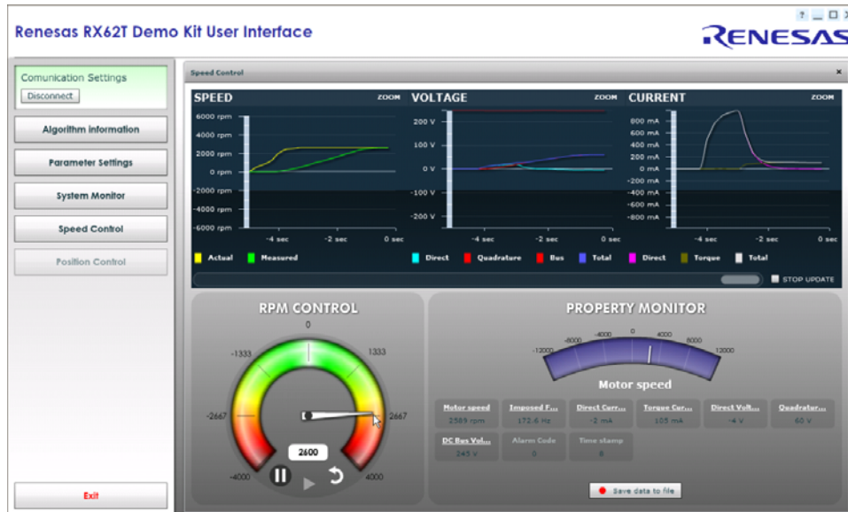
Figure 12 PC-GUI Step 11
