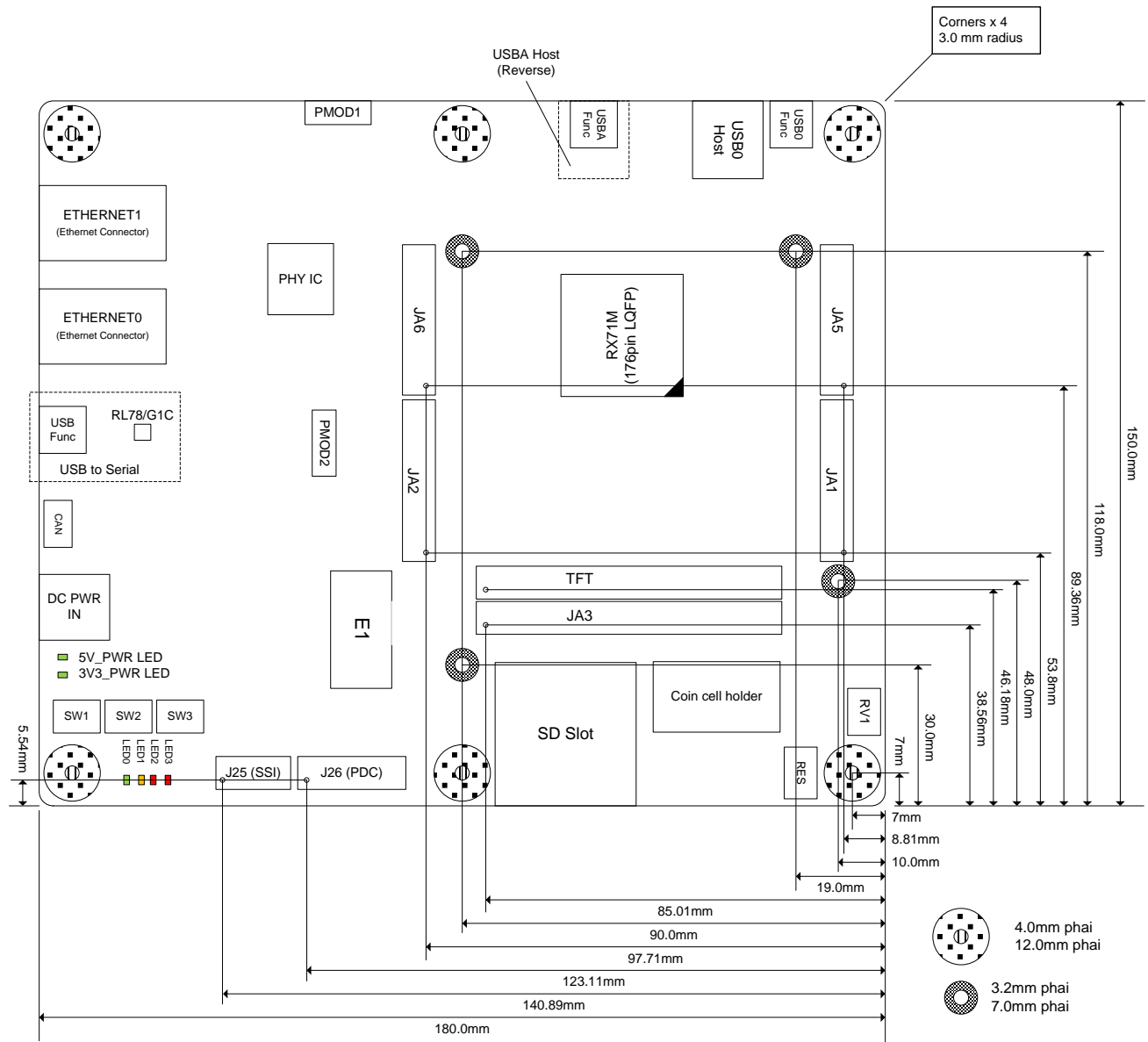
Figure 3-2: Board Dimensions
