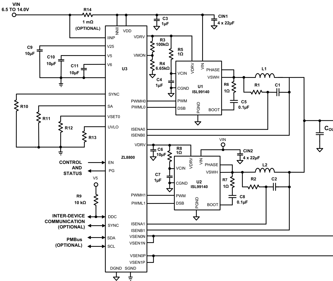
FIGURE 4. TWO PHASE SCHEMATIC
