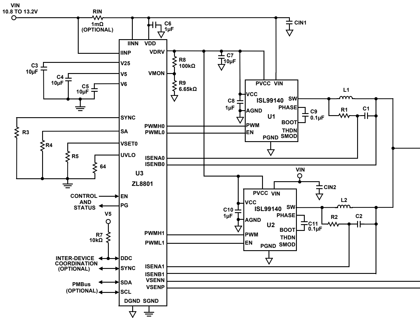
FIGURE 3. ZL8801 SCHEMATIC
