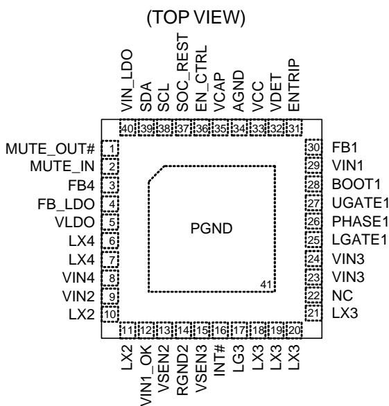
WQFN-40L 5x5
