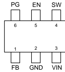
SOT-563 (FC) (RT5760A/B)
