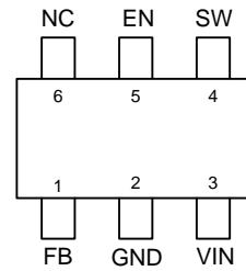
SOT-563 (FC) (RT5760C/D)
