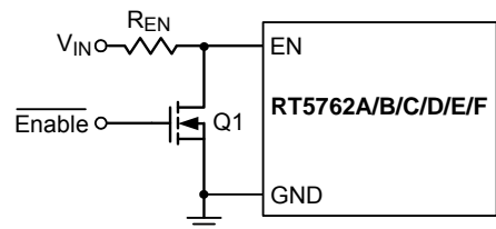
Figure 7. Logic Control for the EN Pin
