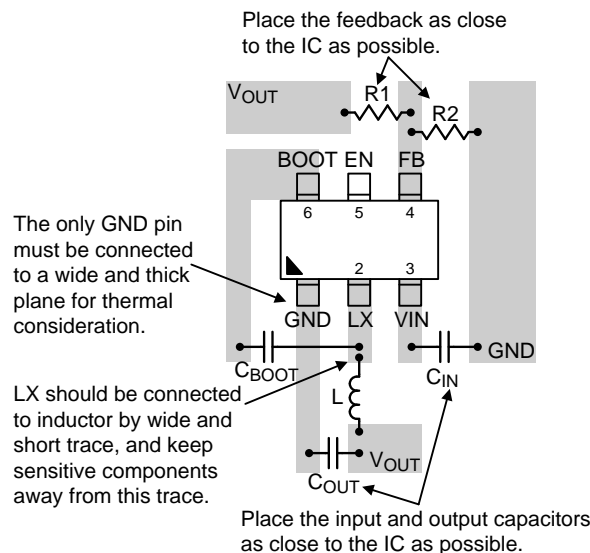
Figure 8. PCB Layout Guide
