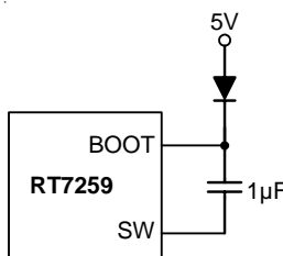
Figure 2. External Bootstrap Diode
