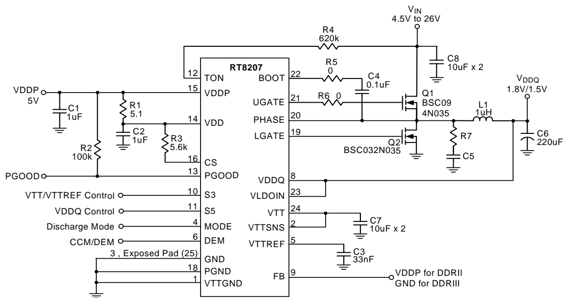
Figure 2. Fixed Voltage Regulator
