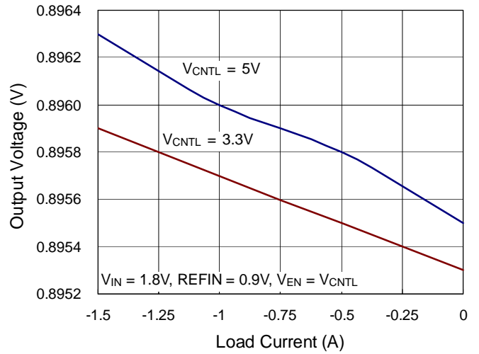
DDR II Output Voltage vs. Load Current
