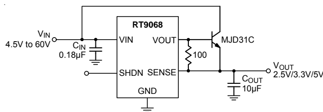
Figure 3. RT9068-25/33/50 External Transistor Application
