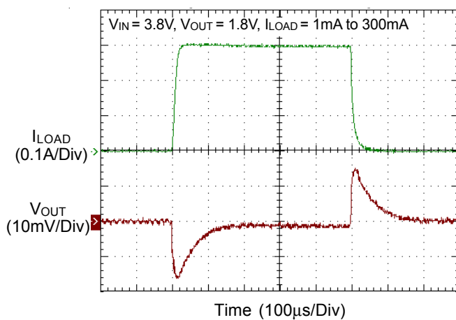
Load Transient
