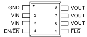
SOP-8/MSOP-8
