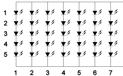
LED Diagram Circ
