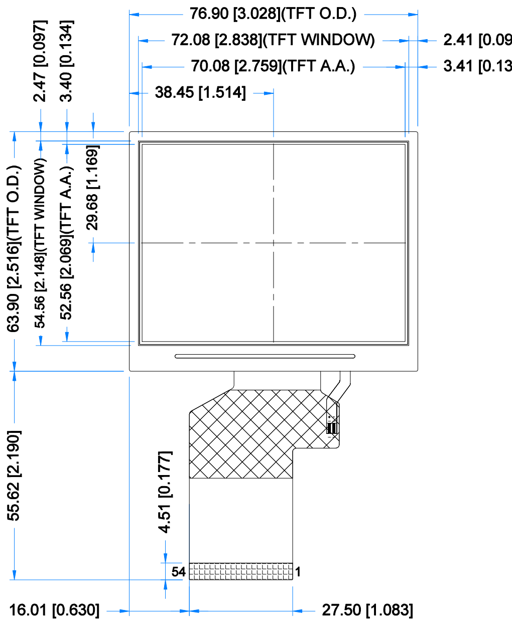
DETAIL A SCALE 2:1
