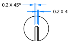
DETAIL B SCALE 4:1
