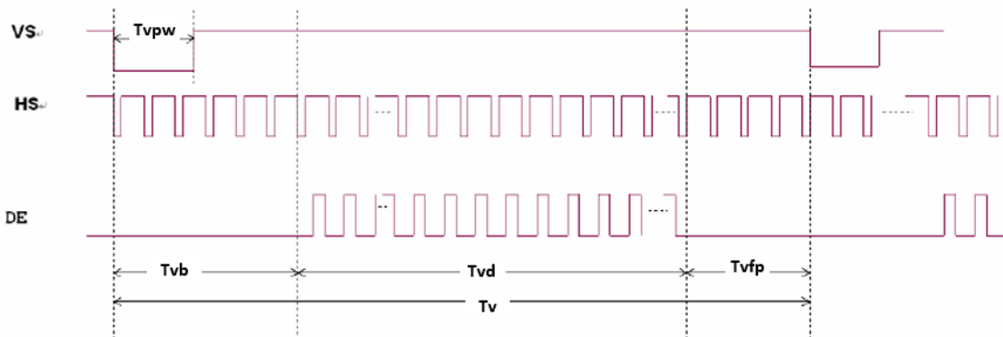
Figure 5. Vertical input timing diagram
