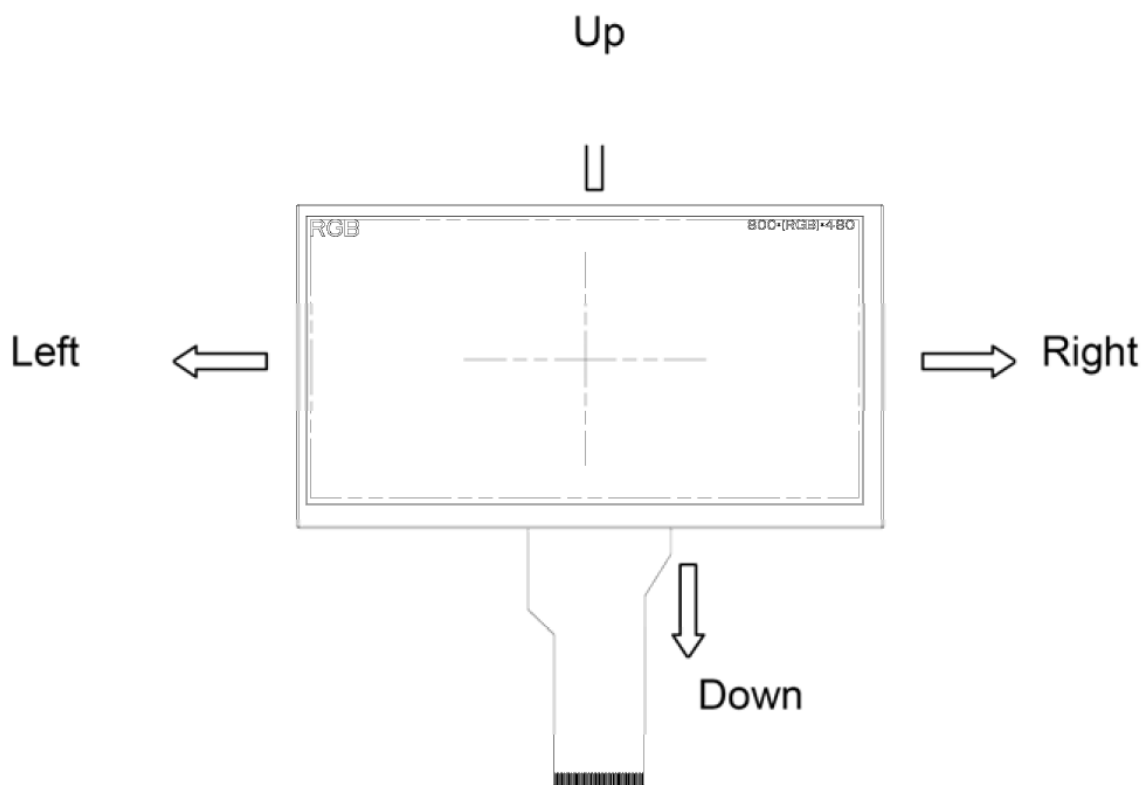
Figure 4. Definition of scanning direction
