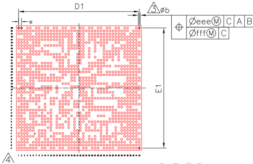
Fig.2-3 Package Bottom View
