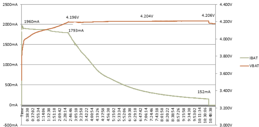
Fig. 4-17 Charge curve
