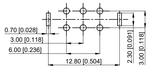
PCB LAYOUT BOTTOM VIEW PCB布局底视图
