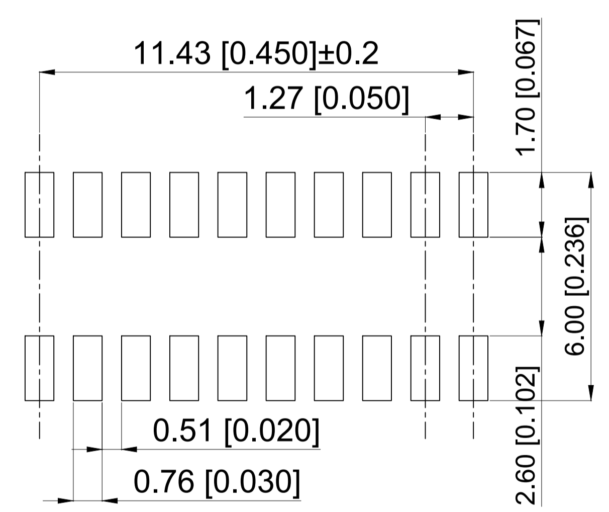
PCB LAYOUT
