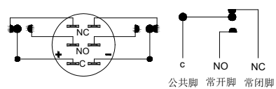
Electrical schematic diagram without lights 无灯电气原理图
